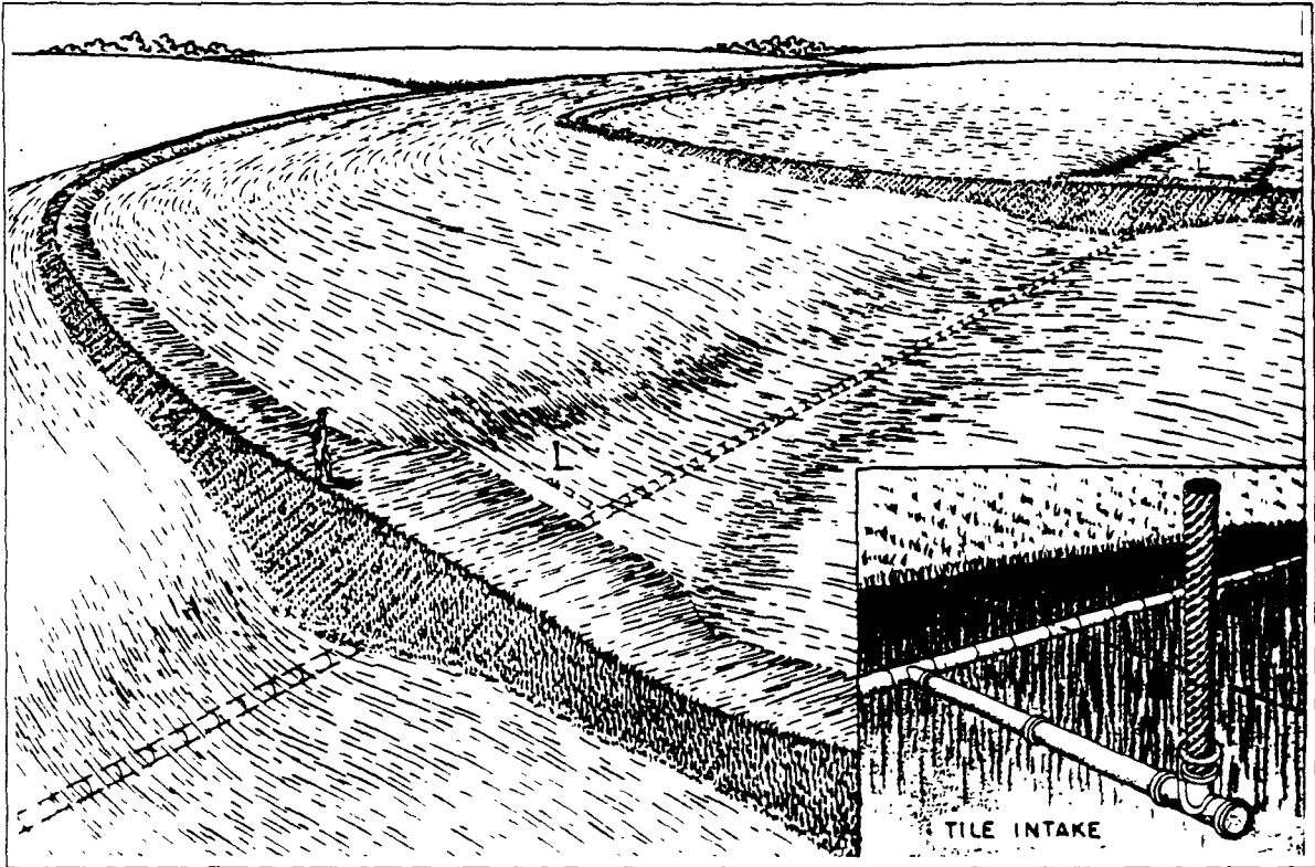
Figure 2-5. Gradient terraces with tile outlets (USDA-SCS, 1984).
