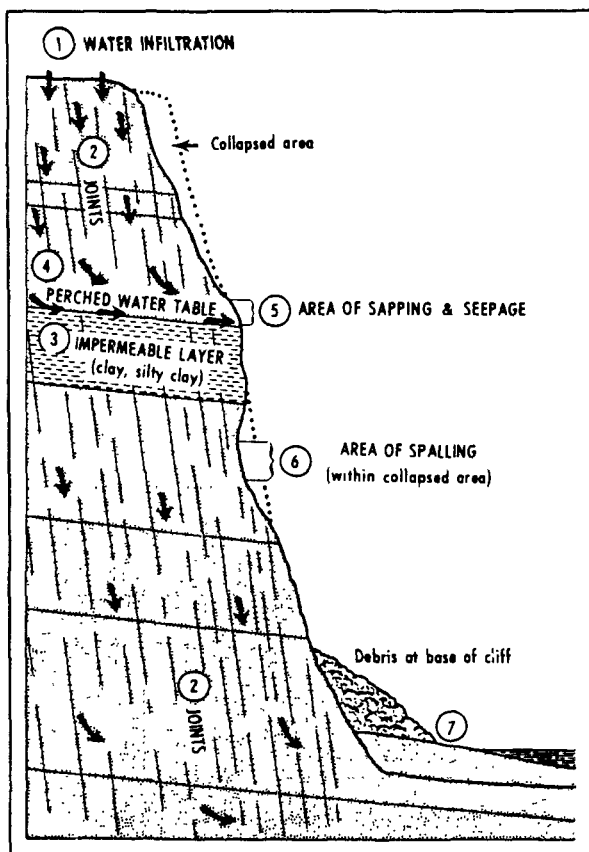
Figure 6-10. The physical processes of bluff erosion in a coastal bay. 1. Water enters the ground by infiltration of rainwater or snowmelt. 2. Nearly vertical cracks called joints aid the downward movement of water. 3. Water moves toward the cliff face upon reaching an impermeable layer of sediment formed by clay. 4. A perched water table forms above the clay layer; the overlying sandy sediments become saturated with water. 5. As water seeps out of the cliff and runs down the cliff face, it may erode the sandy sediments above the clay layer, in a process called sapping . 6. Spalling is another process by which the bluff face breaks off along a more or less planar surface roughly parallel to the face. Spalling is continuous throughout the year, but it intensifies during the winter months when freezing and thawing occur along the joints and seepage zones. 7. Wave action at the base removes fallen debris, allowing cliff failure to continue. (After Leatherman, 1986.)
