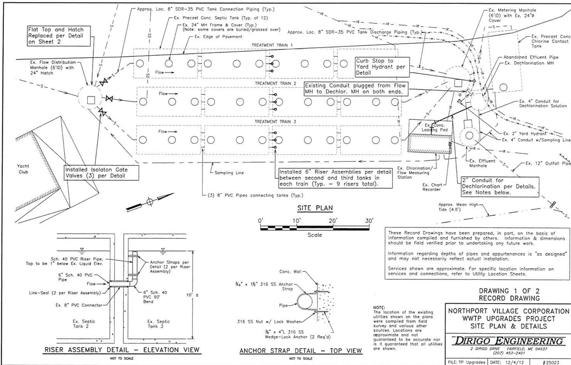
Treatment Schematic - Northport Village Corporation Wastewater Treatment Plant
