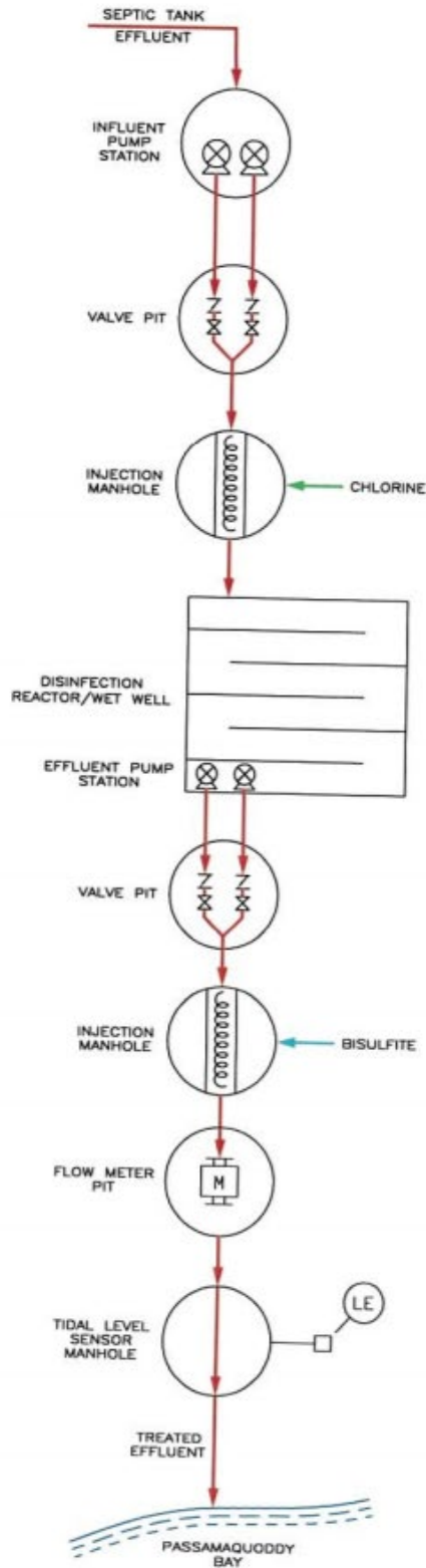
CITY OF EASTPORT, MAINE QUODDY VILLAGE TREATMENT PLANT SCHEMATIC DIAGRAM
