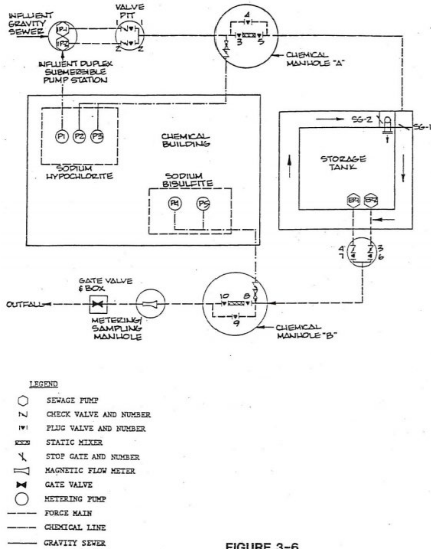
FIGURE 3-6 QUODDY DISINFECTION FACILITY PROCESS FLOW DIAGRAM
