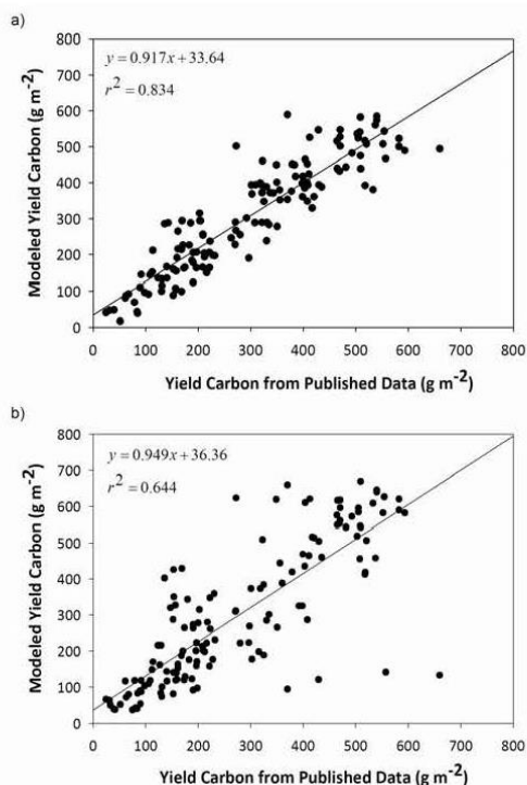
Figure A-9: Modeled versus measured net primary production (g C m -2 )
