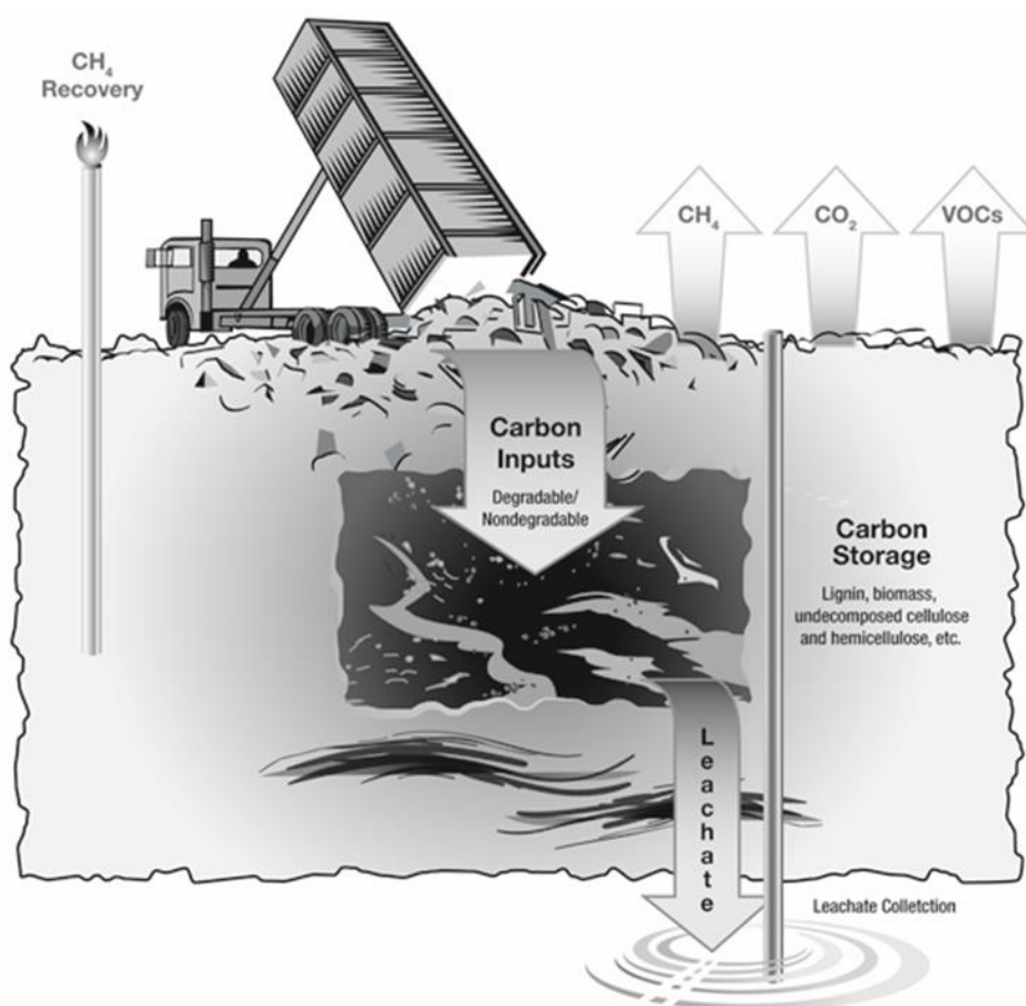
Exhibit 6-2: Landfill Carbon Mass Balance
