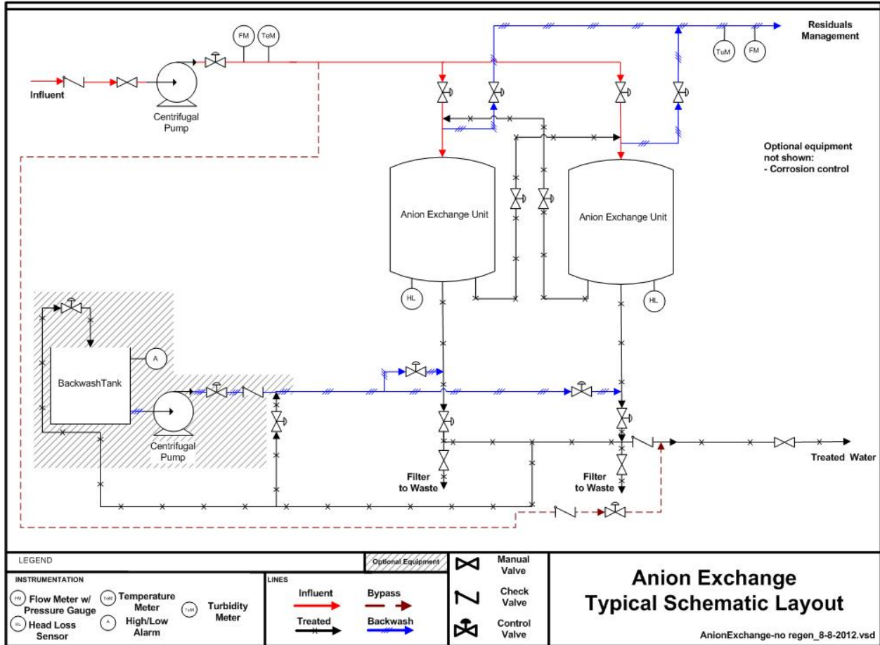
Exhibit 3-3. Typical Schematic Layout for Perchlorate Removal by Ion Exchange with Resin Disposal
