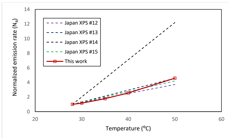
Figure_Apx G-10. Comparison of Normalized Emission Rates
