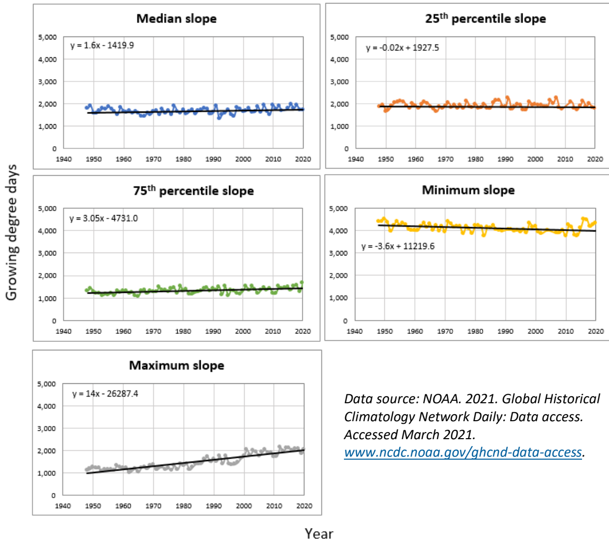
Figure TD-1. Annual Growing Degree Days for Five Sample Sites, 1948–2020
