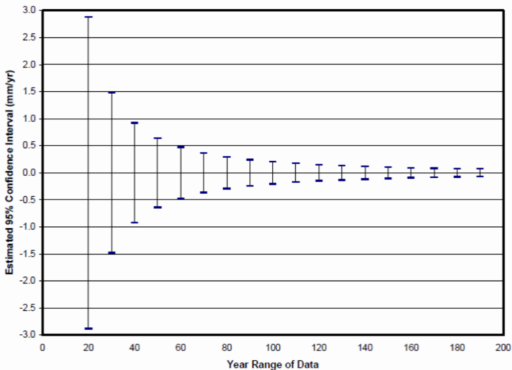
Figure TD-1. Comparison of 95% Confidence Intervals Versus Series Length for Linear Mean Sea Level Trends
