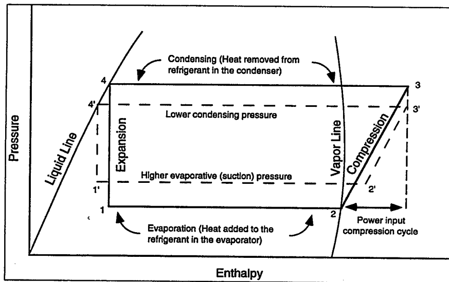
Exhibit 9.16: Pressure-Enthalpy Diagram
