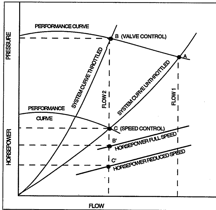
Exhibit 6.4: Fan Drive: Variable Speed vs. Valve Control
