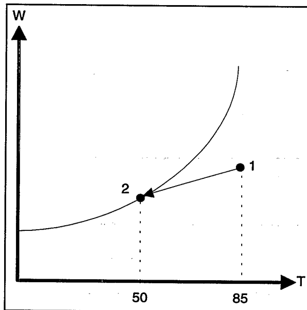
Exhibit B.10: Boiling Curve
