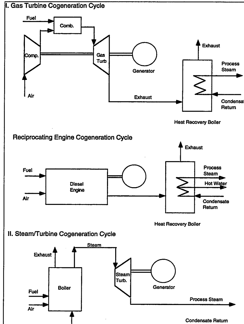
Exhibit 7.18: Cogeneration Cycles
