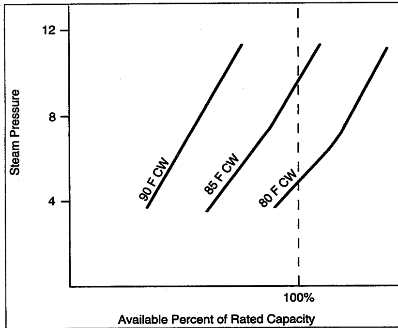
Exhibit 9.13: Capacity as Function of Temperature of Heat Source and Cooling Water
