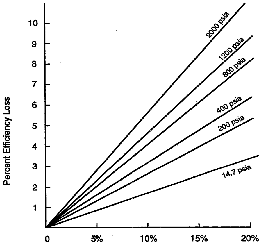
Exhibit 7.5: Efficiency Loss Due to Blowdown
