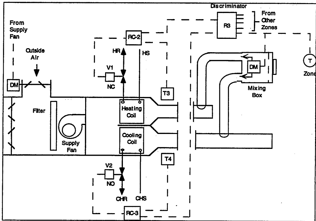
Exhibit 10.23: Dual Duct Air Handling System
