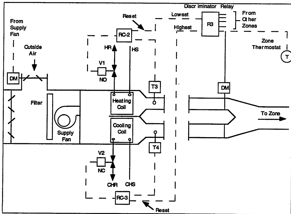
Exhibit 10.24: Multi-zone Air Handling Unit
