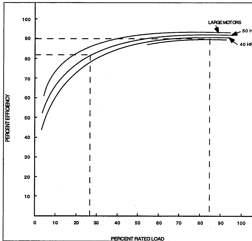
Exhibit 6.1: Motor Efficiency
