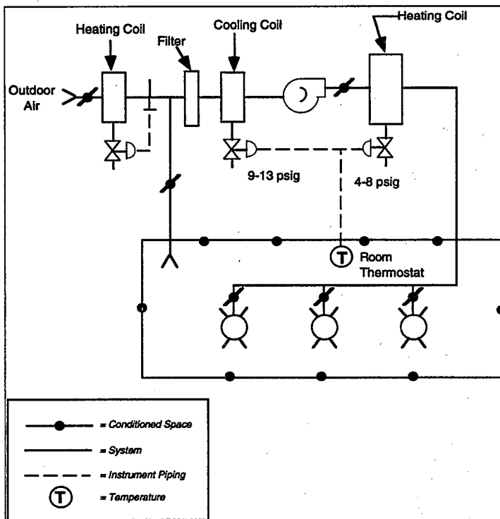
Exhibit 10.2: Modified Air Conditioning System Controls
