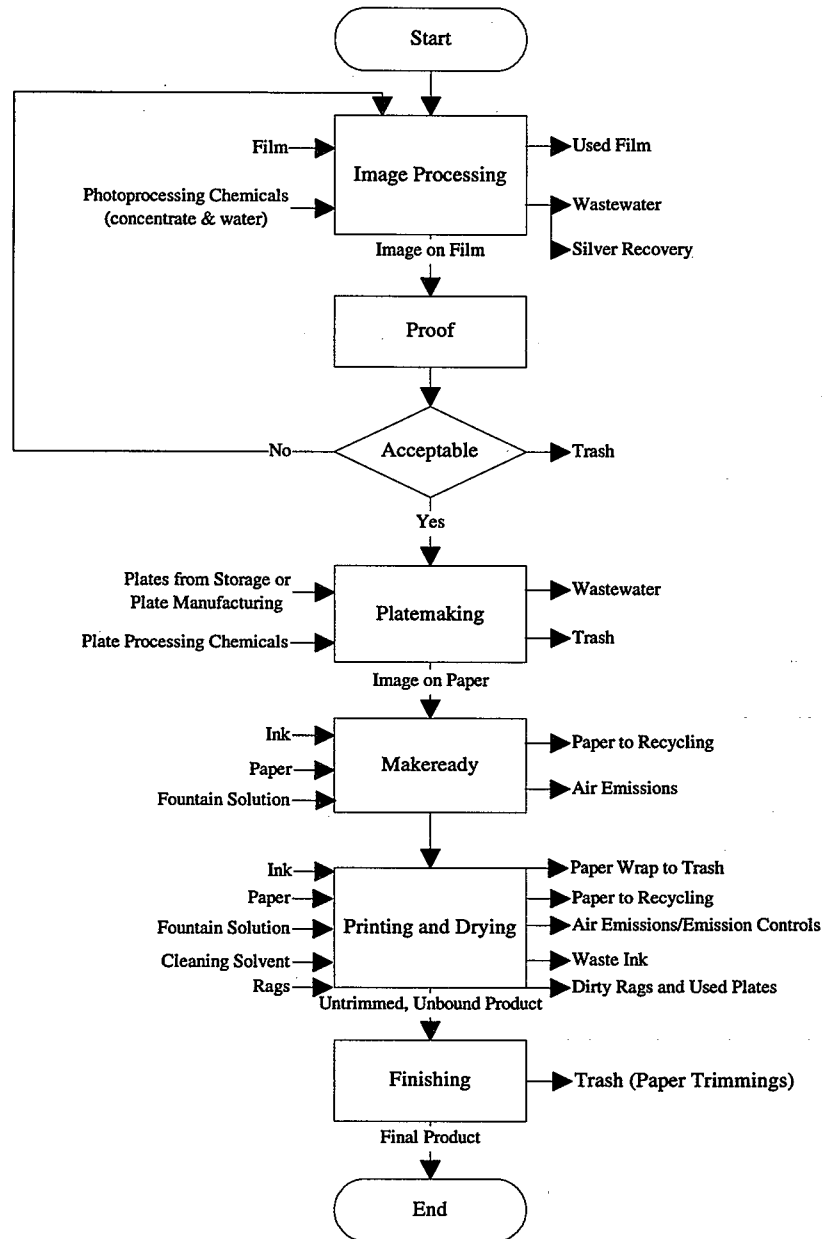
Exhibit 5.12: Process Flow Diagram for a Typical Commercial Printing Operation
