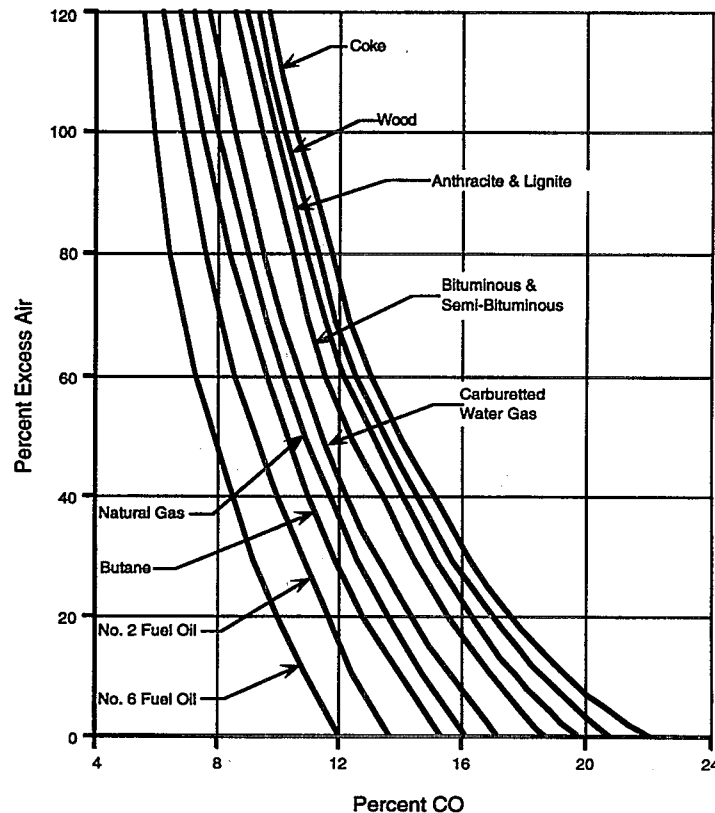
Exhibit 7.17: Percent Excess Air From CO 2 Reading
