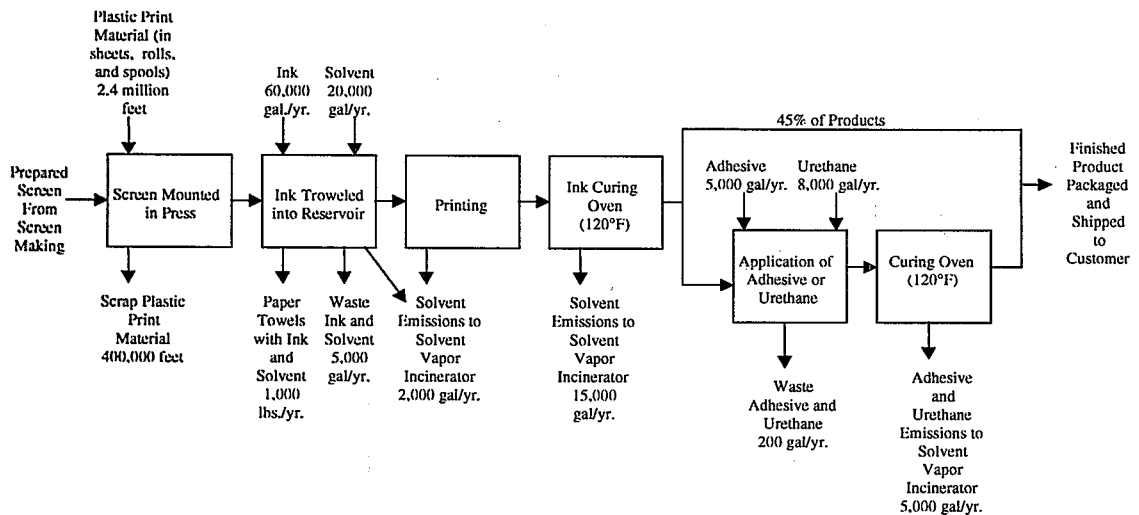
Exhibit 2.8: Example Flow Diagram for the Mars Screen Printing, Printing Operation
