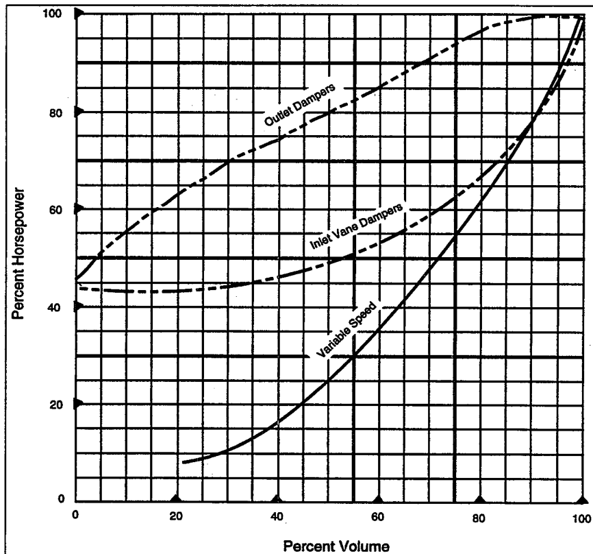
Exhibit 8.8: Effect of Volume Control on Fan Horsepower
