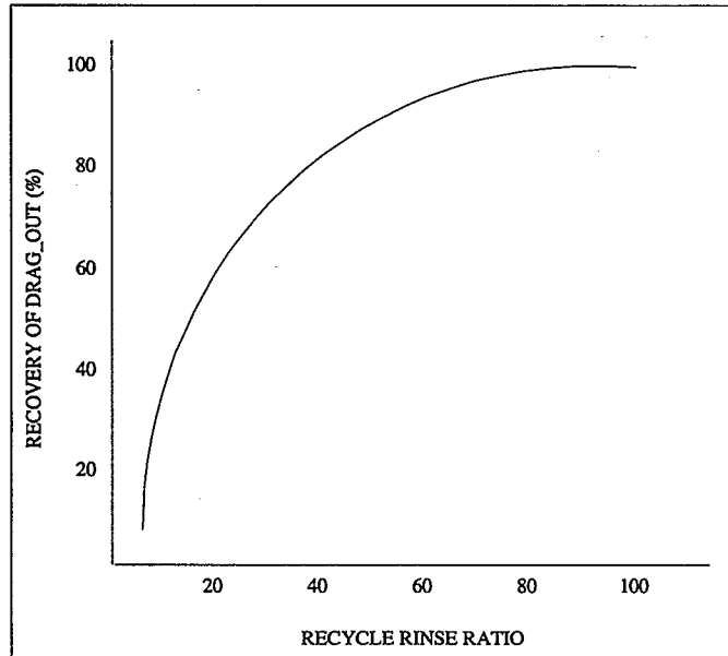
Exhibit F.7: Drag-Out Recovery as a Function of Recycle Rinse Ratio
