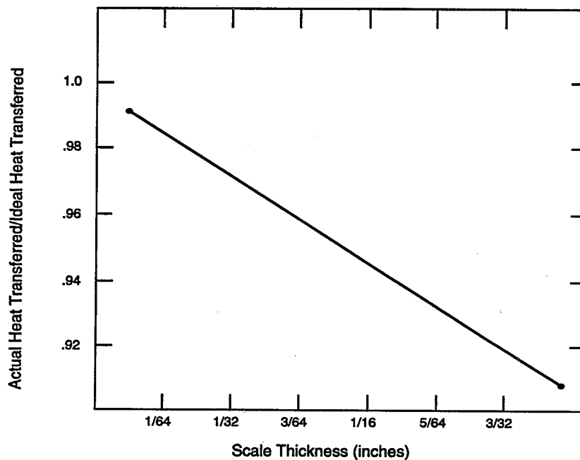
Exhibit 7.3: Effect of Scale Thickness in Boilers on Heat Transfer
