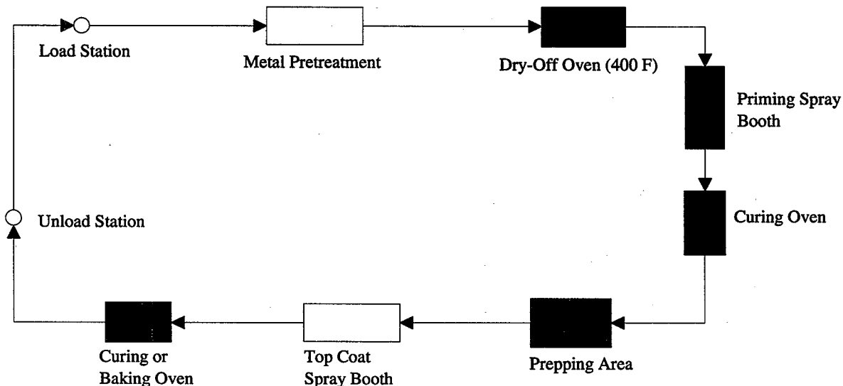
Exhibit 5.8: Schematic of a ConveyORIZED Paints and Coatings Operation
