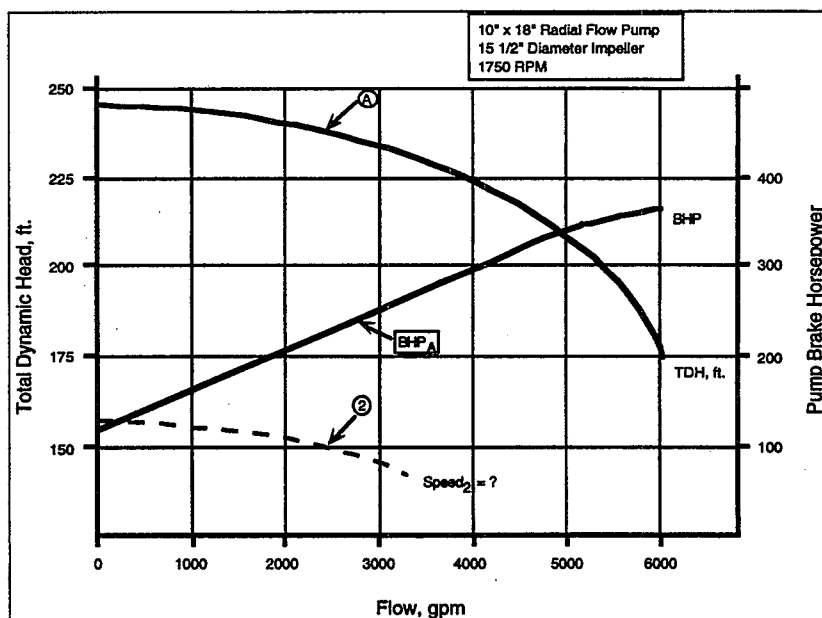
Exhibit 8.2: Centrifugal Pump Curve
