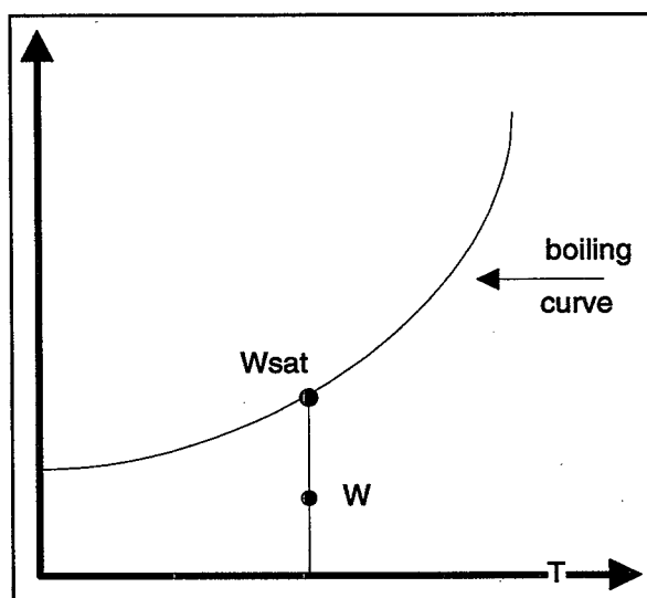
Exhibit B.3: Humidity vs. Temperature (Boiling Curve)
