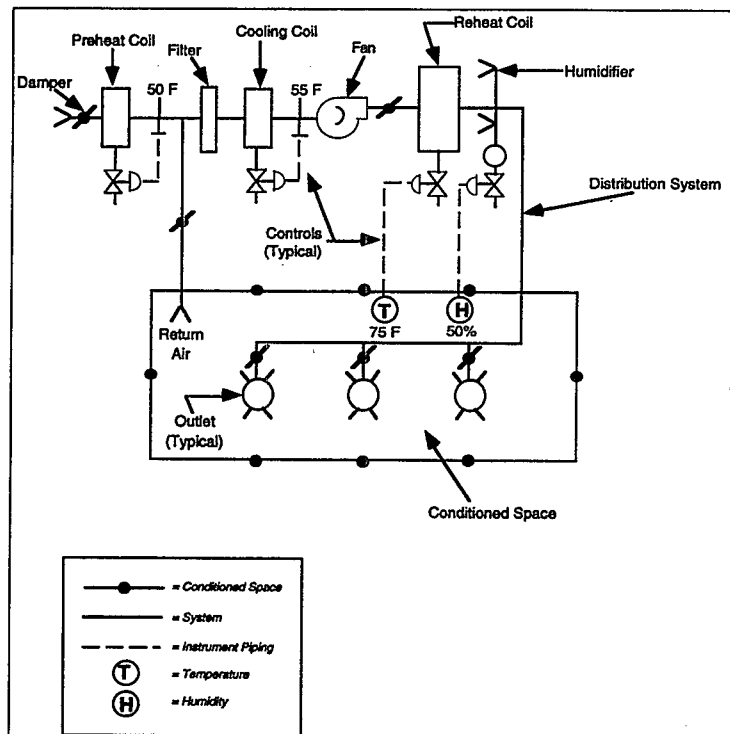
Exhibit 10.1: Air Conditioning Equipment
