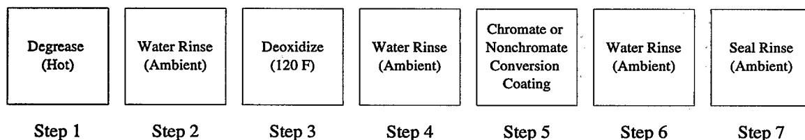
Exhibit 5.5: Typical Conversion Coating Process for Aluminum
