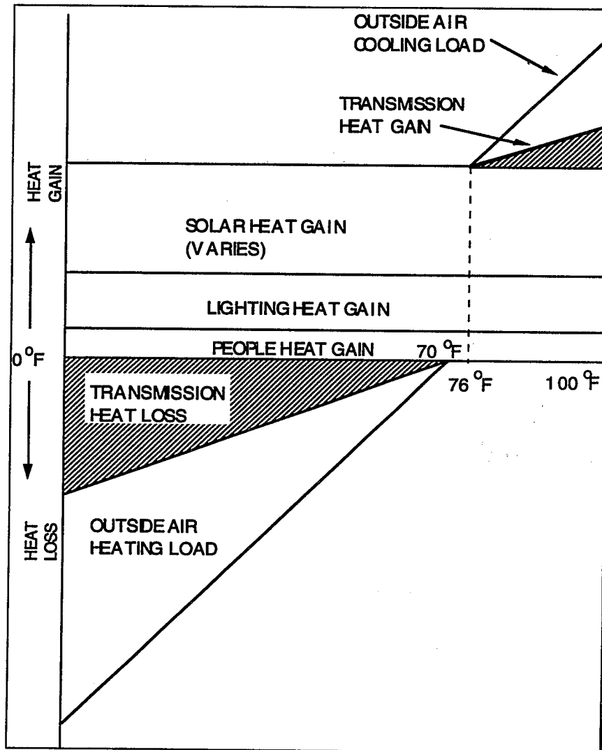
Exhibit 10.11: Heating and Cooling Loads
