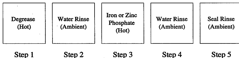
Exhibit 5.4: Five-stage Iron or Zinc Phosphating Process
