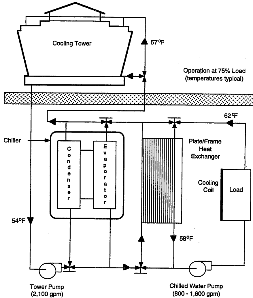
Exhibit 9.6: Free Cooling (Water Side Economizer) Define Operating Conditions
