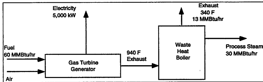
Exhibit 7.19: Gas-Turbine Cycle
