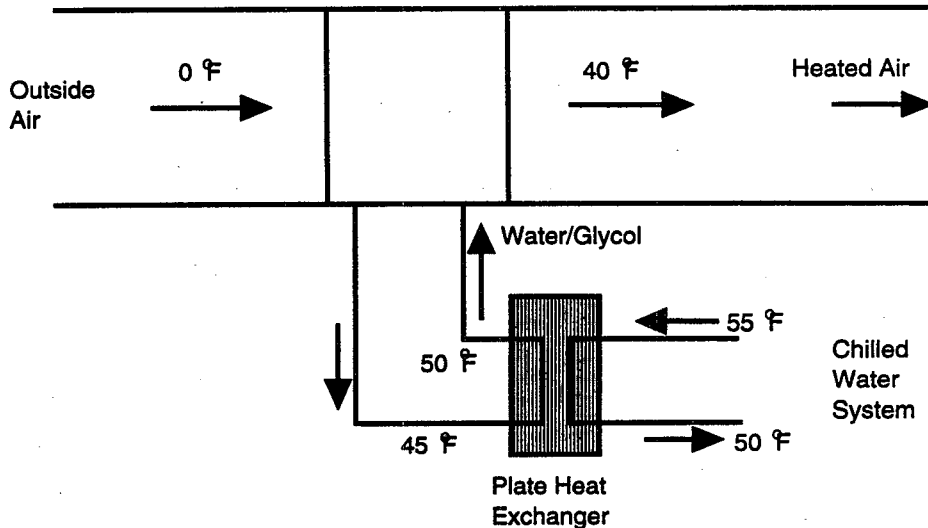
Exhibit 9.4: Free Cooling/Air Preheat
