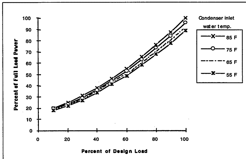
Exhibit 9.17: Partial Load Requirement for Centrifugal Refrigeration Compressors
