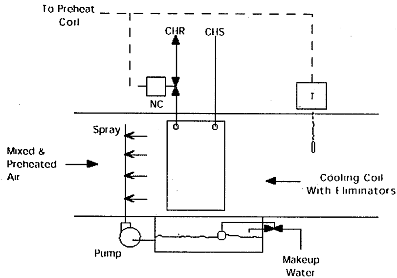
Exhibit 10.19: Sprayed Coil Dehumidifier
