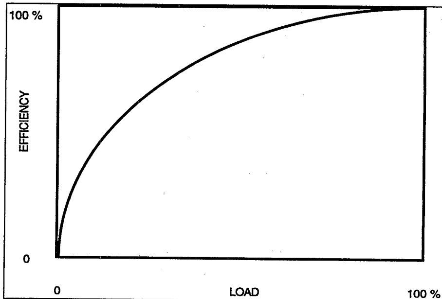
Exhibit 10.10: Control Valve Characteristics
