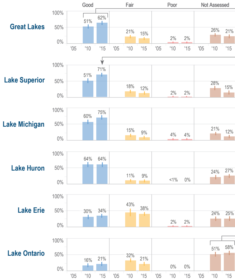
Figure 4.3.2. Change in Great Lakes Sediment Quality
