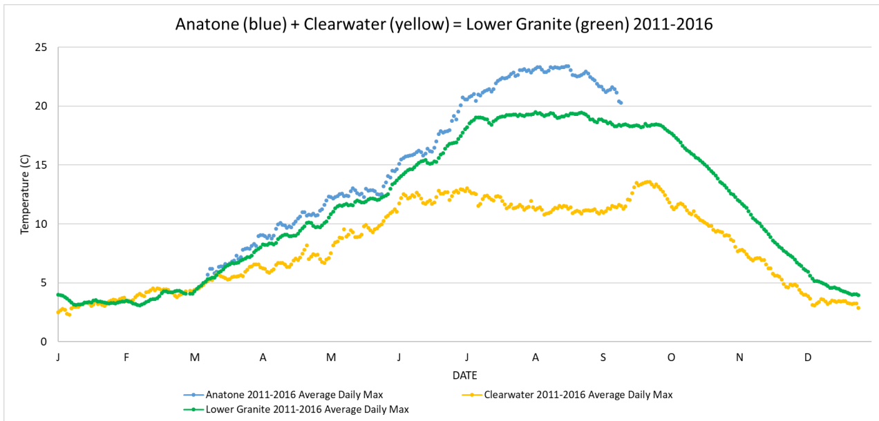
Figure 29. Anatone, WA average maximum river temperature (blue) and Clearwater River average maximum river temperature (yellow) blend at the Clearwater River confluence, leading to the average maximum river temperature at Lower Granite Dam 2011-2016.
