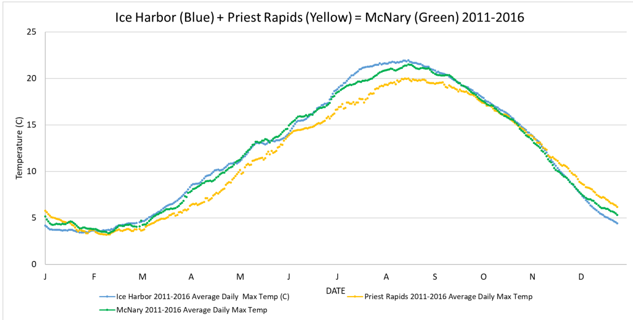
Figure 28. Ice Harbor Dam average maximum river temperature (blue) and Priest Rapids Dam average maximum river temperature (yellow) blend at the Snake River confluence, leading to the average maximum river temperature at McNary Dam (green) 2011-2016. Note that there is also warming between Priest Rapids Dam and the Snake River confluence not represented in this plot due to data limitations at the Pasco monitoring site.
