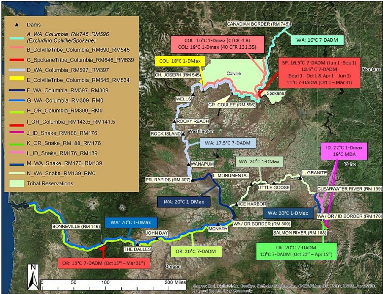
Figure 2. Numeric temperature water quality criteria on the Columbia and Lower Snake Rivers. Data Source: EPA Temperature WQC Compilation 2018.
