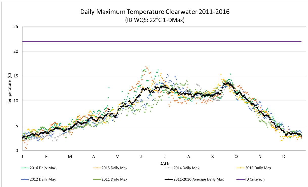
Figure 21. Daily maximum river temperature at the Clearwater station for the years 2011-2016, plotted against the applicable Idaho numeric WQC of 22°C DM.
