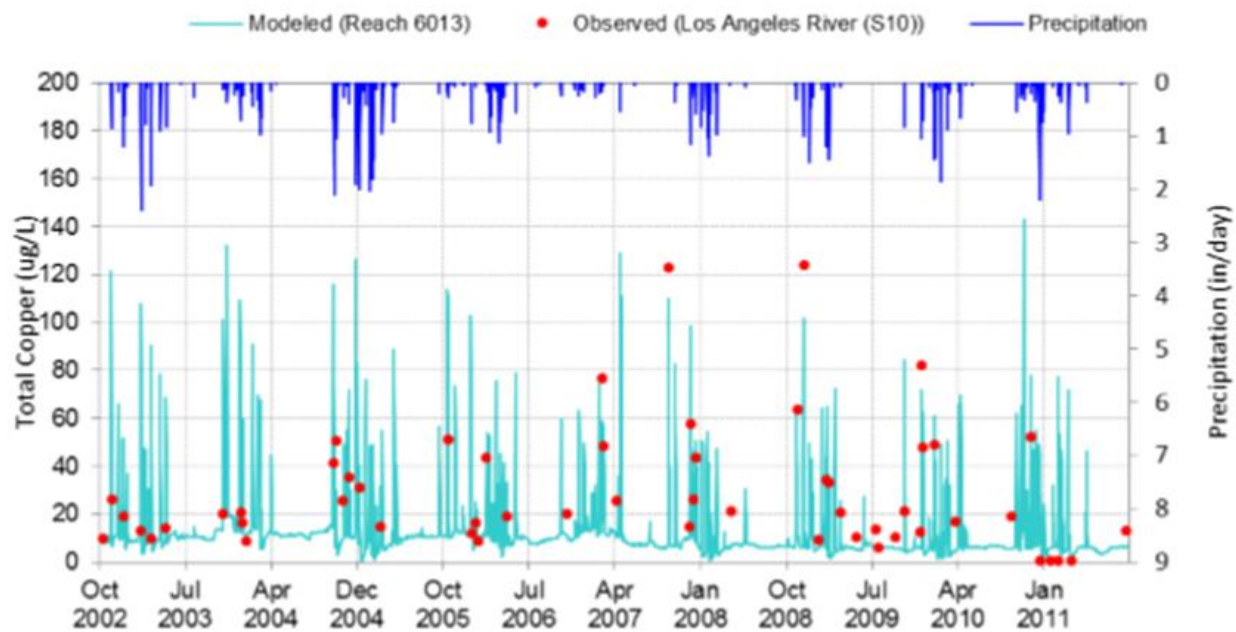
Figure A-2. Model Water Quality (total copper) Calibration for Los Angeles River (ULAR WMG 2016).
