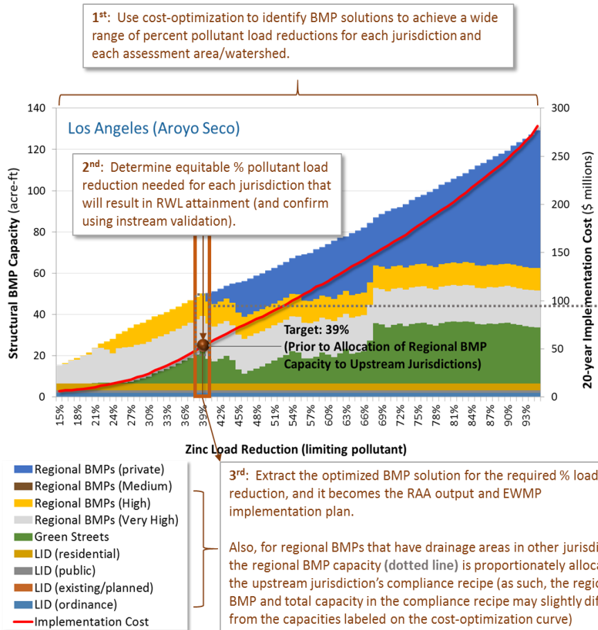
Figure A-4. Illustration of how the EWMP Implementation Strategy is Extracted from a Cost Optimization Curve (ULAR WMG 2016). 2
