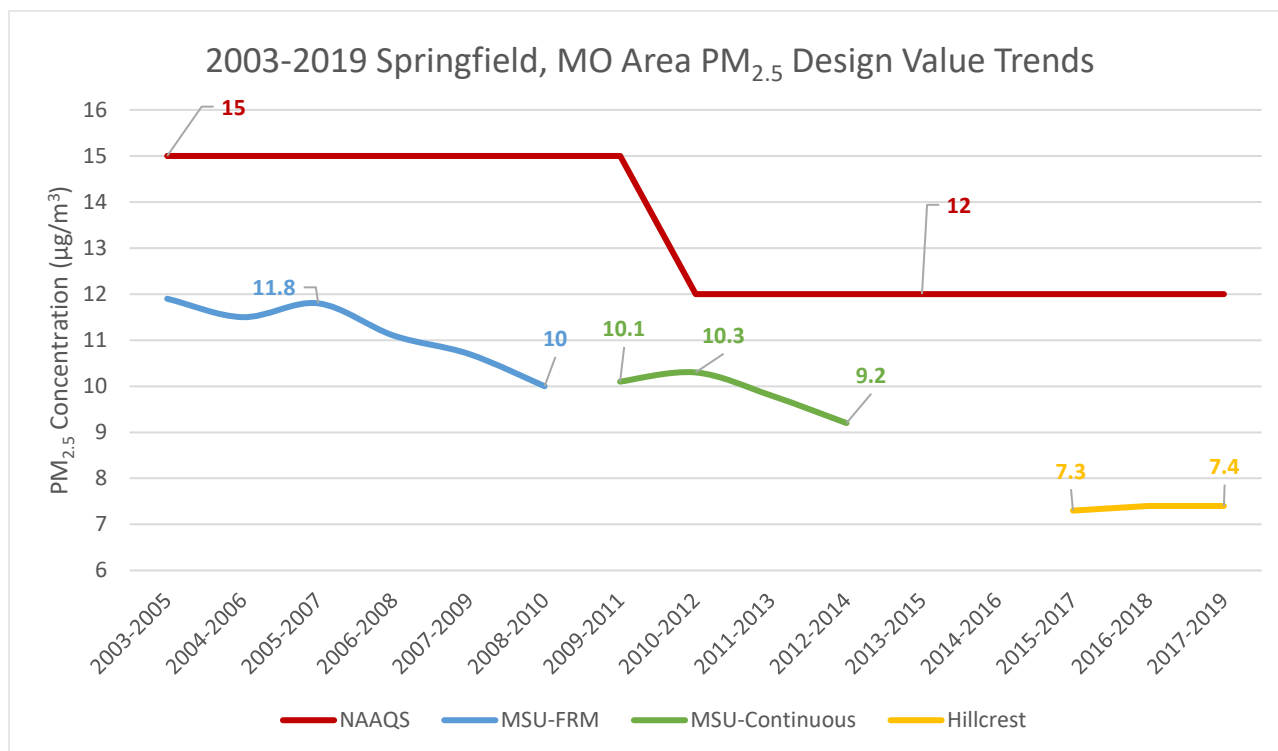
Figure 8. Fine Particulate Matter (PM 2.5 ) Design Value Trends in the Springfield, MO Area from 2003 to 2019. One line represents the evolving EPA NAAQS standards, which can be used for comparison with the actual measured values from Hillcrest High School and MSU. Gaps in the data exist due to certification of data when monitors are moved. PM 2.5 concentration is measured in micrograms per cubic meter ( \mu\text{g}/\text{m}^3 ).
