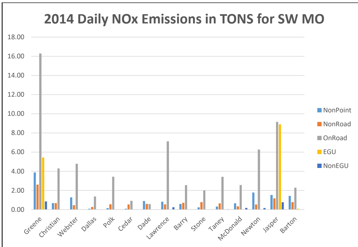
Figure 2. Daily NO x Emissions in Southwest Missouri in 2014. This graph depicts the amounts of NO x emissions produced daily by each county in 2014. These emissions are divided into each of the five man-made emissions categories outlined previously. Emissions are measured in tons per day.
