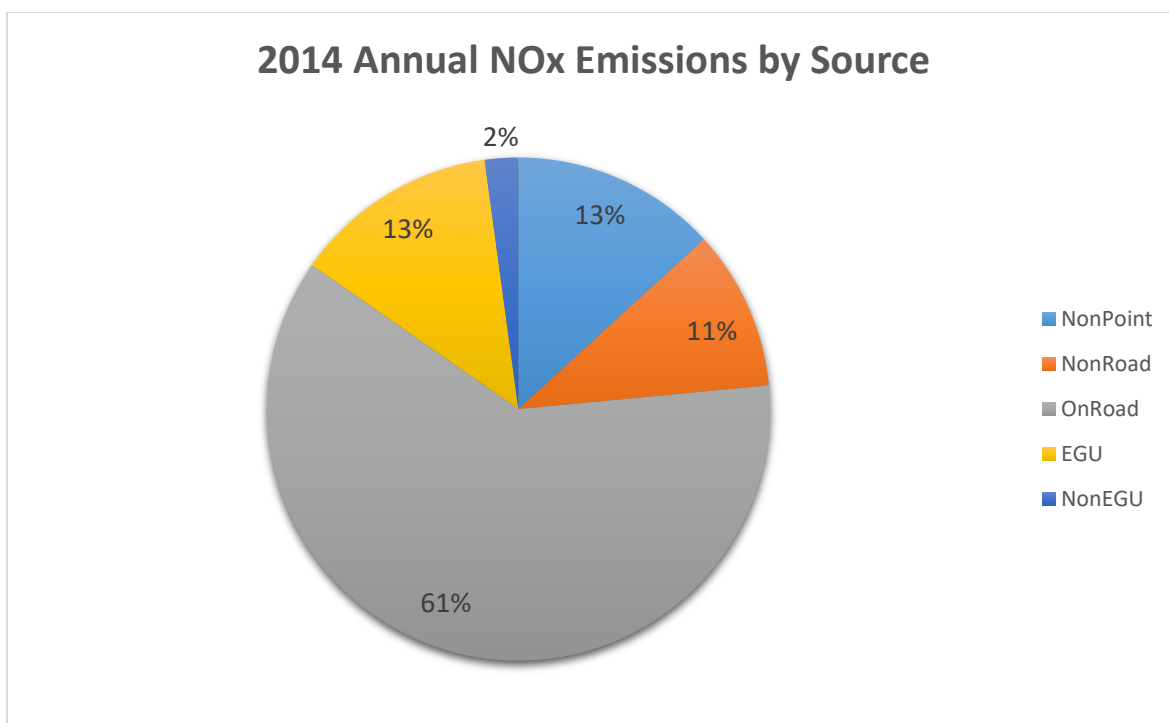
Figure 4. NO x Emissions by Source in 2014. This circle totals all emissions in all counties, depicting each man-made source category as a percentage of the whole.
