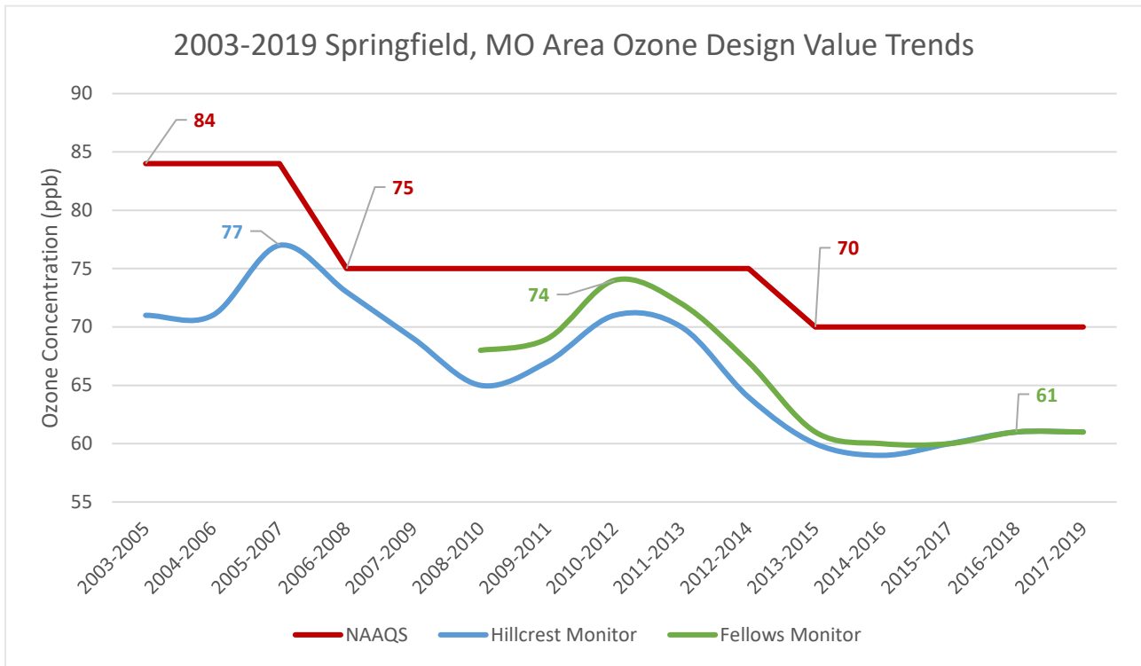
Figure 6. Ozone Design Value Trends in the Springfield, MO Area from 2003 to 2019. One line represents the evolving EPA NAAQ standards, which can be used for comparison with the actual measured values from Hillcrest High School and Fellows Lake. Ozone concentration is measured in parts per billion (ppb).
