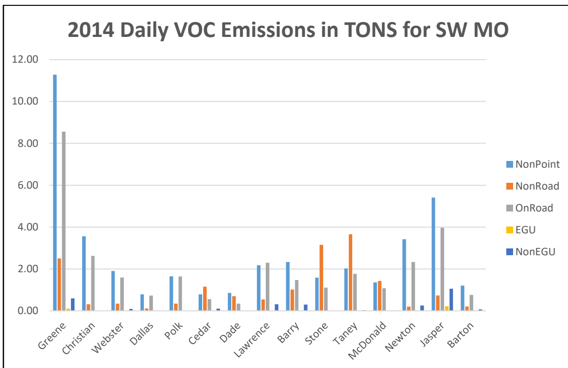
Figure 3. Daily VOC Emissions in Southwest Missouri in 2014. This graph depicts the amounts of VOC emissions produced daily by each county in 2014. These emissions are divided into each of the five man-made emissions categories outlined previously. Emissions are measured in tons per day.
