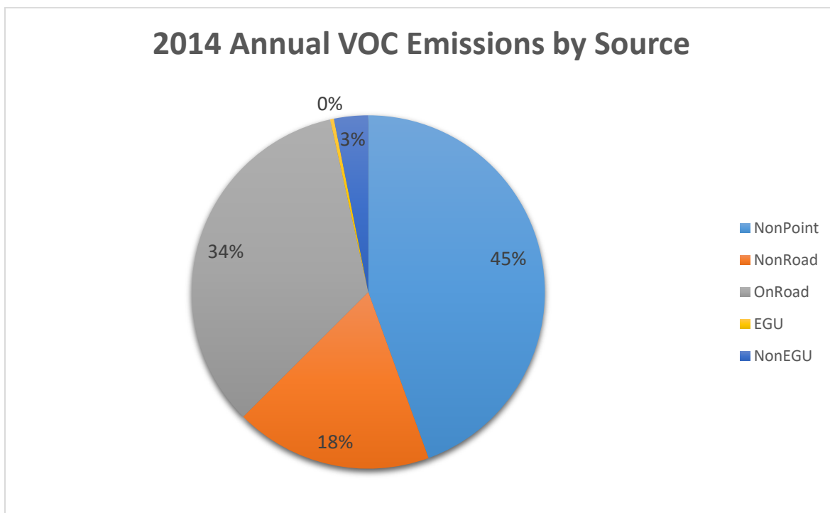
Figure 5. VOC Emissions by Source in 2014. This circle totals all emissions in all counties, depicting each man-made source category as a percentage of the whole.
