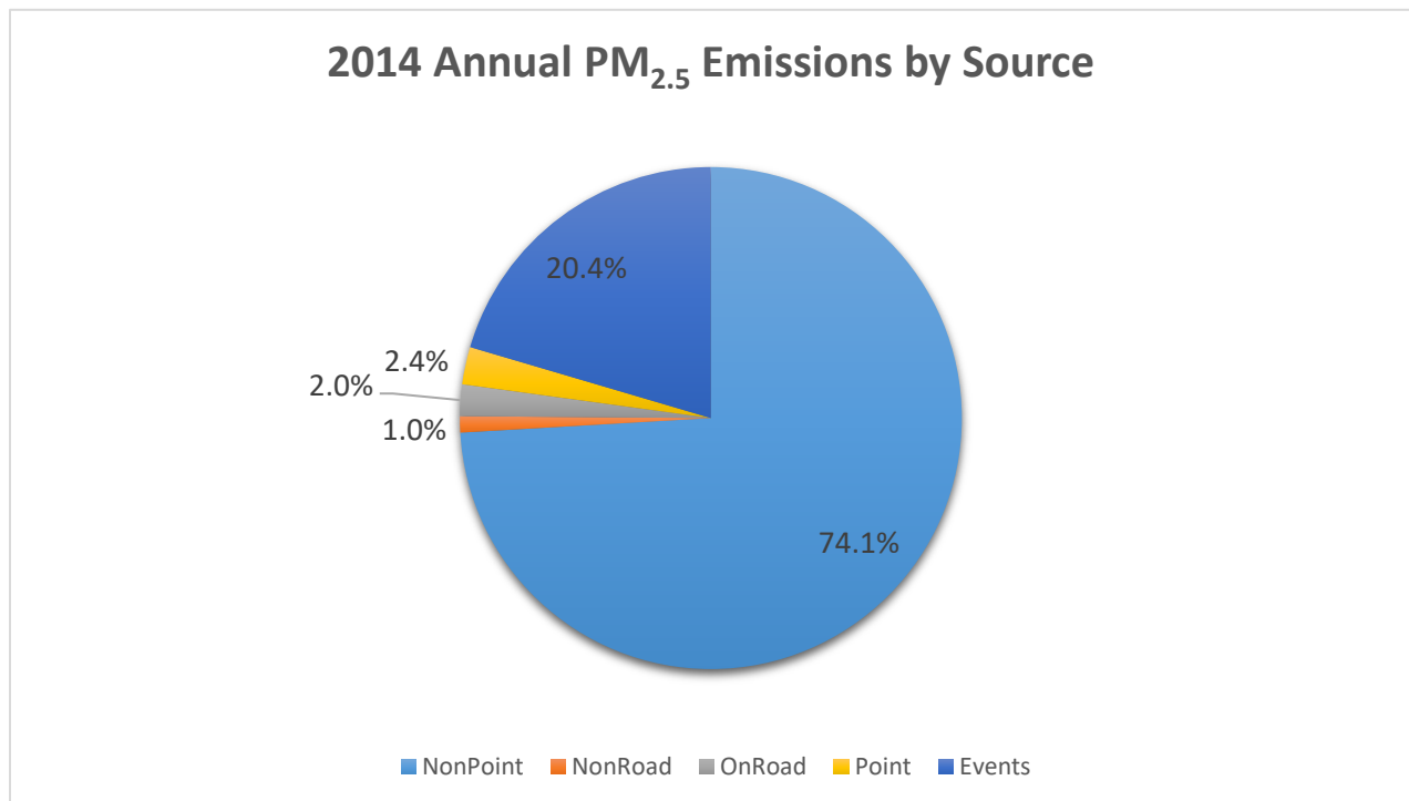
Figure 7. Fine Particulate Emissions by Source in 2014. This circle totals all emissions in all counties, depicting each man-made source category as a percentage of the whole.
