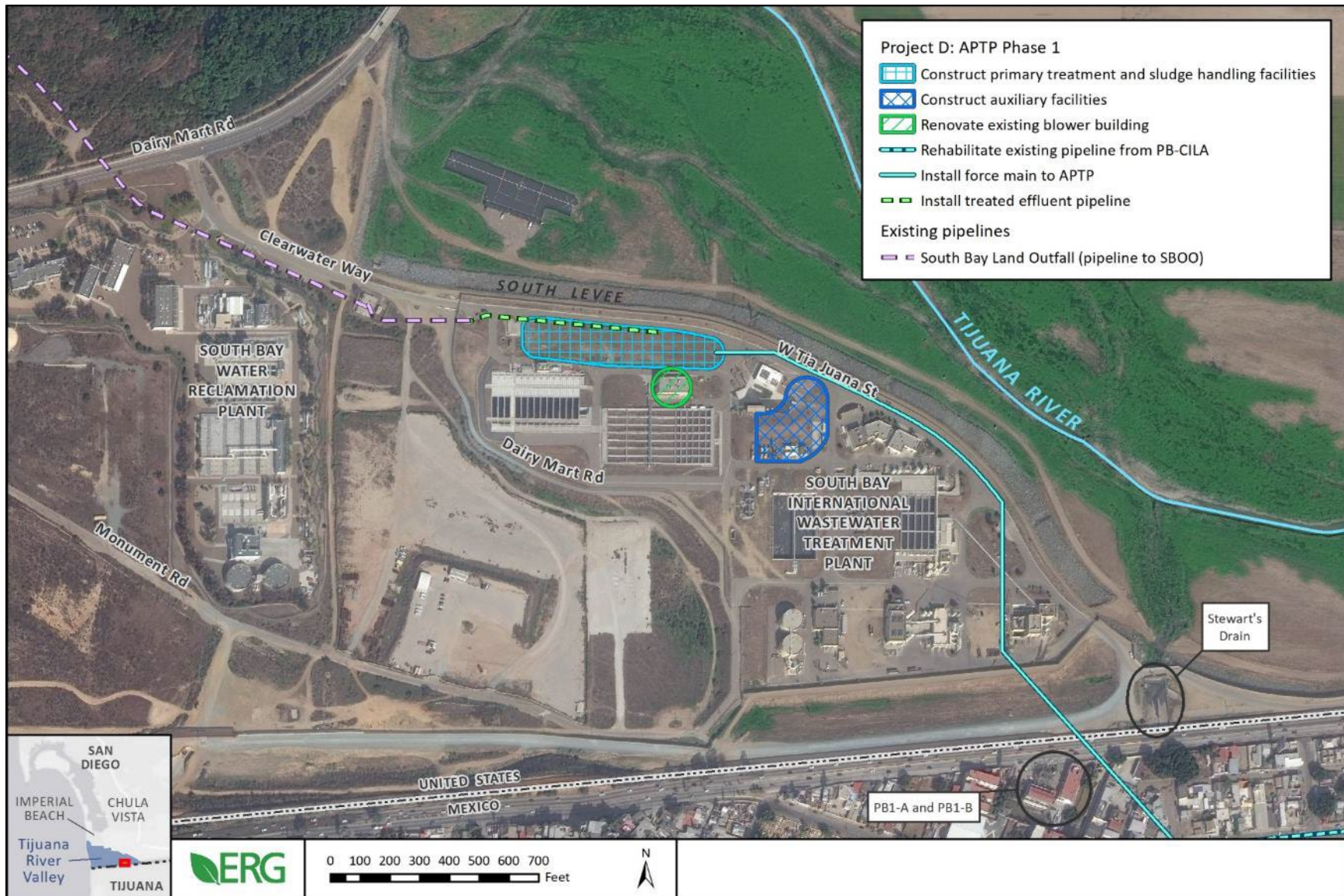
Figure 1-7. Project D (AFTP Phase 1) – Locations of Project Components (1 of 2)
