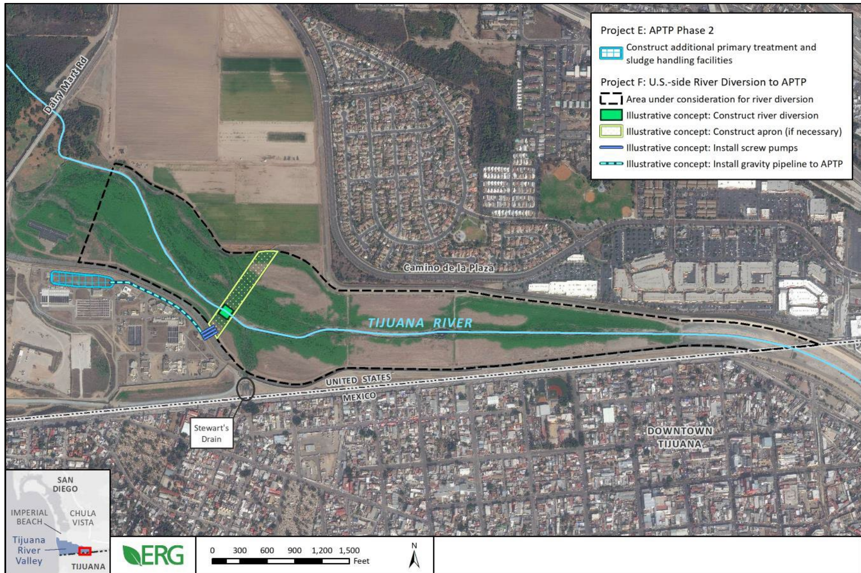
Figure 2-1. Projects E (AFTP Phase 2) and F (U.S.-side River Diversion to AFTP) – Conceptual Locations of Project Components
