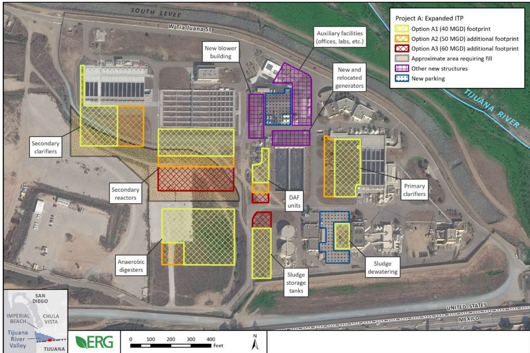
Figure 1-2. Project A (Expanded ITP) – Conceptual Site Plan of Proposed Facilities
