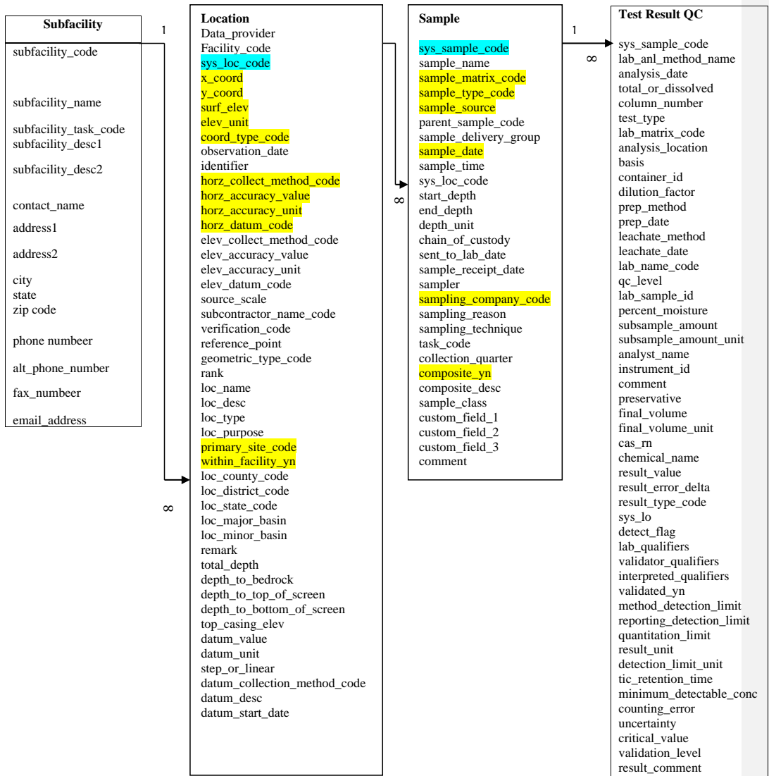
Figure 2-1 Relationships between Lab file data structures.
