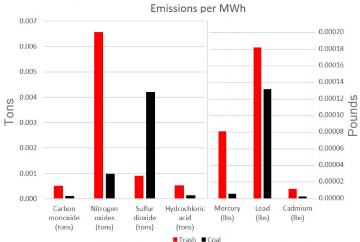
Figure 1. New York Department of Environmental Conservation Comparison of Trash Incinerator to Coal Power Plan emissions rates
