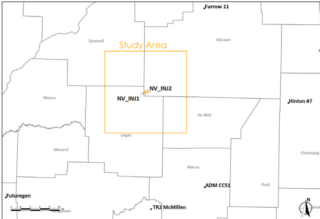
Figure 26: Wells used for petrophysical analysis of the Vervain injection and confining zones. ADM CCS1 Mt. Simon Sandstone porosity and permeability values are reported in Table 4, and geomechanical properties are reported in Table 5.
