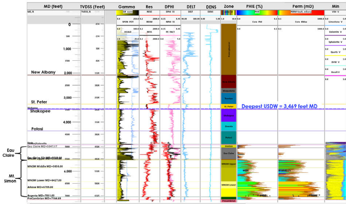
Figure 41: ADM CCS1 (IL121152341500) well logs that show that the lowermost USDW occurs in the St. Peter Sandstone at 3,469 feet measured depth. MD=measured depth in feet, TVDSS=subsea true vertical depth, Gamma=gamma ray, RES=deep resistivity, DPHI=density porosity, DELT=sonic, DENS=density, Zone=stratigraphic zone, PHIE=effective porosity (%), Perm=permeability (mD), and Min=mineralogy.
