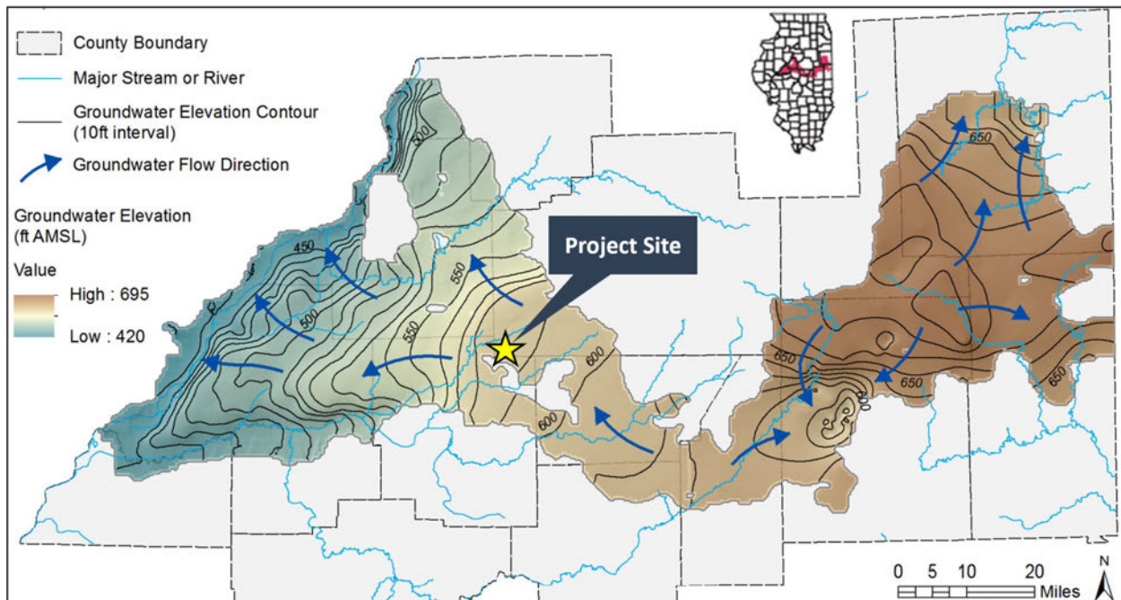
Figure 39: Map of the Mahomet aquifer with groundwater elevation in feet above mean sea level (AMSL) contours and flow direction. Modified from Roadcap et al., (2011).
