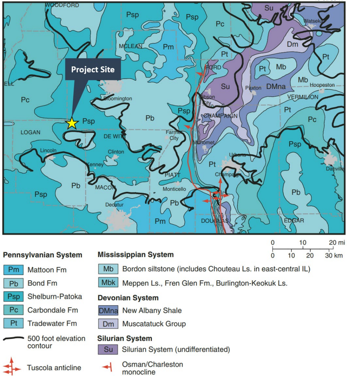
Figure 38: Bedrock geology underlying the Mahomet Aquifer. Modified from Kempton et al., 1991 & Kolata et al., 2005.
