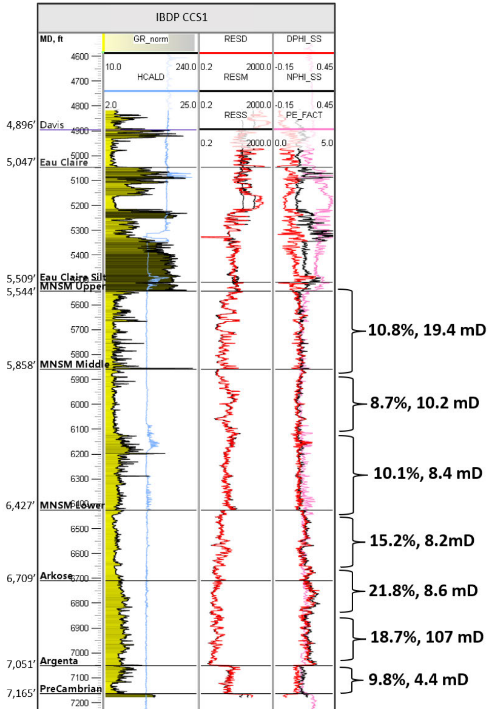
Figure 27: ADM CCS1 geophysical logs with measured depth (MD), formation tops, average effective porosity (%), and intrinsic permeability (mD) values. GR_norm=normalized gamma ray log; HCALD=caliper; RESD, RESM, and RESS = deep, medium, and shallow resistivity; DPHI_SS=density derived sandstone porosity; NPHI_SS=neutron-derived sandstone porosity; PE_FACT= photoelectric factor.
