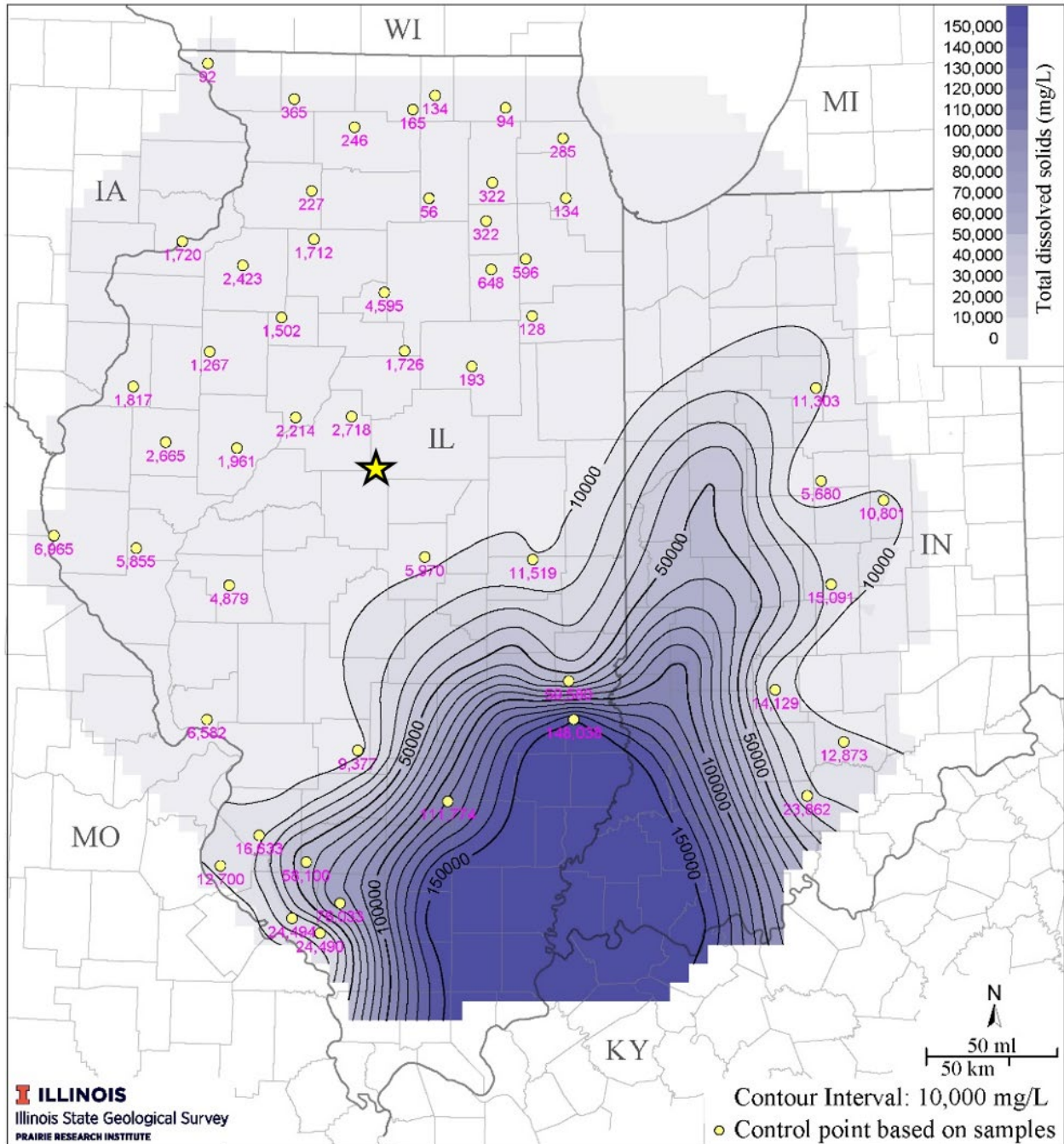
Figure 42: Map of the St. Peter Sandstone total dissolved solids. The project site is represented with a yellow star and sample locations are shown by yellow circles. This is unpublished work by the Illinois State Geological Survey (Whittaker, 2021).
