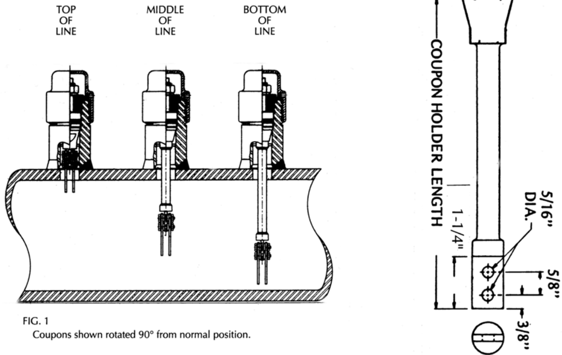
Figure 7: Corrosion coupon illustration in pipeline (Cosasco, 2022)
