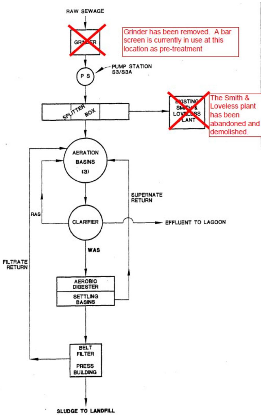
GENERAL FLOW DIAGRAM
