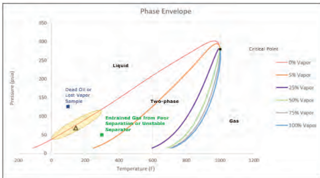
Figure 5-1. Phase Envelope
