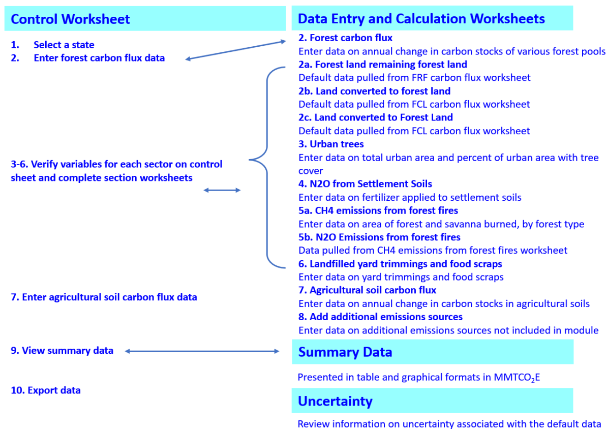
Figure 3: Flow of Information in the LULUCF Module*
