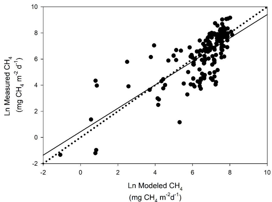
1 Figure A-17: Comparisons of Results from DayCent Model and Measurements of Soil 2 Methane Emissions from Rice Cultivation
