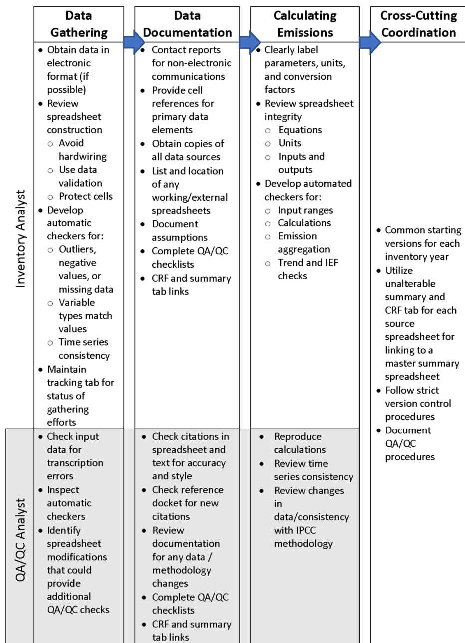
Figure A-22: U.S. QA/QC Plan Summary
