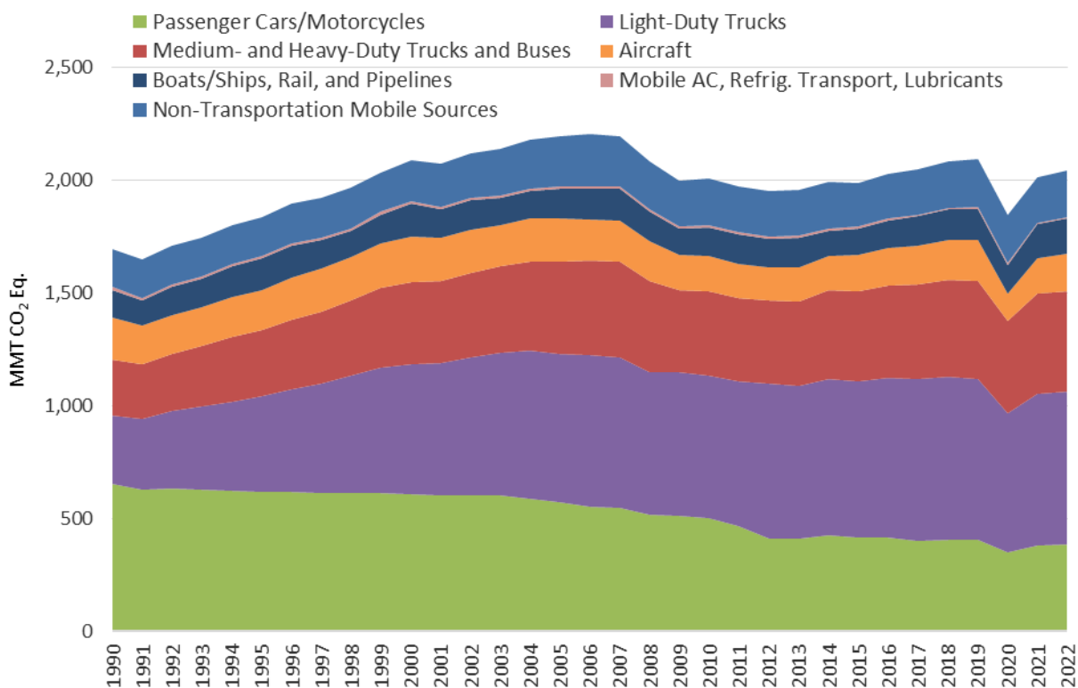
1 Figure A-4: Domestic Greenhouse Gas Emissions by Mode and Vehicle Type, 1990 to 2022
