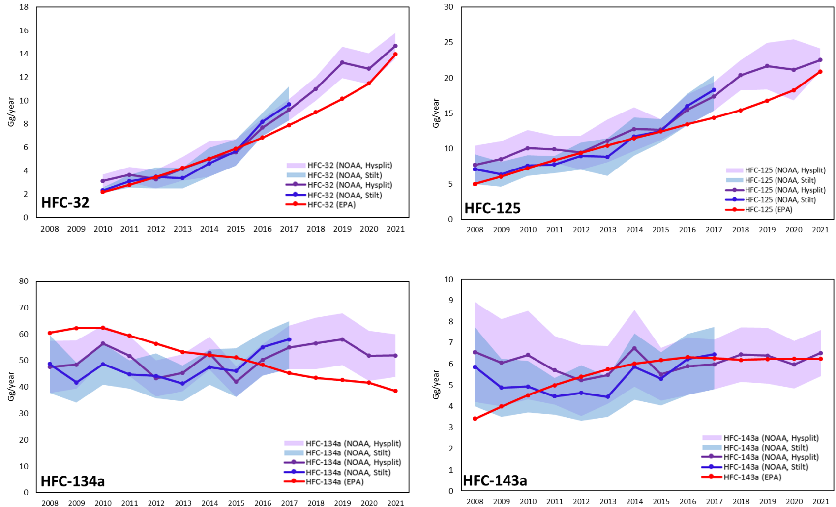
1 Figure A-8: U.S. Emissions of HFC-32, HFC-125U, HFC-134a, and HFC-143a
