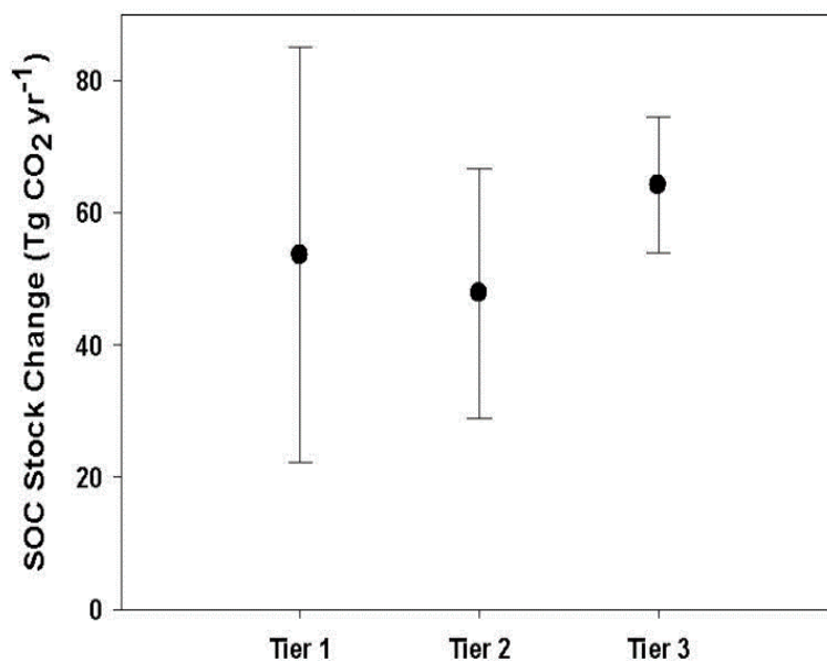
Figure A-15: Comparison of Estimated Soil Organic Carbon Stock Changes and Uncertainties using Tier 1 (IPCC 2006), Tier 2 (Ogle et al. 2003, 2006) and Tier 3 Methods
