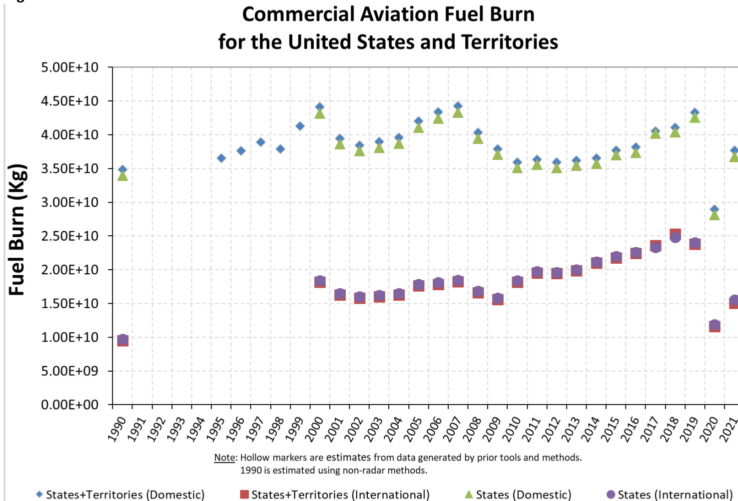
1 Figure A-5: Commercial Aviation Fuel Burn for the United States and Territories
