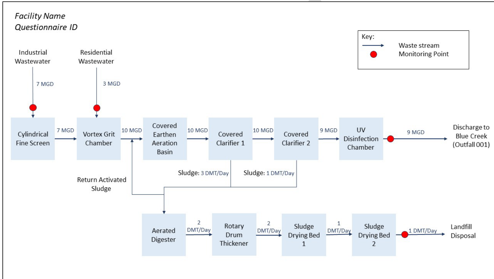
Figure 11. Example Wastewater Treatment Diagram
