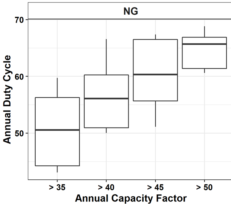
Figure 4: Boxplot of minimum annual duty cycle versus capacity factor group. Outer lines mark the 10 th and 90 th percentiles. Outer edges of the boxes mark the 25 th and 75 th percentiles. Center lines mark the 50 th percentiles.
