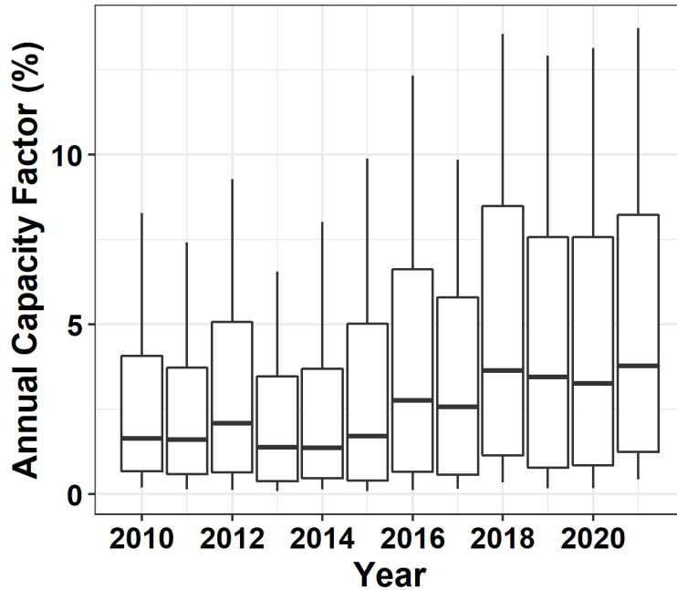
Figure 4: Capacity factor of simple cycle turbines by year. Center lines show median values for annual capacity factor from simple cycle units. The upper and lower bounds of each box mark the 25 th and 75 th percentile of the distribution of annual capacity factors for each year. The upper and lower bounds of each set of vertical lines mark the 10 th and 90 th percentile of the distribution of annual capacity factors for each year.
