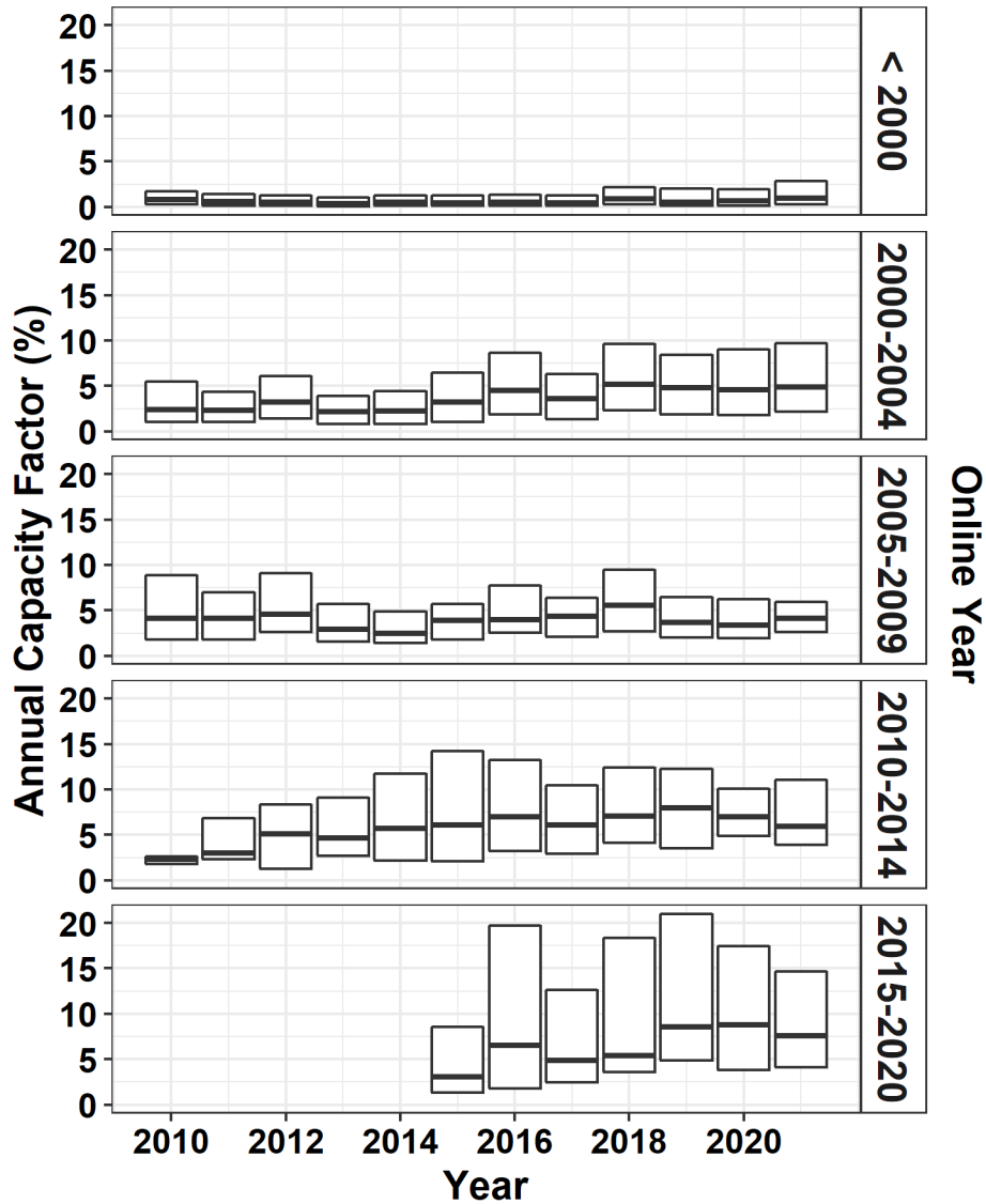
Figure 6: Annual capacity factor (based on gross generation) of simple cycle turbines by year, grouped by year of initial commercial operation. Center lines show median values for annual capacity factor from simple cycle units. The upper and lower bounds of each box mark the 25 th and 75 th percentile of the distribution of annual capacity factors for each year.
