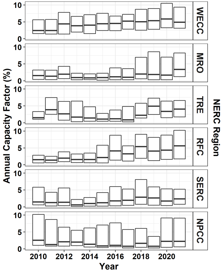
Figure 5: Annual capacity factor (based on gross generation) of simple cycle turbines by year, grouped by NERC Region. Center lines show median values for annual capacity factor from simple cycle units. The upper and lower bounds of each box mark the 25 th and 75 th percentile of the distribution of annual capacity factors for each year.
