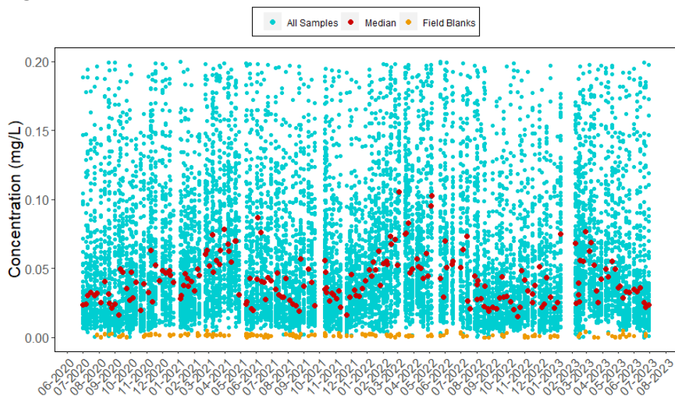
Figure 24. Concentrations of \text{Na}^+ from Teflon Filters
