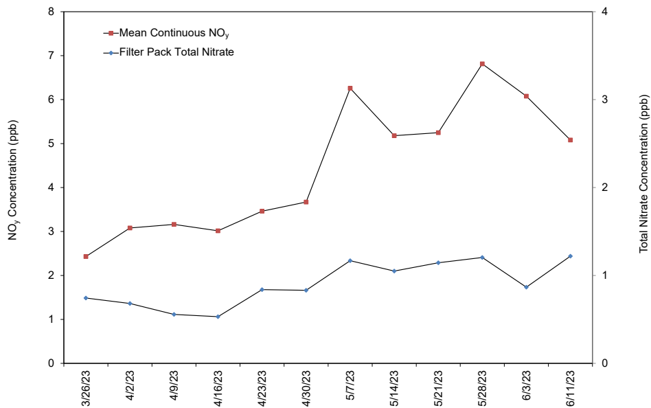
Figure 30. Comparison of BVL130, IL Weekly Mean \text{NO}_y and Total \text{NO}_3^- Concentrations
