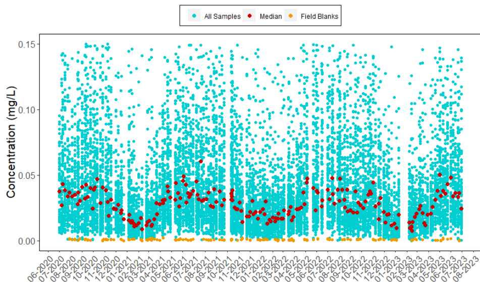
Figure 23. Concentrations of \text{Mg}^{2+} from Teflon Filters
