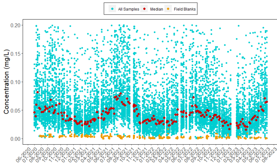
Figure 22. Concentrations of \text{K}^{+} from Teflon Filters
