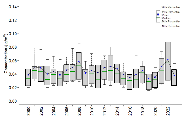
Figure 11. Trends in Second Quarter Mean \text{Mg}^{2+} Concentrations Western Reference Sites
