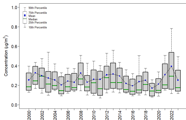
Figure 9. Trends in Second Quarter Mean \text{Ca}^{2+} Concentrations Western Reference Sites
