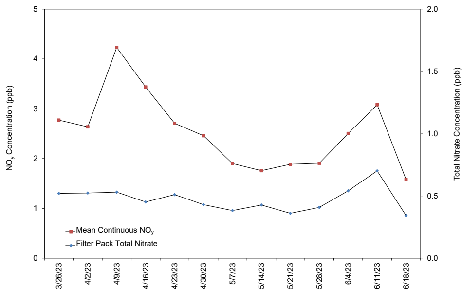
Figure 31. Comparison of MAC426, KY Weekly Mean \text{NO}_y and Total \text{NO}_3^- Concentrations
