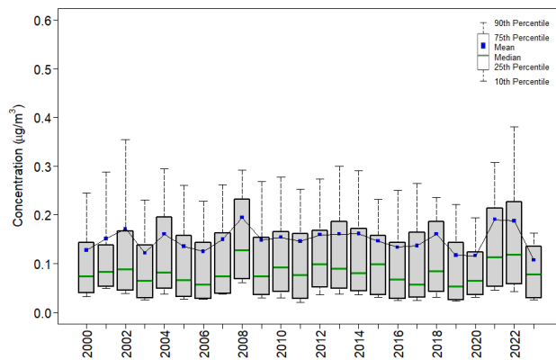
Figure 12. Trends in Second Quarter Mean \text{Na}^+ Concentrations Western Reference Sites
