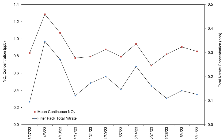
Figure 35. Comparison of PND165, WY Weekly Mean \text{NO}_y and Total \text{NO}_3^- Concentrations
