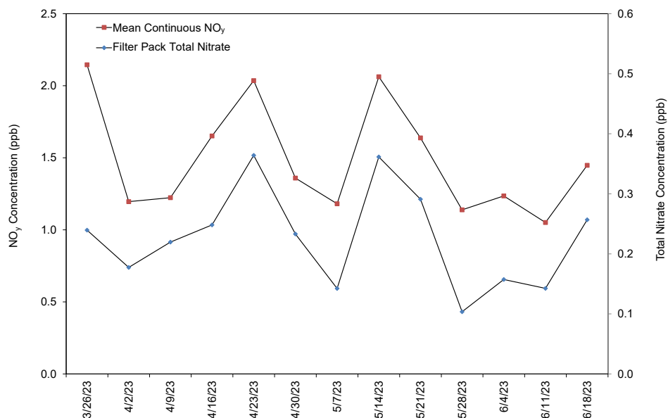
Figure 36. Comparison of ROM206, CO Weekly Mean \text{NO}_y and Total \text{NO}_3^- Concentrations
