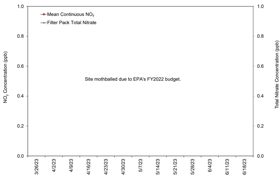
Figure 34. Comparison of PNF126, NC Weekly Mean \text{NO}_y and Total \text{NO}_3^- Concentrations
