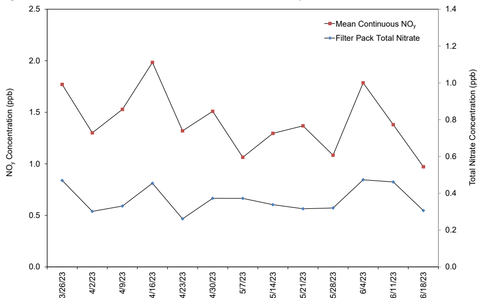
Figure 33. Comparison of GRS420, TN Weekly Mean \text{NO}_y and Total \text{NO}_3^- Concentrations
