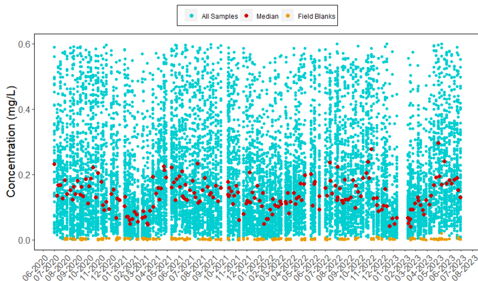
Figure 21. Concentrations of \text{Ca}^{2+} from Teflon Filters
