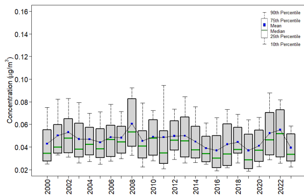
Figure 10. Trends in Second Quarter Mean \text{K}^+ Concentrations Western Reference Sites
