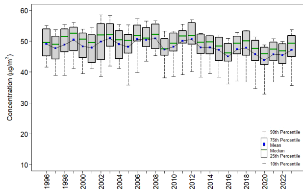
Figure 13. Trends in Second Quarter Mean \text{O}_3 Concentrations Western Reference Sites
