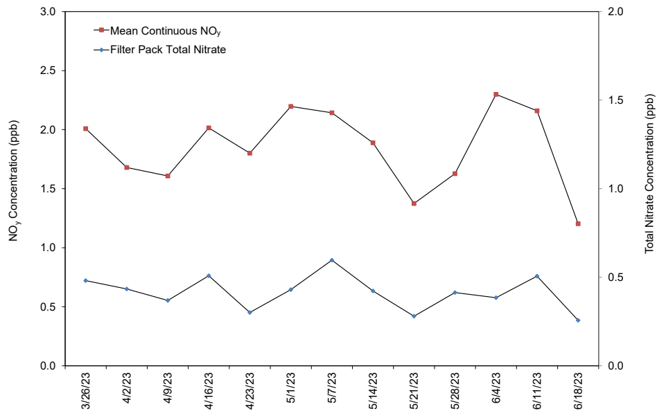
Figure 29. Comparison of DUK008, NC Weekly Mean \text{NO}_y and Total \text{NO}_3^- Concentrations
