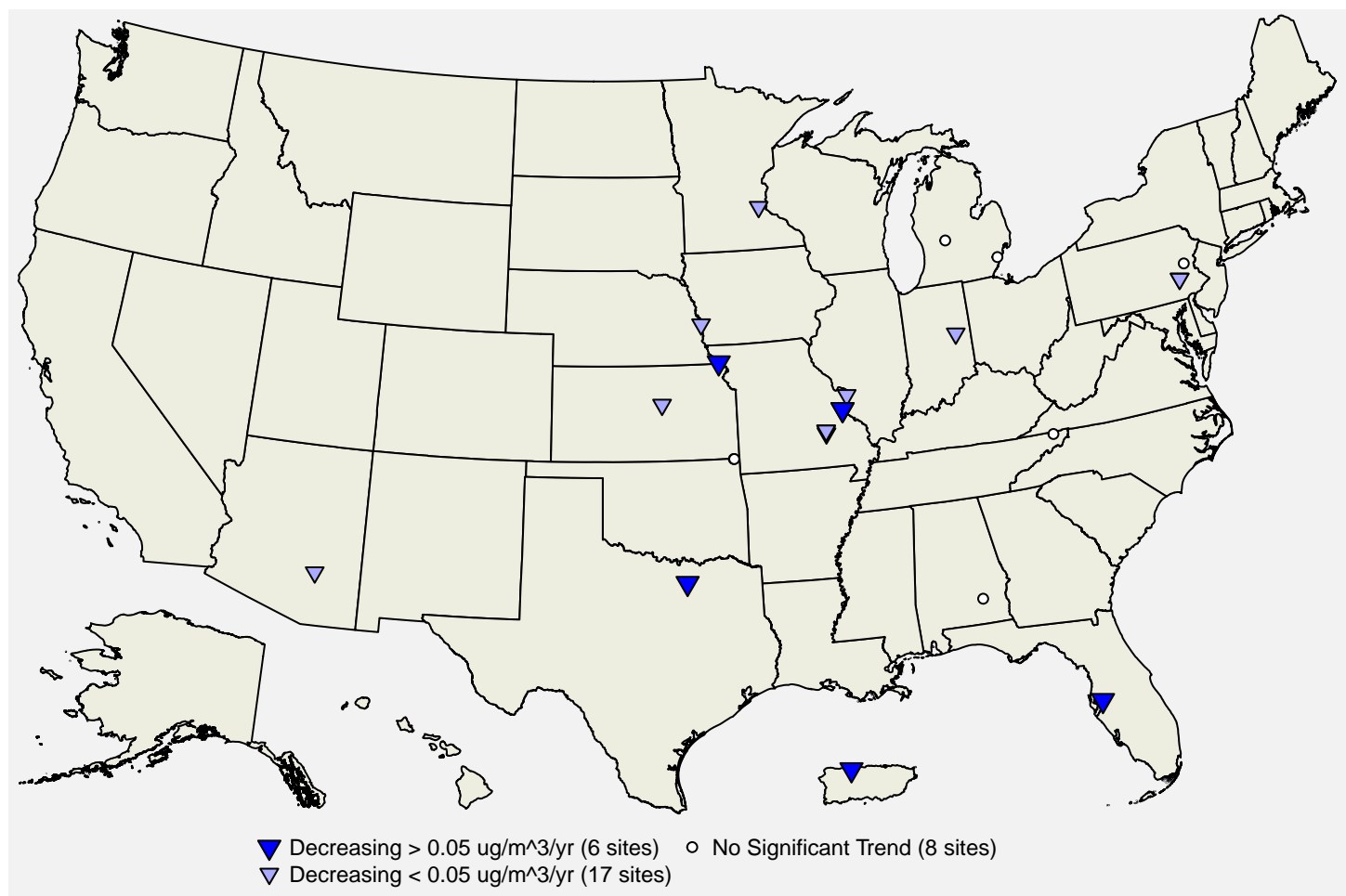
Figure 7: Site-level trends in Pb design values based on data from 2010 through 2023. Source: AQS , trends computed using R statistical software.
