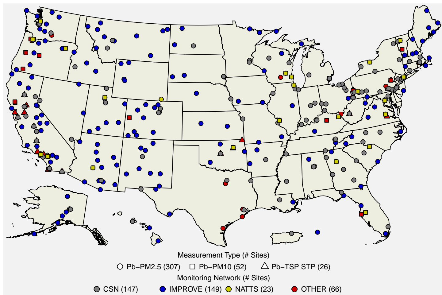
Figure 5: Map of U.S. ambient air monitoring sites reporting non-regulatory Pb data to the EPA during the 2021-2023 period. Source: AQS.
