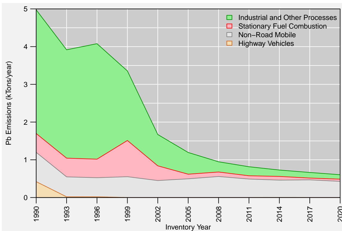
Figure 3. U.S. anthropogenic Pb emissions trend, 1990-2020. Source: Our Nation's Air: Status and Trends Through 2023
