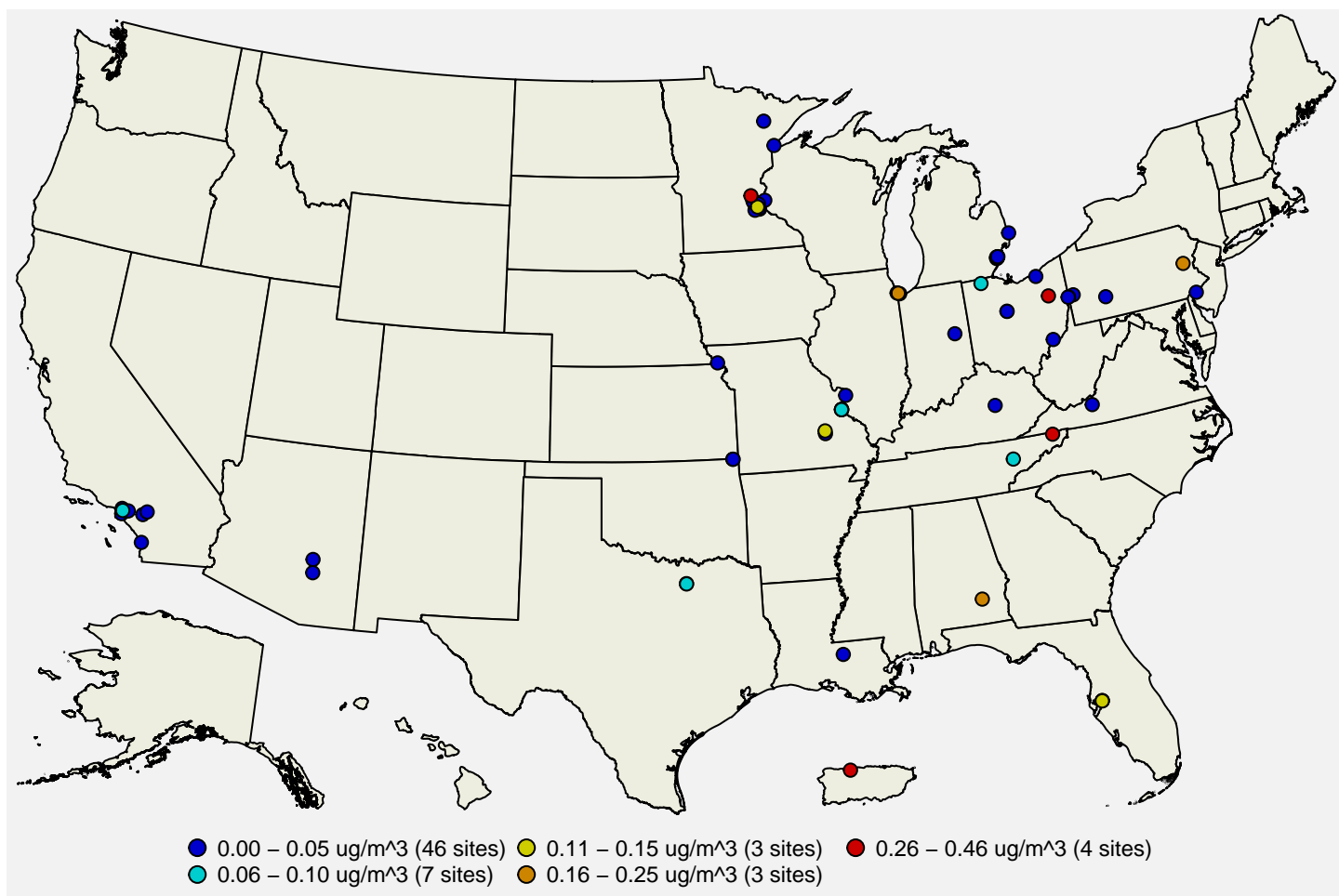
Figure 6: Pb design values in \mu\text{g}/\text{m}^3 for the 2021-2023 period. Source: AQS .
