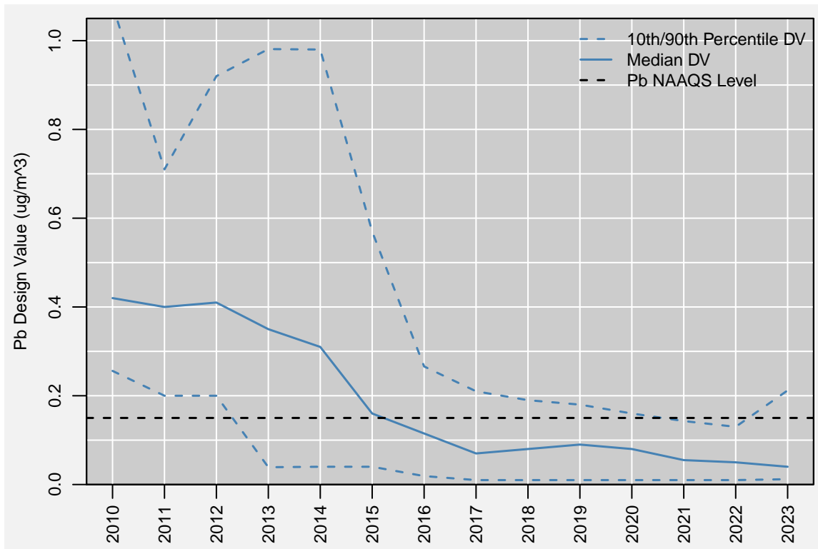
Figure 8: National trend in Pb design values in \mu\text{g}/\text{m}^3 , 2010 to 2023. Source: AQS .
