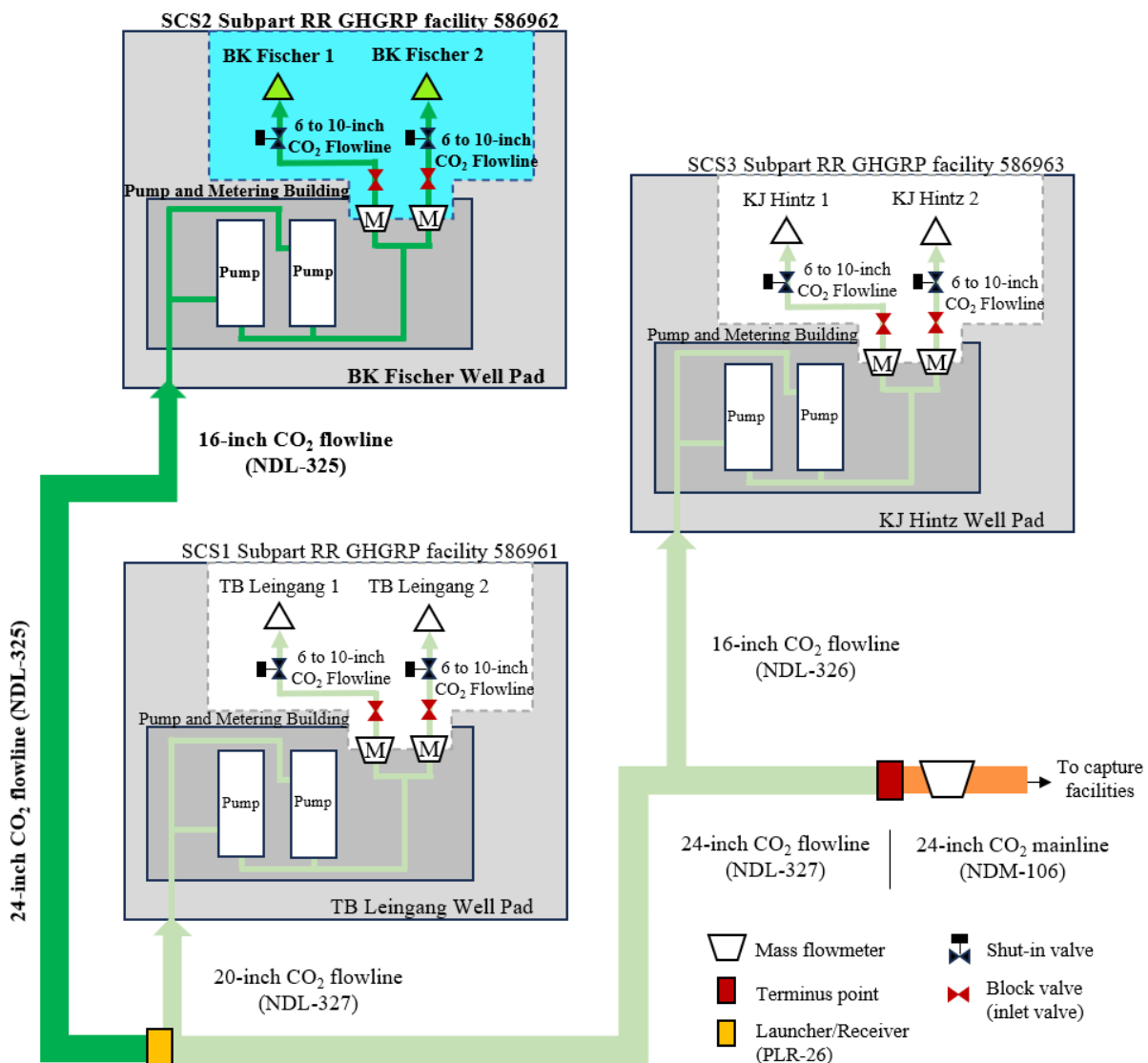
Figure 1-12. Process flow diagram of CO 2 transport to the BK Fischer 1 and 2 injection wells. Area in blue defines the extent of the BK Fischer Subpart RR GHGRP facility.
