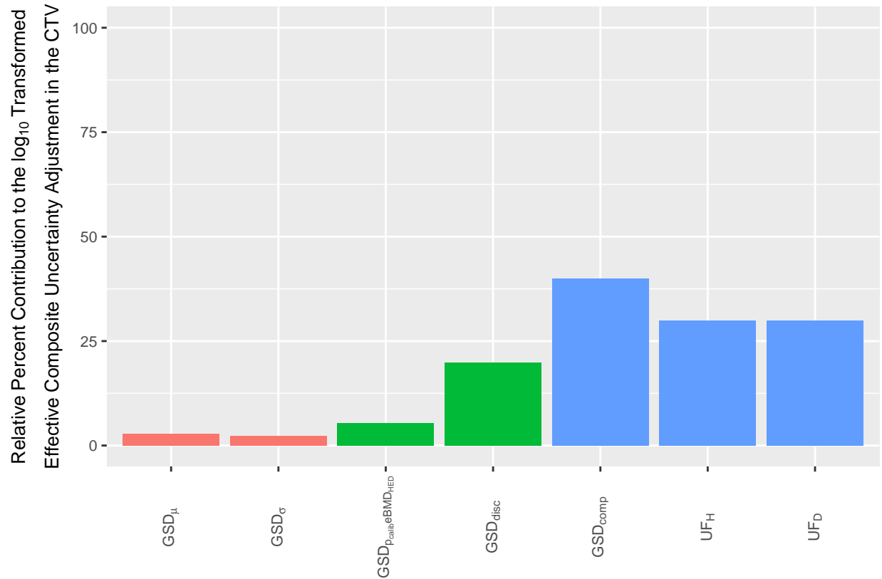
Figure 5: Relative percent contribution to the effective composite uncertainty adjustment in the CTV for Tetralin. Orange bars are the uncertainties surrounding the conversion of the DRSVs to eBMD_{HED} ( GSD_{\mu} ) and the inter-study variability ( GSD_{\sigma} ). The first green bar ( p_{calib} eBMD_{HED} ) is the combined uncertainty from GSD_{\mu} and GSD_{\sigma} . The second green bar ( GSD_{disc} ) is the uncertainty from the calibration process. The first blue bar ( GSD_{comp} ) is the combined uncertainty from the two green bars. The blue bars representing UF_H and UF_D are the uncertainty factors used to account for variation in the susceptibility within the human population and lack of a complete database, respectively.
