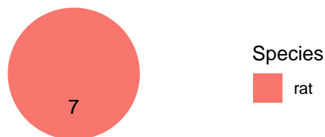
Figure 1: Consolidated study group characteristics reported for Tetralin including (A) data sources; (B) standardized study types; (C) study durations; and (D) study species.
