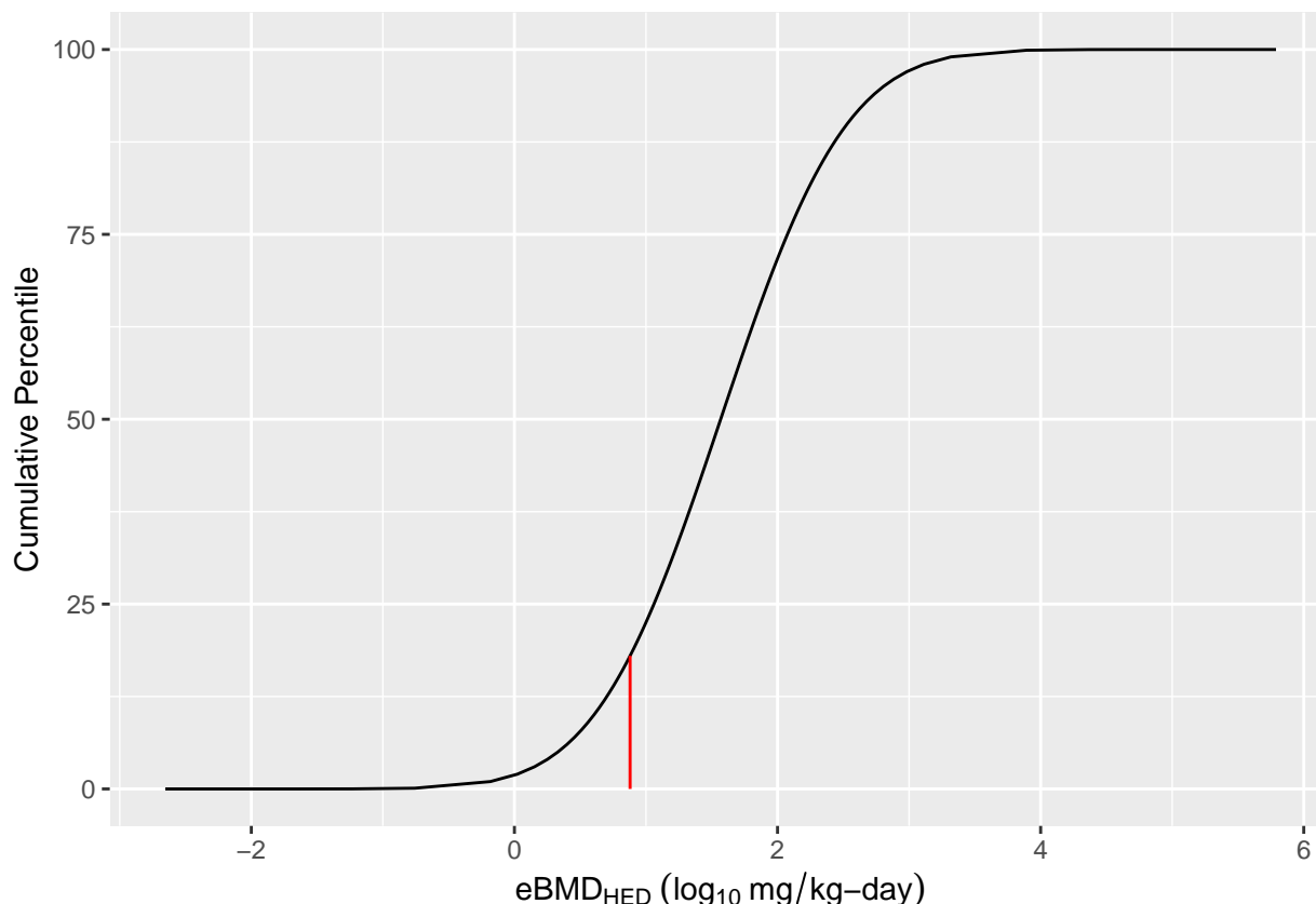
Figure 4: Cumulative distribution of eBMD_{HED} values for Tetralin. The 18th percentile in the distribution ( p_{calib}eBMD_{HED} ) is highlighted with the red line.
