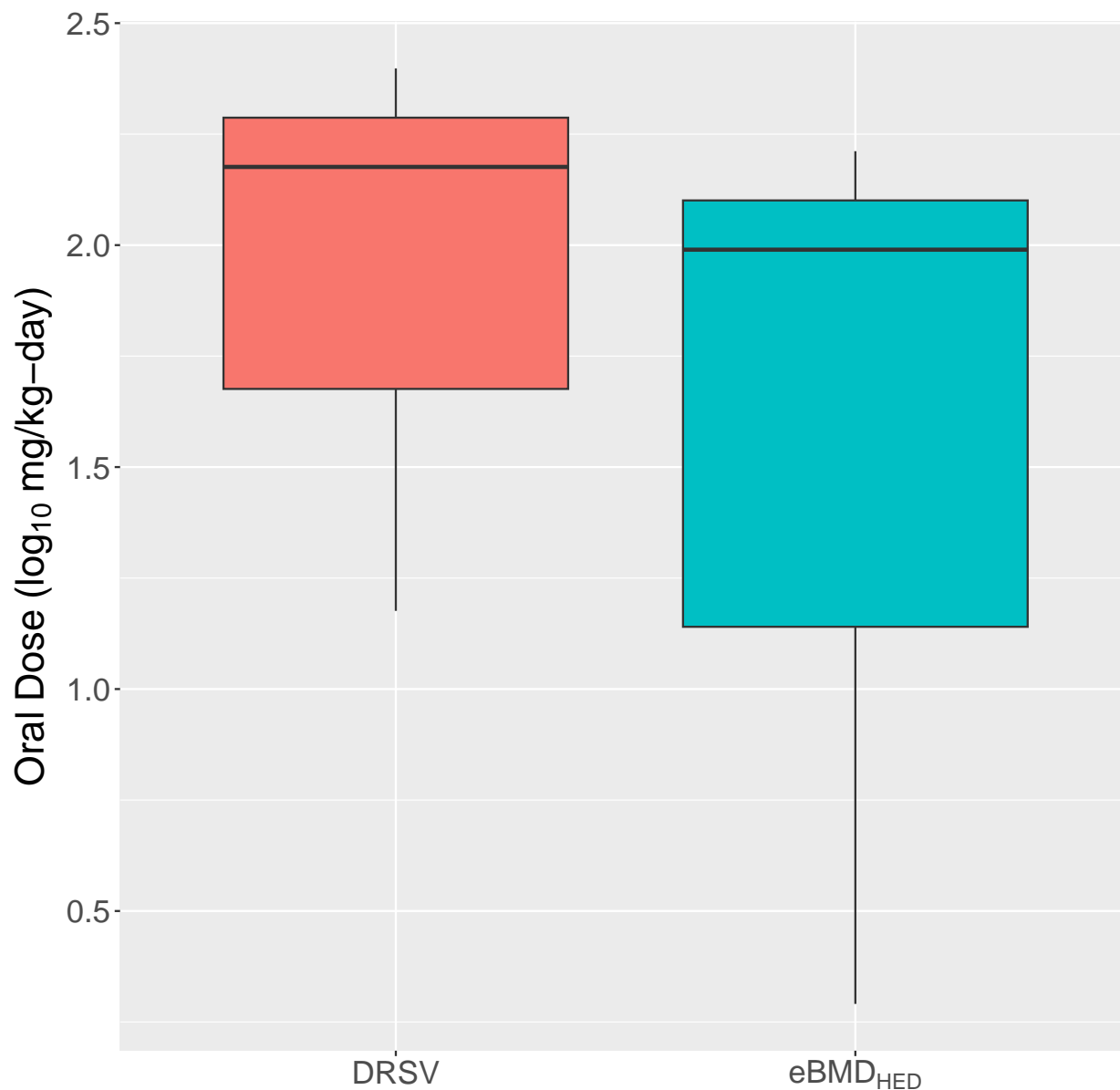
Figure 3: Box and whisker plots of the reported DRSVs (red) and chronic eBMD HED values (blue) for Tetralin. The box represents the inter-quartile range between the 25th and 75th percentiles, while the horizontal line inside the box denotes the median. The whiskers represent the largest (or smallest) observation that is within 1.5 times the interquartile range above Q3 (or below Q1). Observations that fall outside the whiskers are shown individually as dots.
