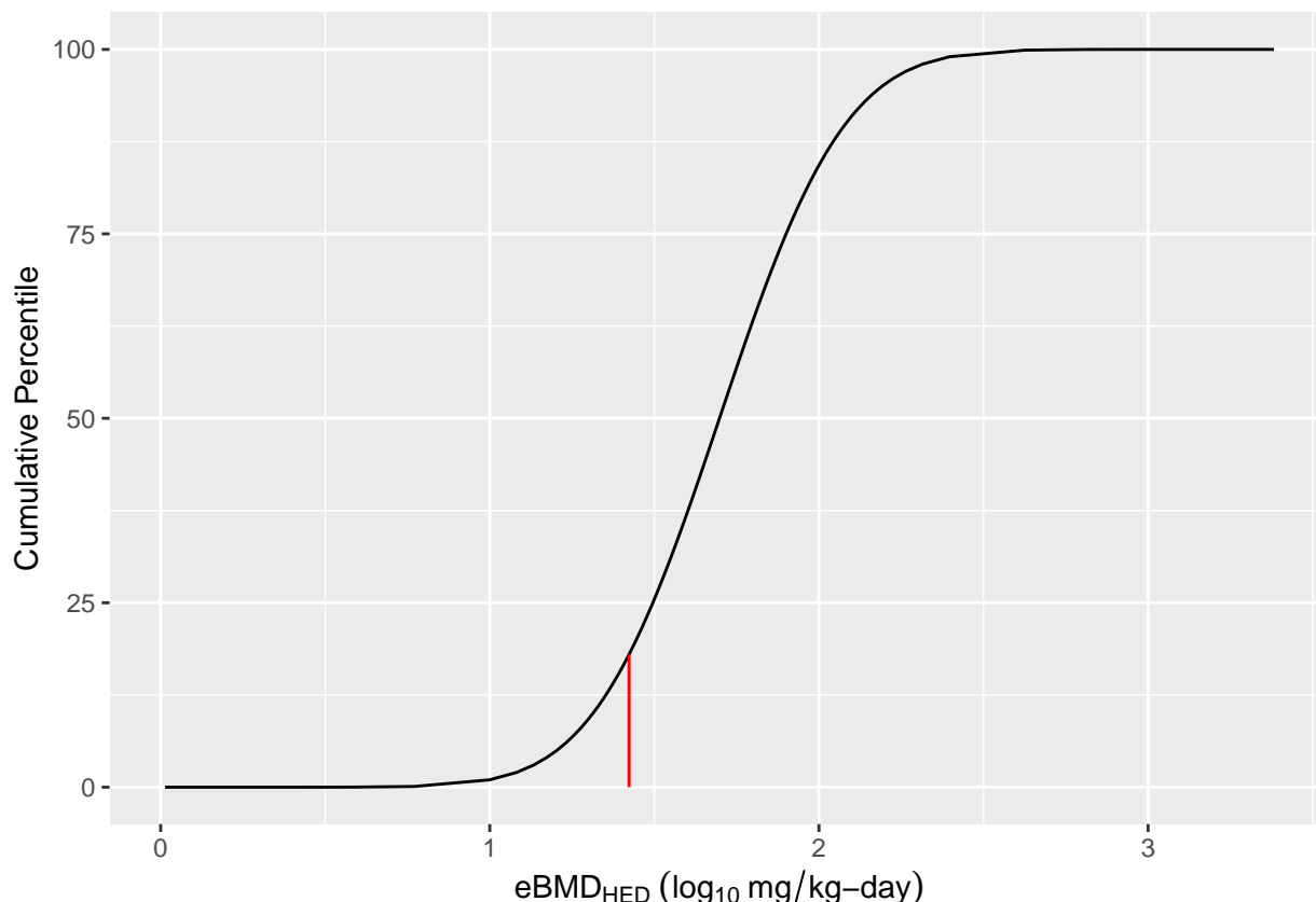
Figure 4: Cumulative distribution of eBMD HED values for 4-Ethyltoluene. The 18th percentile in the distribution ( p_{\text{calib}}\text{eBMD}_{\text{HED}} ) is highlighted with the red line.
