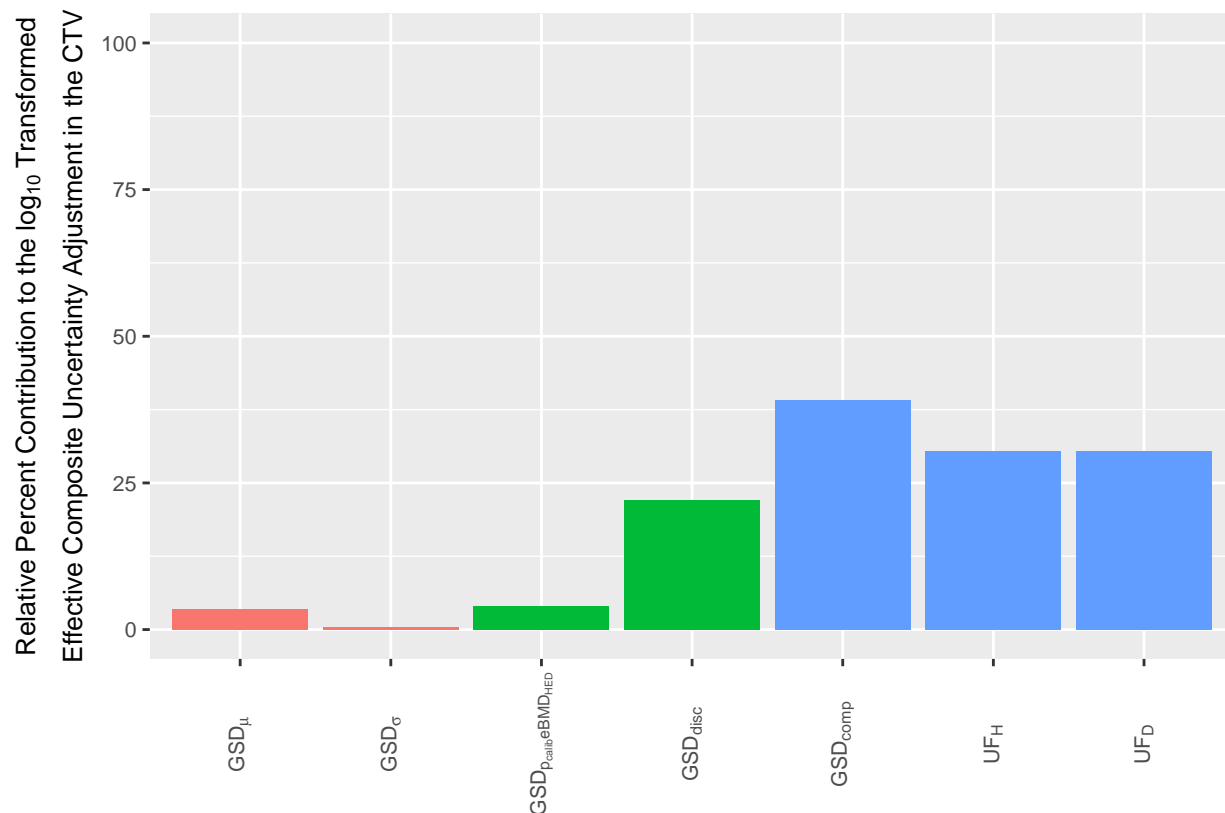
Figure 5: Relative percent contribution to the effective composite uncertainty adjustment in the CTV for 4-Ethyltoluene. Orange bars are the uncertainties surrounding the conversion of the DRSVs to eBMD_{HED} ( GSD_{\mu} ) and the inter-study variability ( GSD_{\sigma} ). The first green bar ( p_{calib} \text{ eBMD}_{HED} ) is the combined uncertainty from GSD_{\mu} and GSD_{\sigma} . The second green bar ( GSD_{disc} ) is the uncertainty from the calibration process. The first blue bar ( GSD_{comp} ) is the combined uncertainty from the two green bars. The blue bars representing UF_H and UF_D are the uncertainty factors used to account for variation in the susceptibility within the human population and lack of a complete database, respectively.
