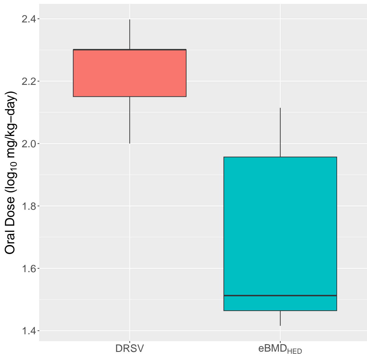
Figure 3: Box and whisker plots of the reported DRSVs (red) and chronic eBMD HED values (blue) for 4-Ethyltoluene. The box represents the inter-quartile range between the 25th and 75th percentiles, while the horizontal line inside the box denotes the median. The whiskers represent the largest (or smallest) observation that is within 1.5 times the interquartile range above Q3 (or below Q1). Observations that fall outside the whiskers are shown individually as dots.
