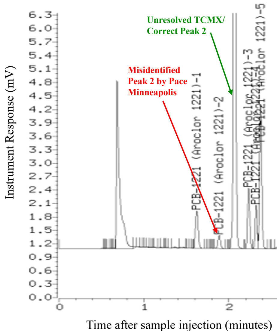
Example Chromatograms for Aroclor 1221 Calibration Standard in 2021 and 2017
