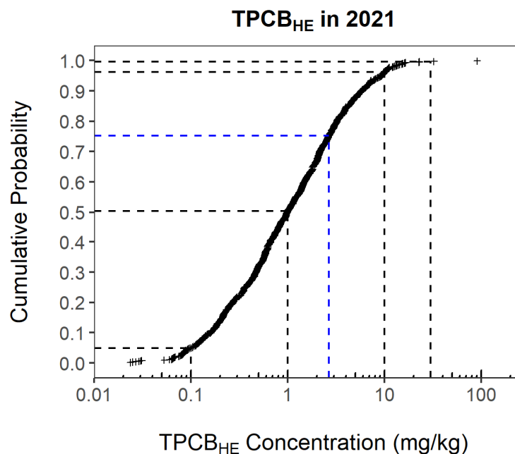
Cumulative Probability Distribution of PCB Concentrations in Surface Sediments
