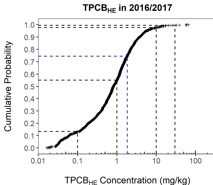
Cumulative Probability Distribution of PCB Concentrations in Surface Sediments
