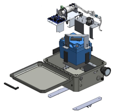
Figure 1: The Canary X Device
