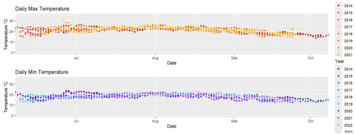
Figure 111: Daily Maximum and Minimum Temperatures at Pass Creek at Mouth (30161-ORDEQ)
