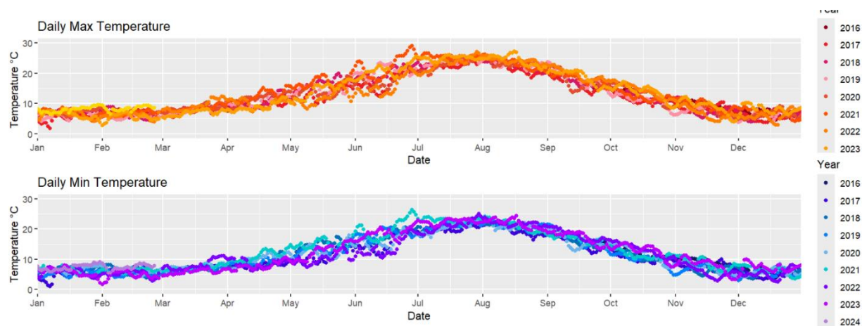
Figure 53: Daily Maximum and Minimum Temperatures at North Umpqua River at Winchester Oregon (USGS-14319500)
