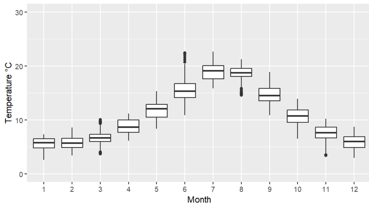
Figure 68: 7DADM Temperature Boxplot at North Umpqua River Near Idleyld Park, Oregon (USGS-14317450)
