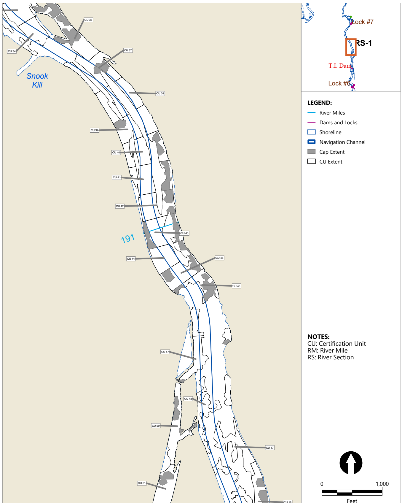
Figure 3 Hudson River Dredging Project: Cap Areas: RM 191 Prepared for General Electric Company
