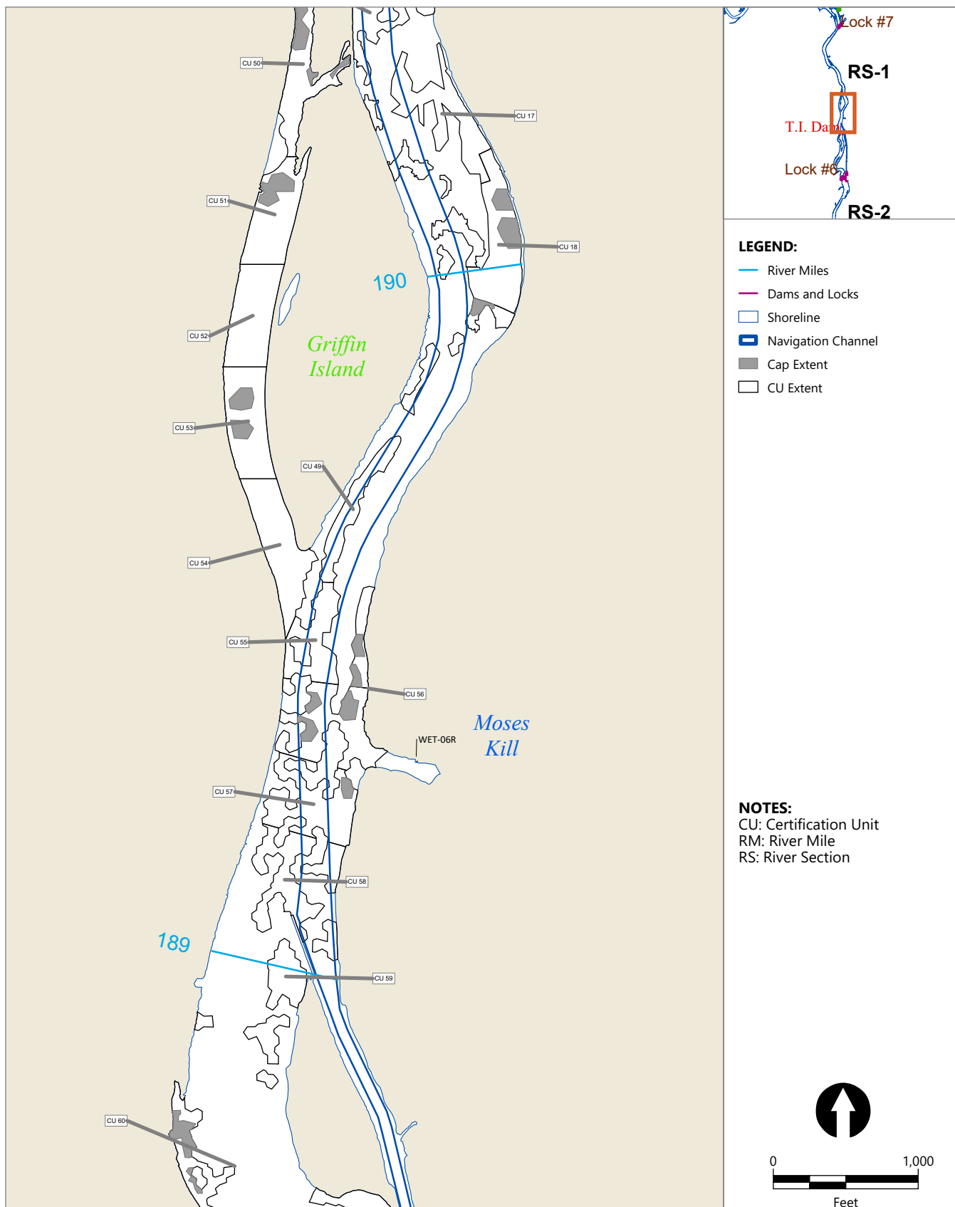
Figure 4 Hudson River Dredging Project: Cap Areas: RM 189-190 Prepared for General Electric Company
