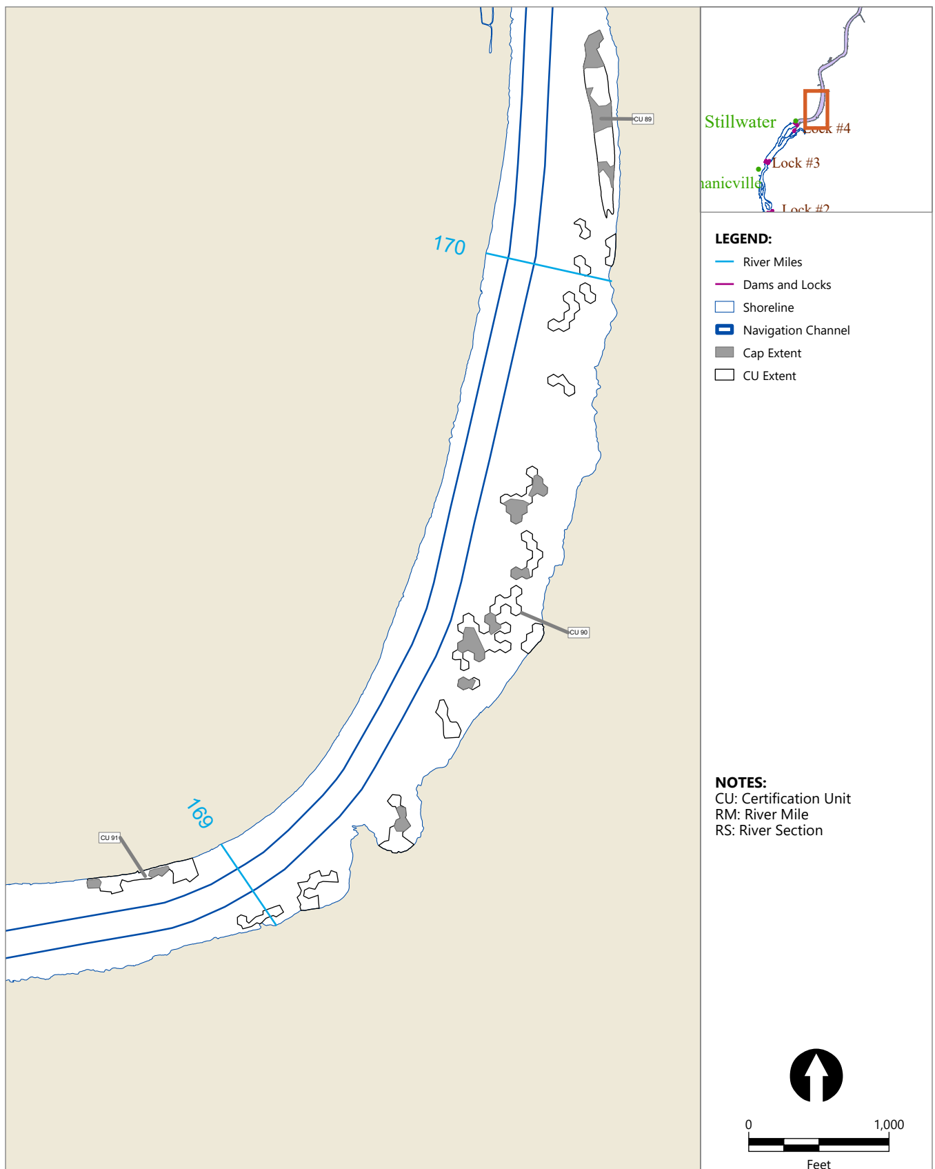
Figure 18 Hudson River Dredging Project: Cap Areas: RM 169-170 Prepared for General Electric Company
