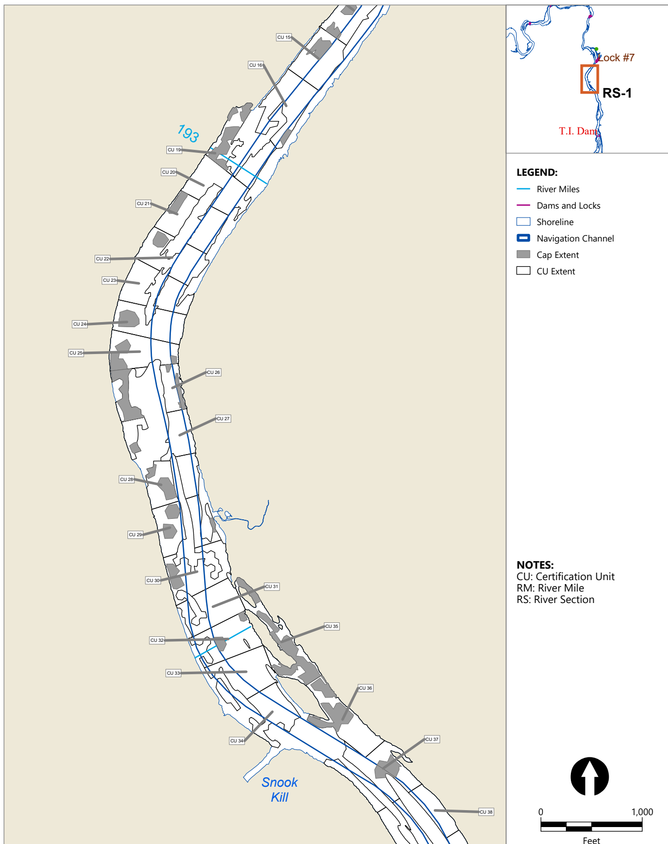
Figure 2 Hudson River Dredging Project: Cap Areas: RM 192-193 Prepared for General Electric Company
