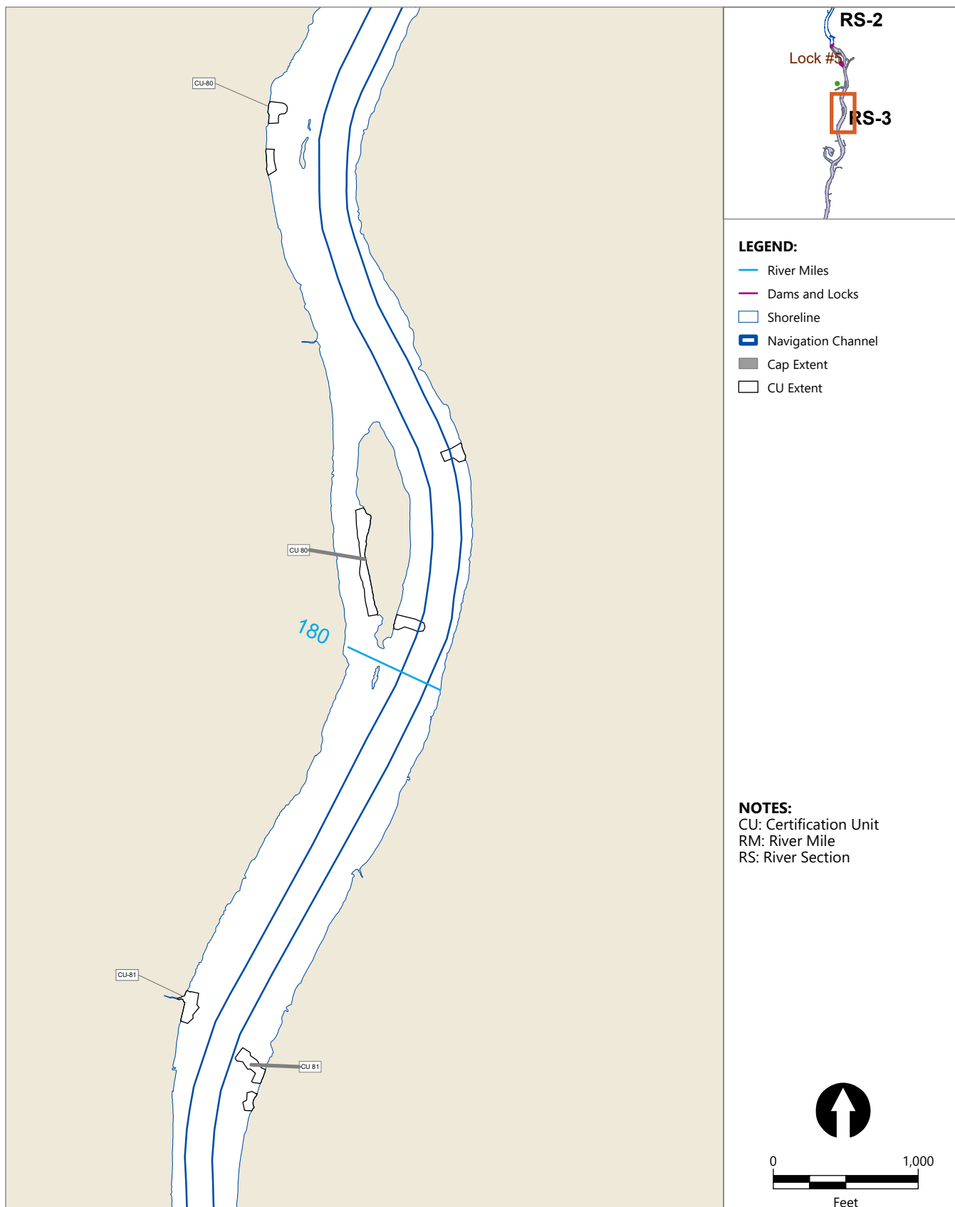
Figure 11 Hudson River Dredging Project: Cap Areas: RM 180 Prepared for General Electric Company
