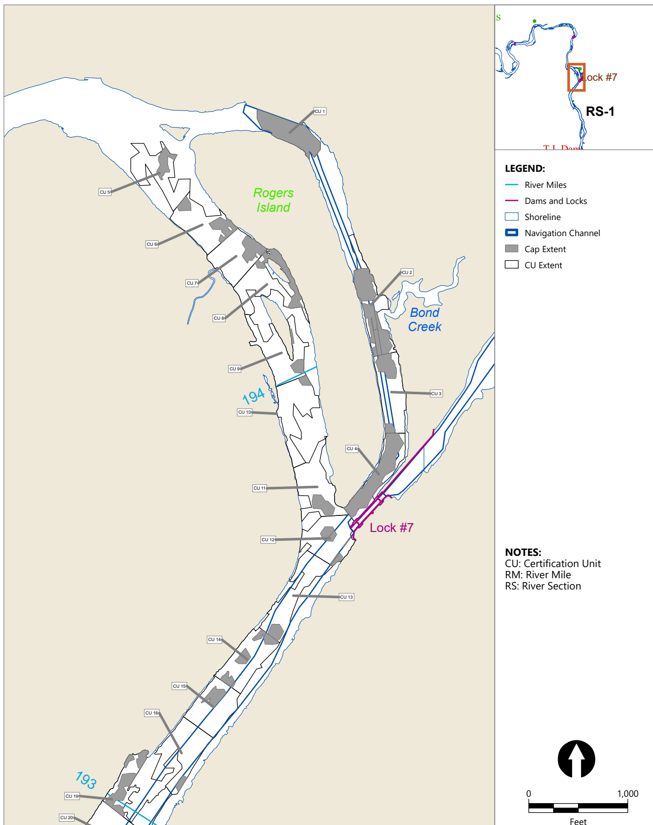
Figure 1 Hudson River Dredging Project: Cap Areas: RM 194 Prepared for General Electric Company
