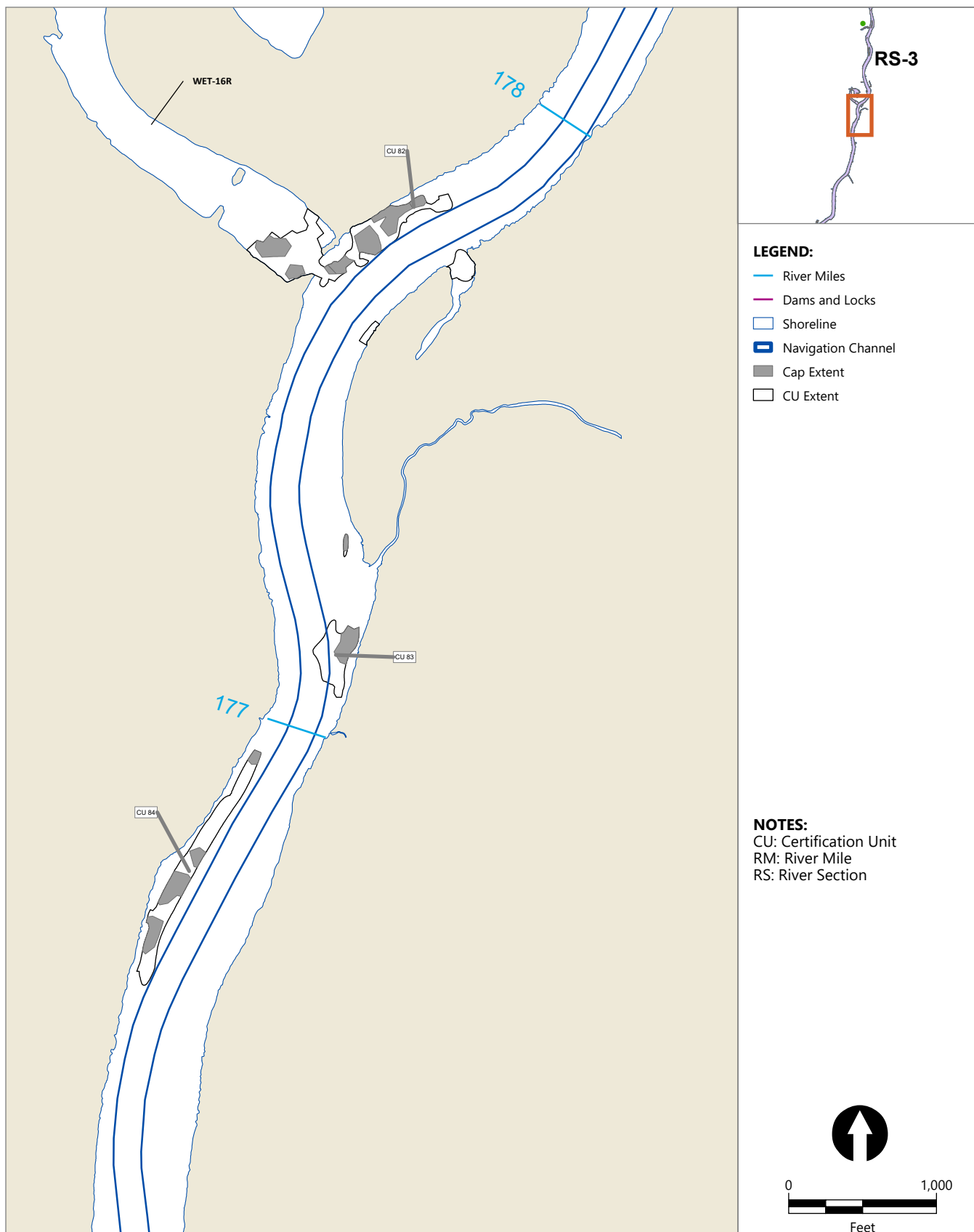
Figure 13 Hudson River Dredging Project: Cap Areas: RM 177-178 Prepared for General Electric Company
