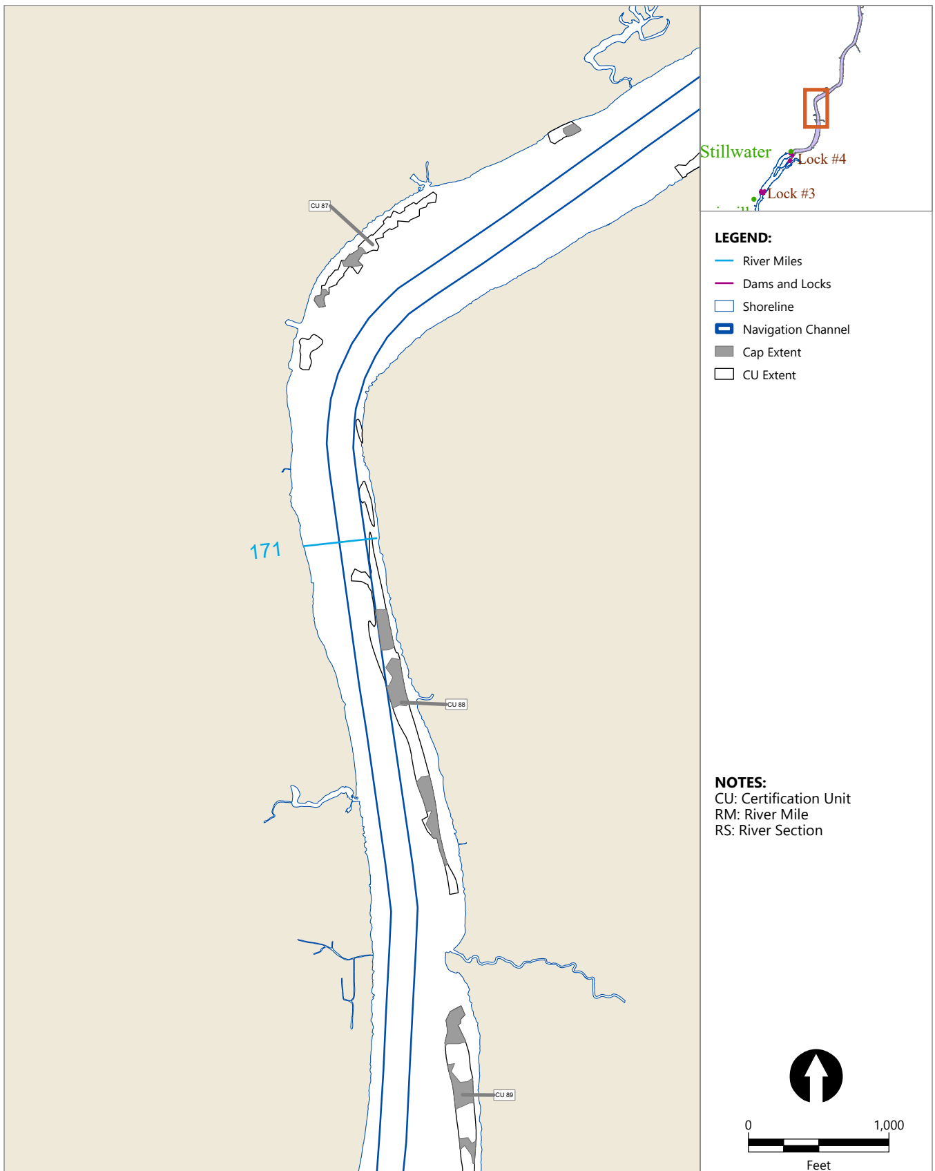
Figure 17 Hudson River Dredging Project: Cap Areas: RM 171 Prepared for General Electric Company
