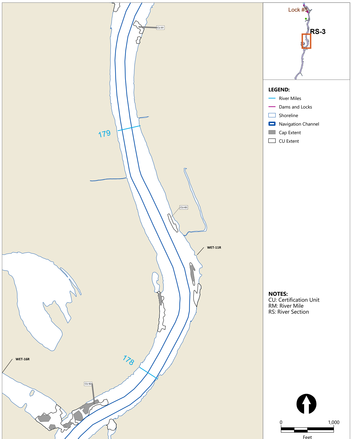
Figure 12 Hudson River Dredging Project: Cap Areas: RM 179 Prepared for General Electric Company
