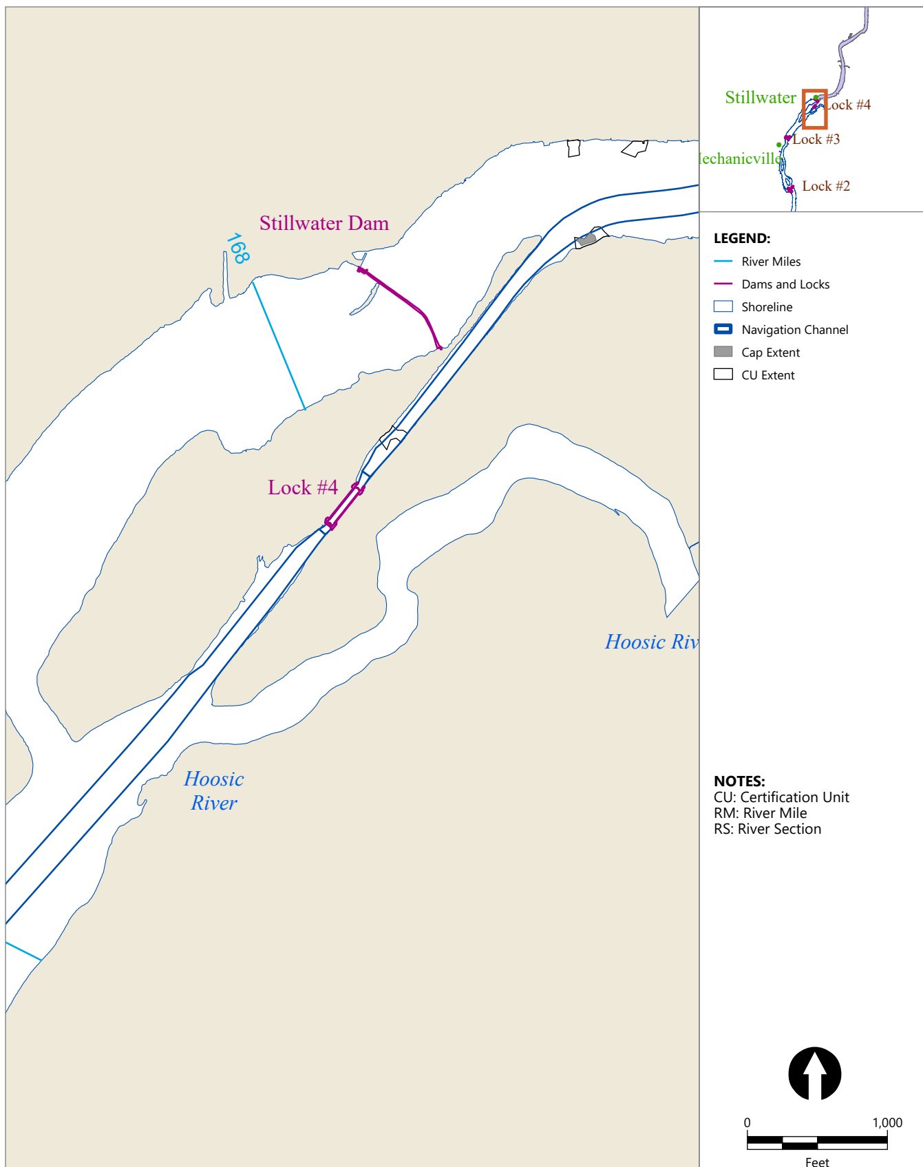
Figure 19 Hudson River Dredging Project: Cap Areas: RM 168 Prepared for General Electric Company
