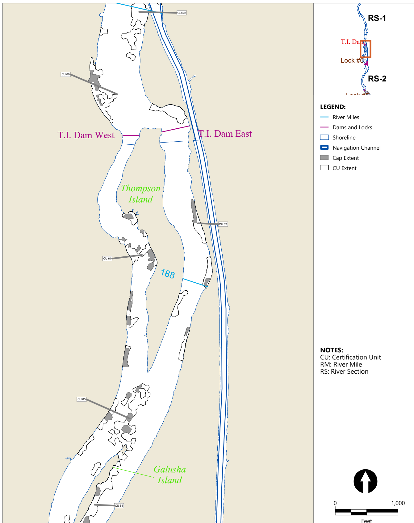
Figure 5 Hudson River Dredging Project: Cap Areas: RM 188 Prepared for General Electric Company
