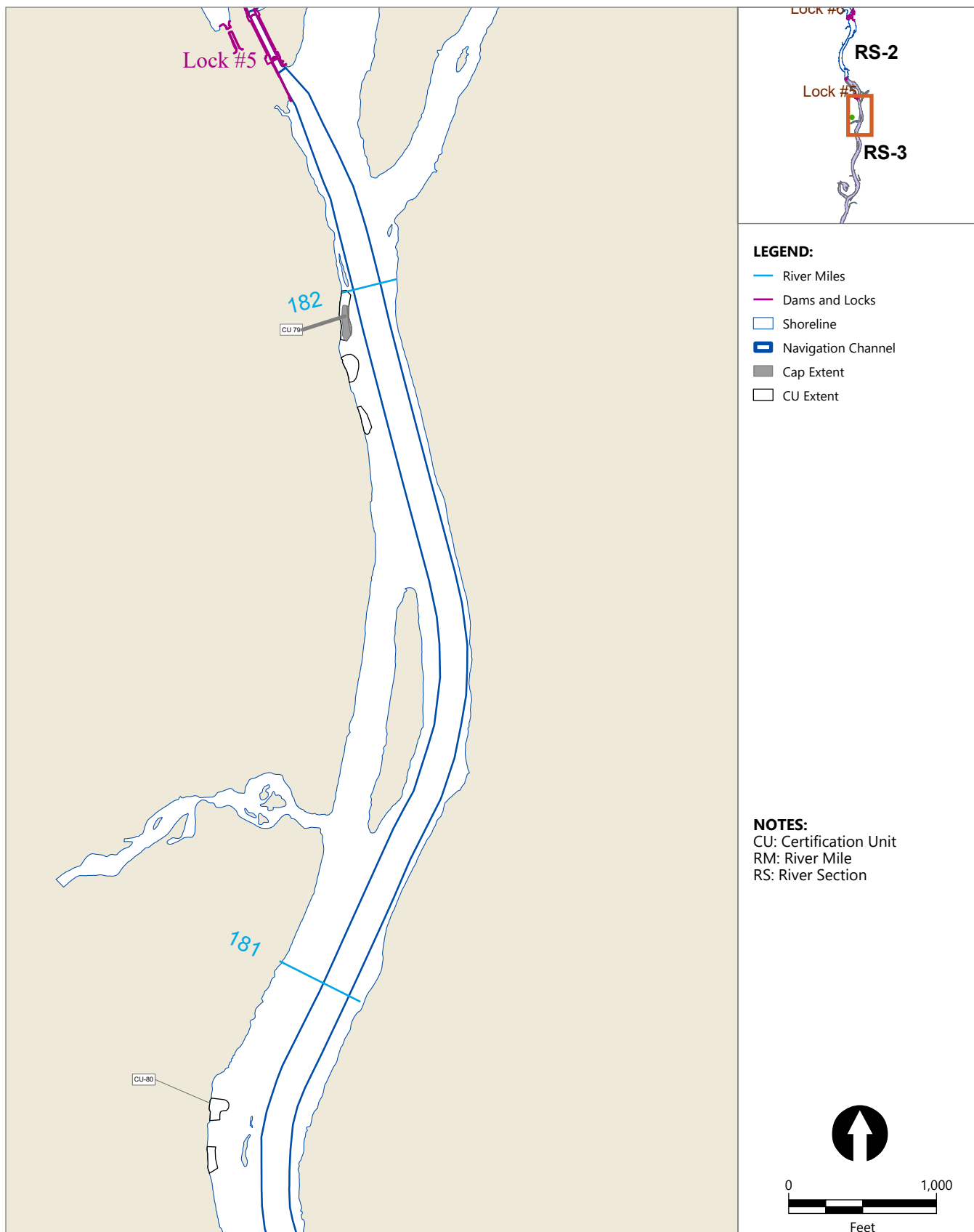
Figure 10 Hudson River Dredging Project: Cap Areas: RM 181-182 Prepared for General Electric Company
