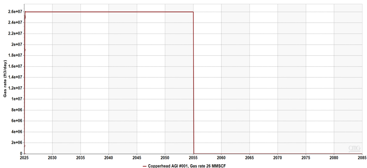
Figure 3.8-4: Forecast of TAG injection rate of Copperhead AGI #001 (2025 to 2055, 26 MMSCFD).
