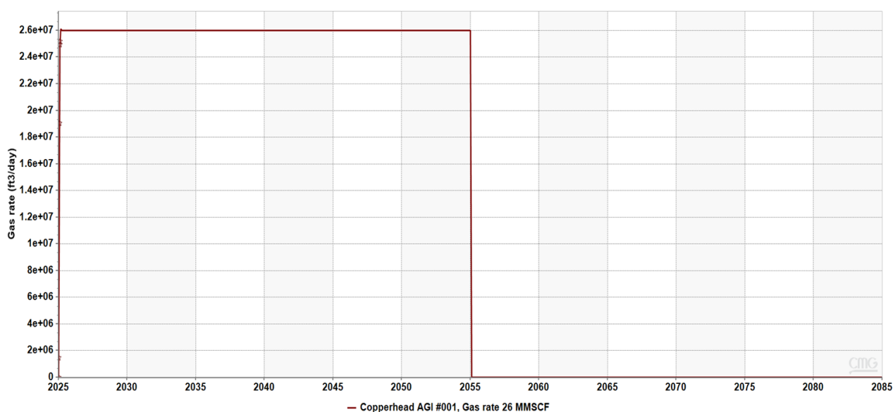
Figure 3.8-4: Forecast of TAG injection rate of the Copperhead AGI #001 well (2025 to 2055, 26 MMSCFD).
