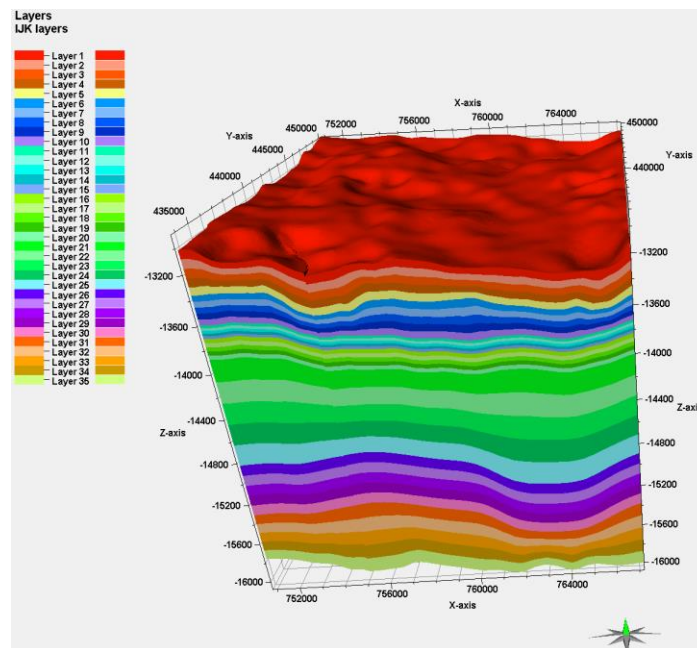
Figure 3.8-1: 3D view of the simulation model.
