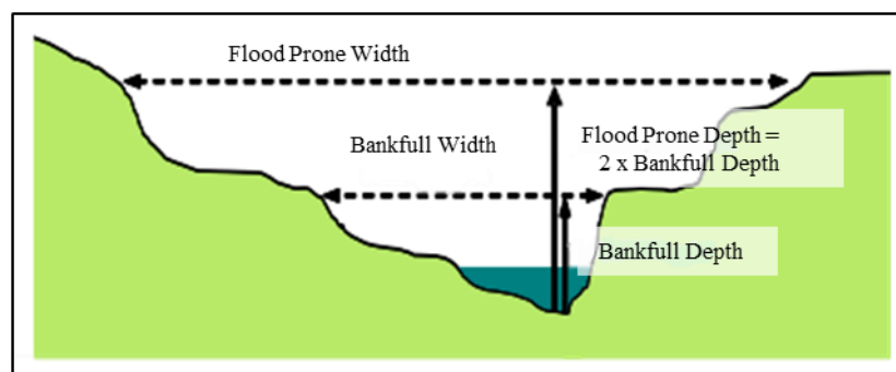
Figure 8. Measurement of entrenchment is based on the ratio of the flood-prone width to the bankfull width.
