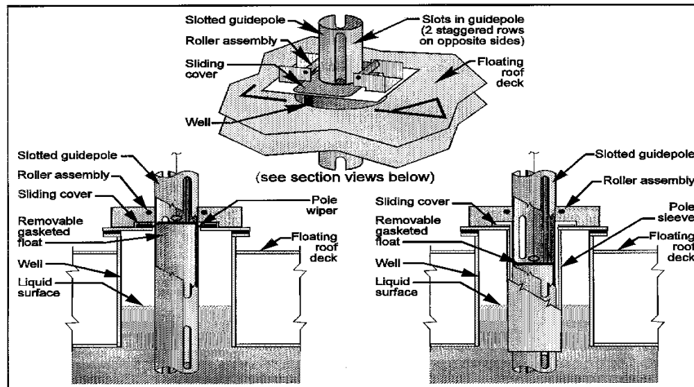
Slotted (perforated) Guidepole
