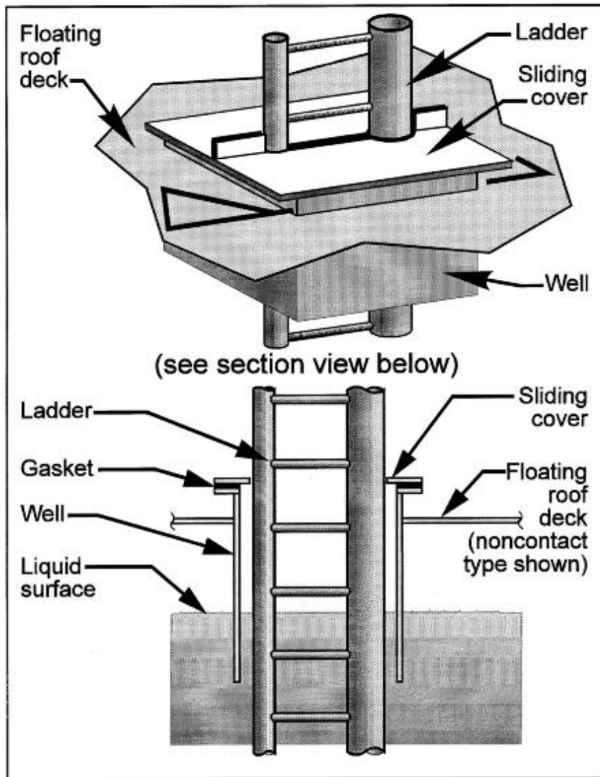
Figure 7.1-12. Ladder well. 20
