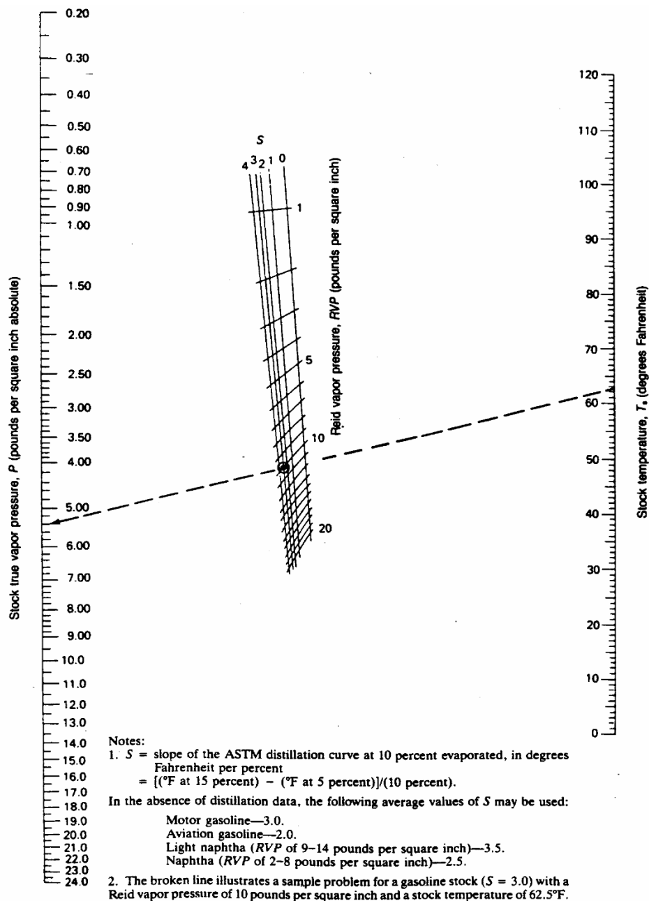
Figure 7.1-14a. True vapor pressure of refined petroleum stocks with Reid vapor pressures of 1 to 20 psi. 4
