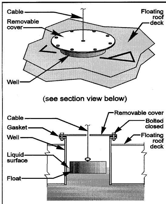
Gauge float
