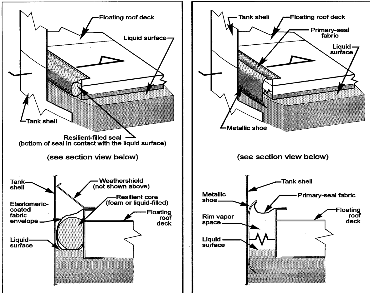
Figure 7.1-7. Liquid-mounted and mechanical shoe primary seals. 20
