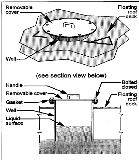
Access Hatch
