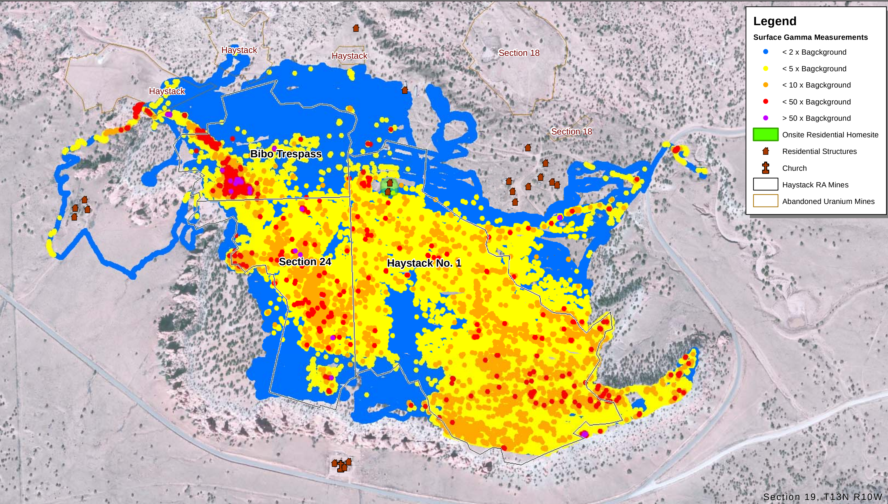
FIGURE #4 SURFACE GAMMA RADIATION Haystack No. 1 Removal Assessment Baca/Haystack Chapter, Navajo Nation, NM
