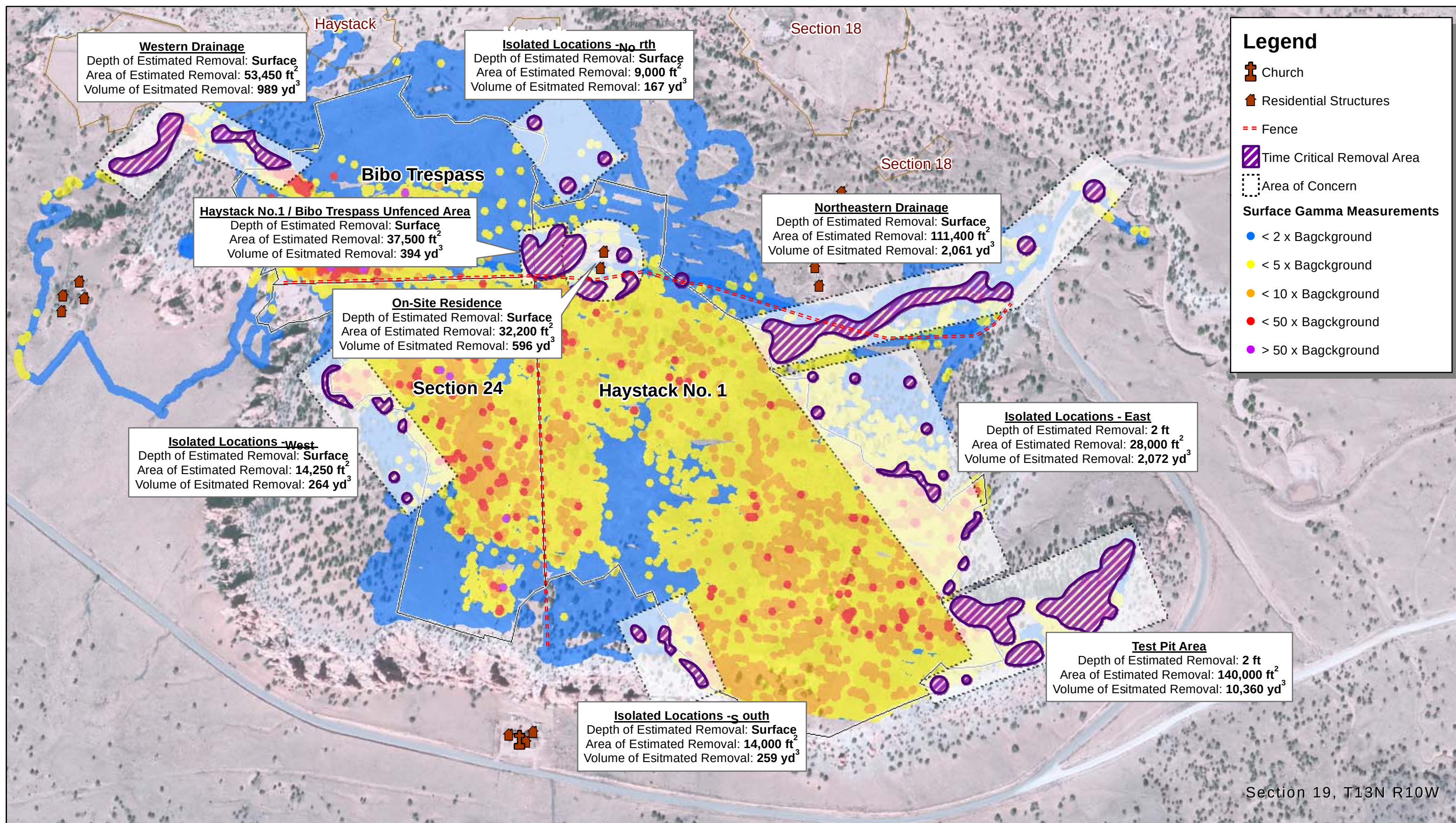
FIGURE #9 TIME CRITICAL REMOVAL AREA Haystack No. 1 Removal Assessment Baca/Haystack Chapter, Navajo Nation, NM
