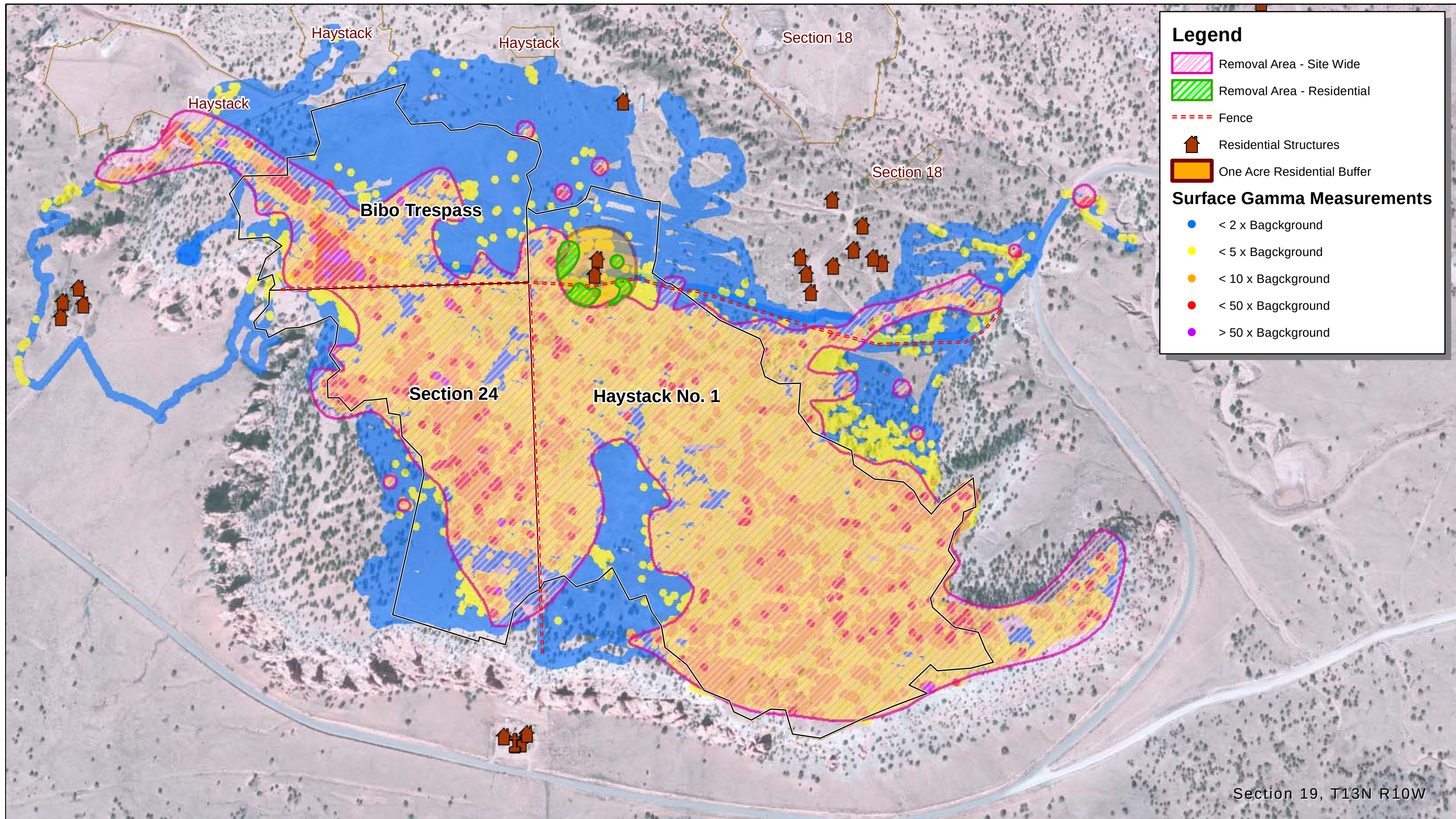
FIGURE #8 SITE WIDE REMOVAL AREA Haystack No. 1 Removal Assessment Baca/Haystack Chapter, Navajo Nation, NM
