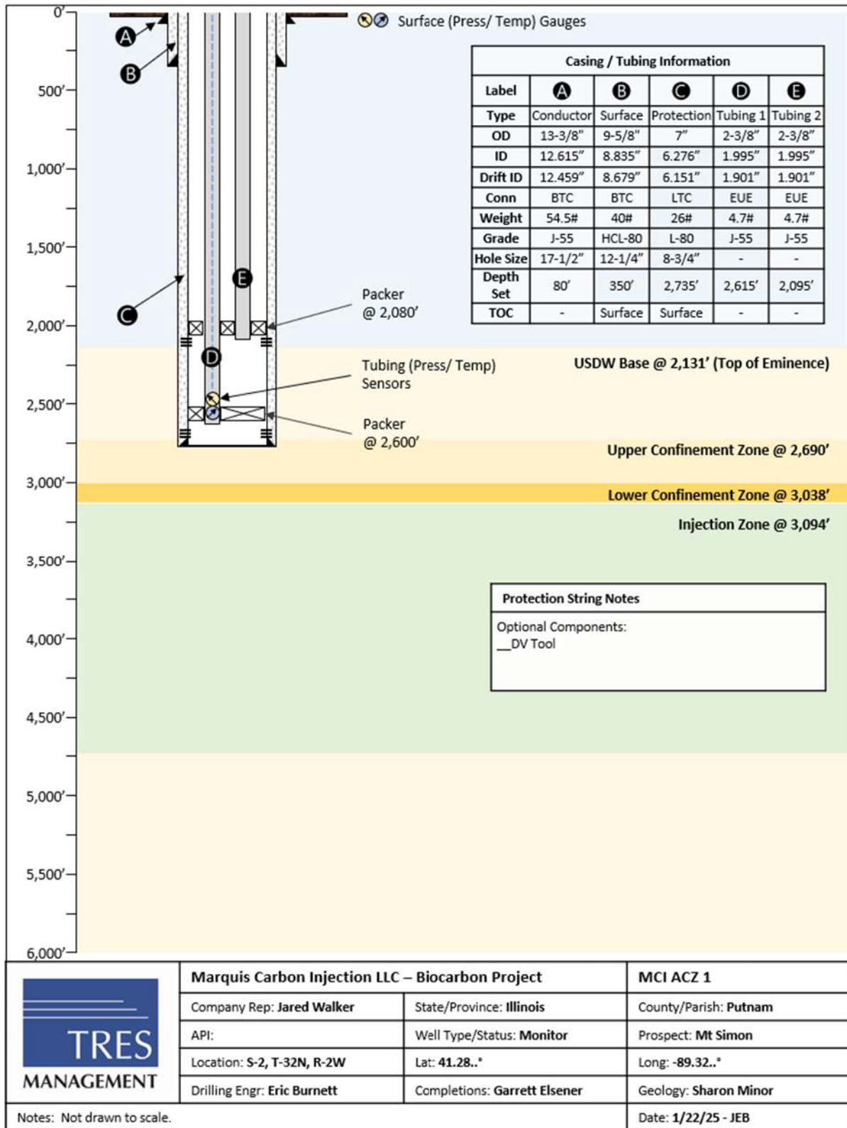
Figure 2: Groundwater Monitoring Well Construction Diagram (MCI ACZ 1).
