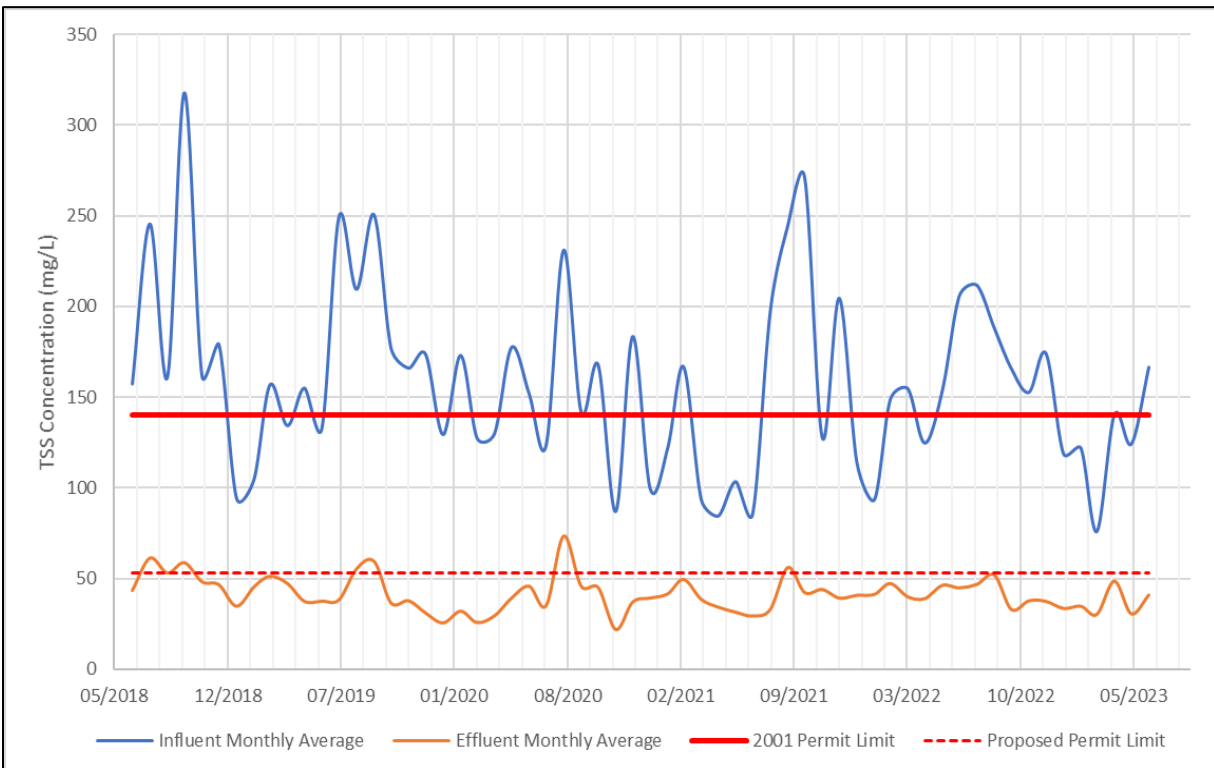
Figure 2. Average Monthly Influent and Effluent TSS Concentrations (06/2018-05/2023)
