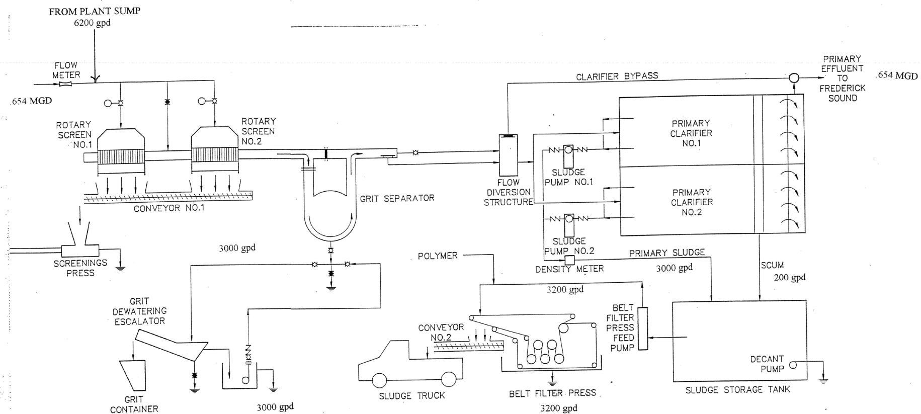
Figure 9. Process Schematic
