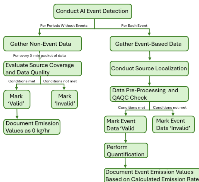
Figure 2. A diagram showing the general data processing and quantification workflow. Quantification is performed at an event-scale across the screening period and undergoes data quality validation.
