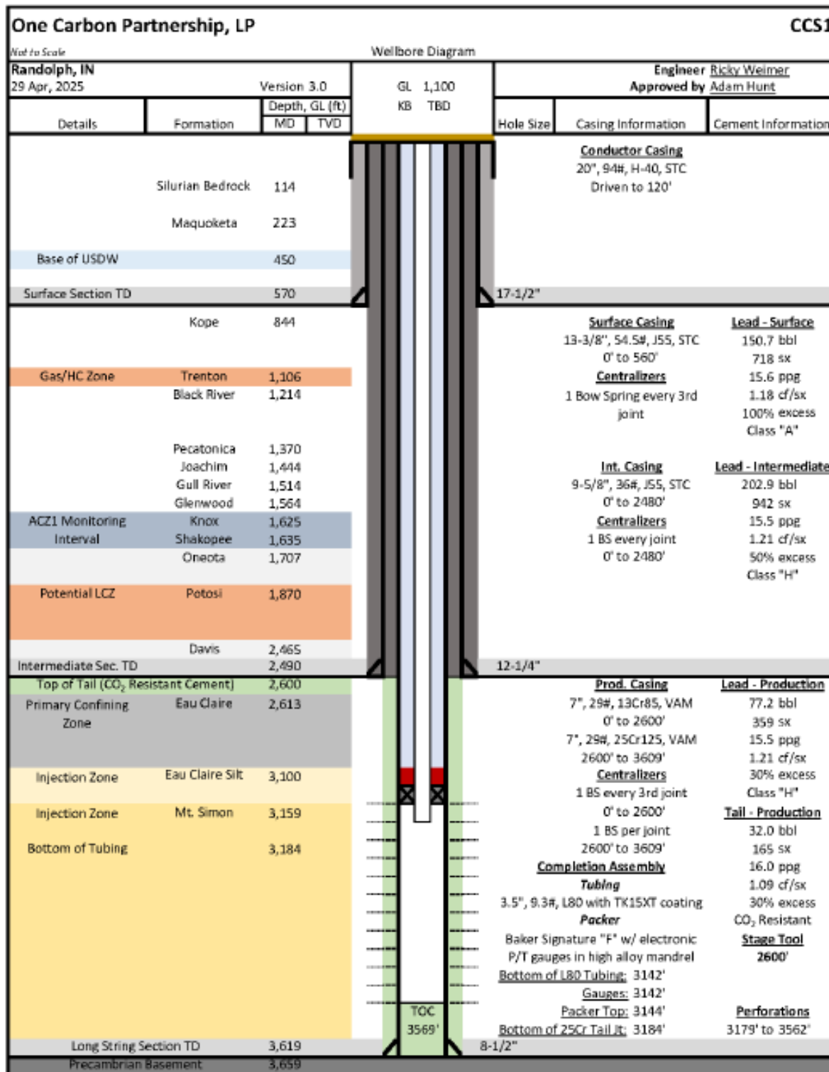
Figure 2: Contingency Injection Well Construction Diagram 1
