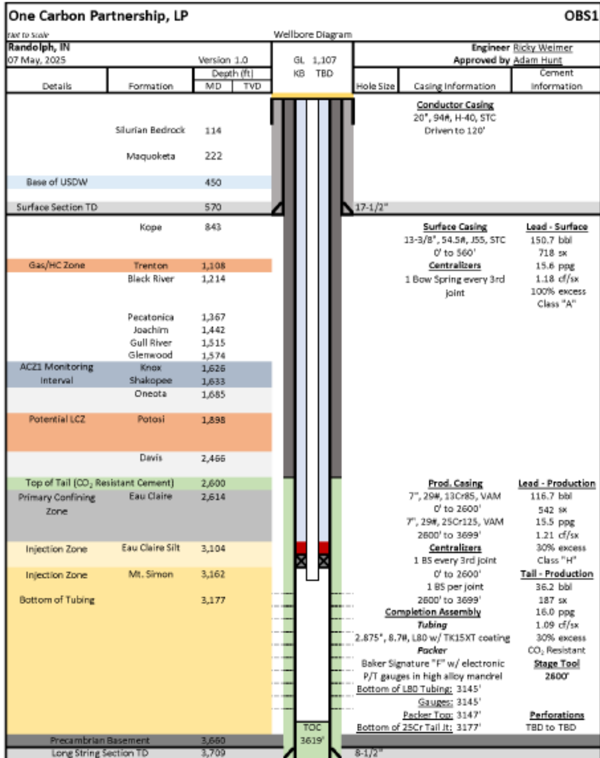
Figure 4: Injection Zone Monitoring Well Construction Diagram
