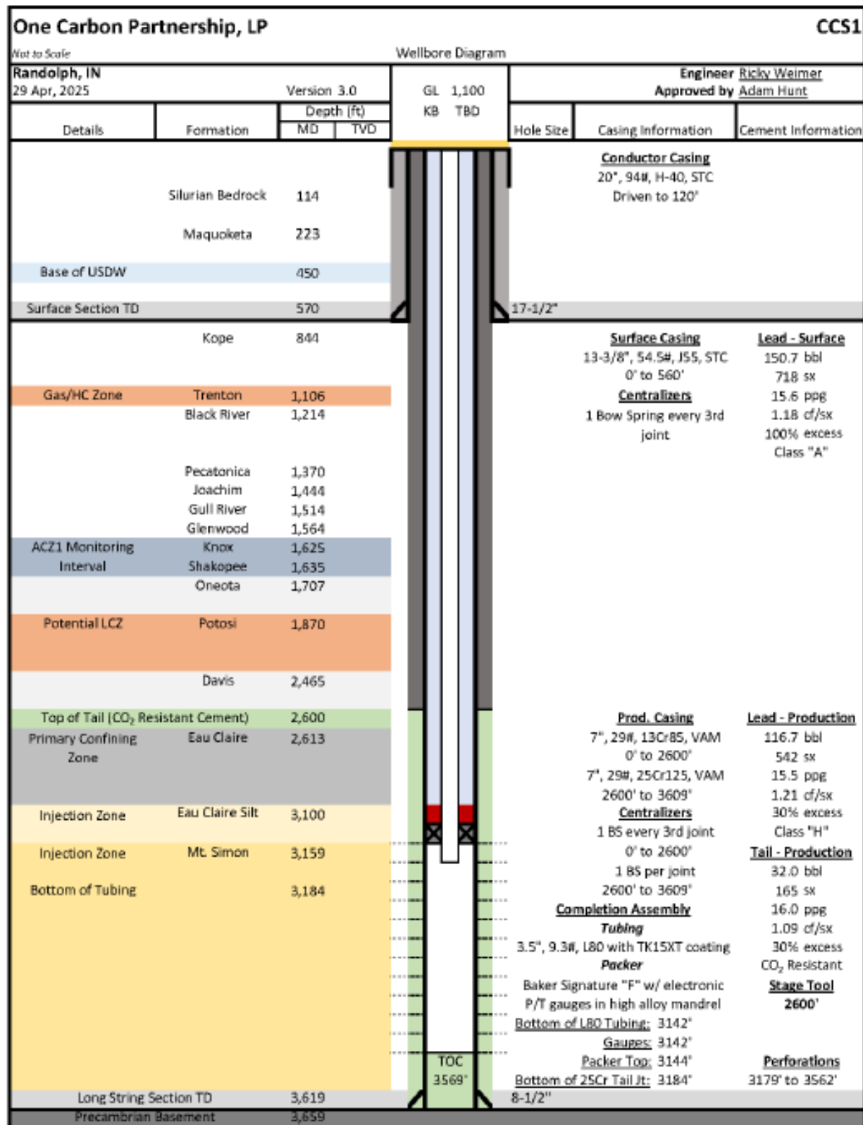
Figure 1: Injection Well Construction Diagram
