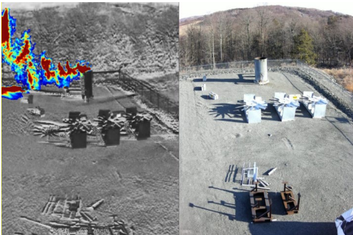
Figure 3: Infrared and visible images of a methane detection
