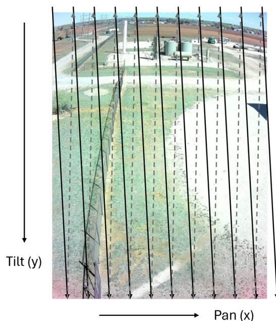
Figure 2: Raster scan pattern employed by the Kuva GCI360. Full field of view is 46° (H) x 54° (V)
