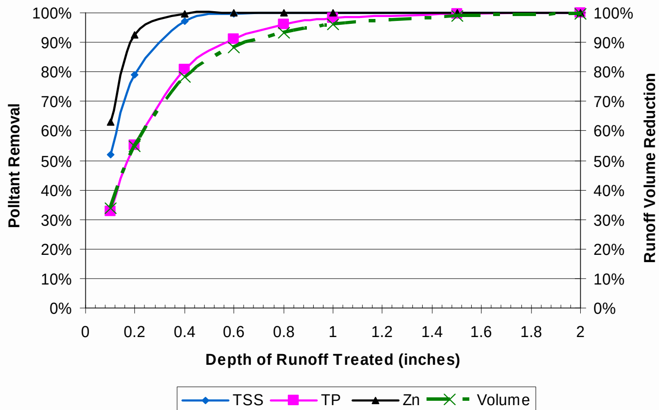
BMP Performance Curve: Infiltration Trench Land Use: High Density Residential (Soil infiltration rate 2.41 in/hr)
