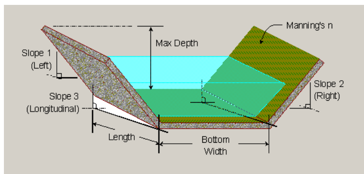
Figure 4-32. The BMPDSS transport module for grass swales.
