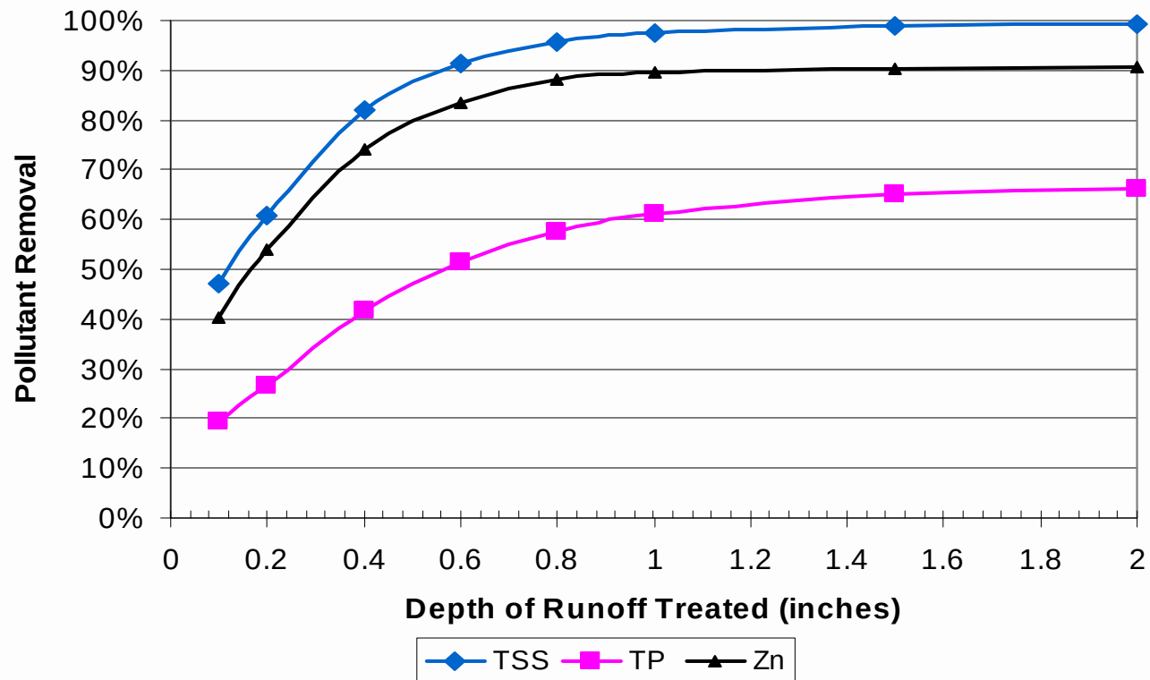
BMP Performance Curve: Gravel Wetland Land Use: Industrial
