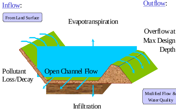
Figure A-3. Major processes included in Class B: Channelized BMPs.
