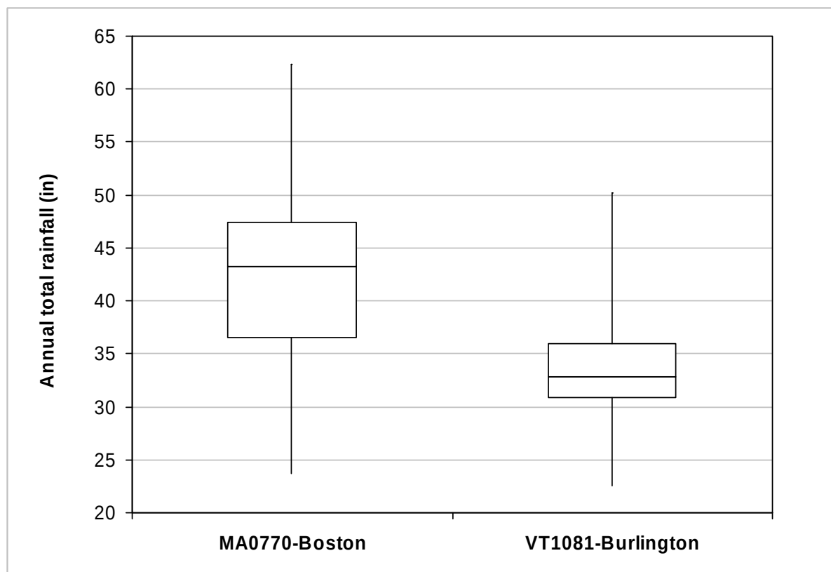
Figure 2-3. Recommended weather stations based on annual precipitation for evaluating BMP performances.
