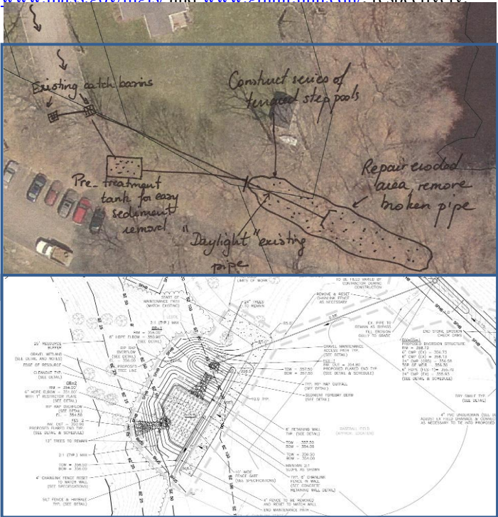
Figure 3. Concept sketches can be done by hand. Once priorities have been identified, concepts can be further advanced to engineering design and construction plans.
