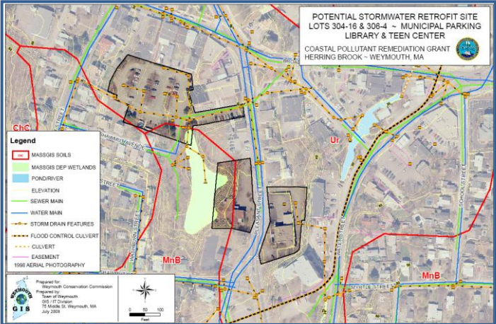
Figure 2. Mapping analysis used to identify potential locations for retrofits in Weymouth, MA showing aerial imagery, parcel ownership, stormwater infrastructure and utilities, topography, soils, and hydrology. The MassGIS and NH’s GRANIT websites are good sources of GIS data and can be found at www.mass.gov/mgis/ and www.granit.unh.edu/ respectively.
