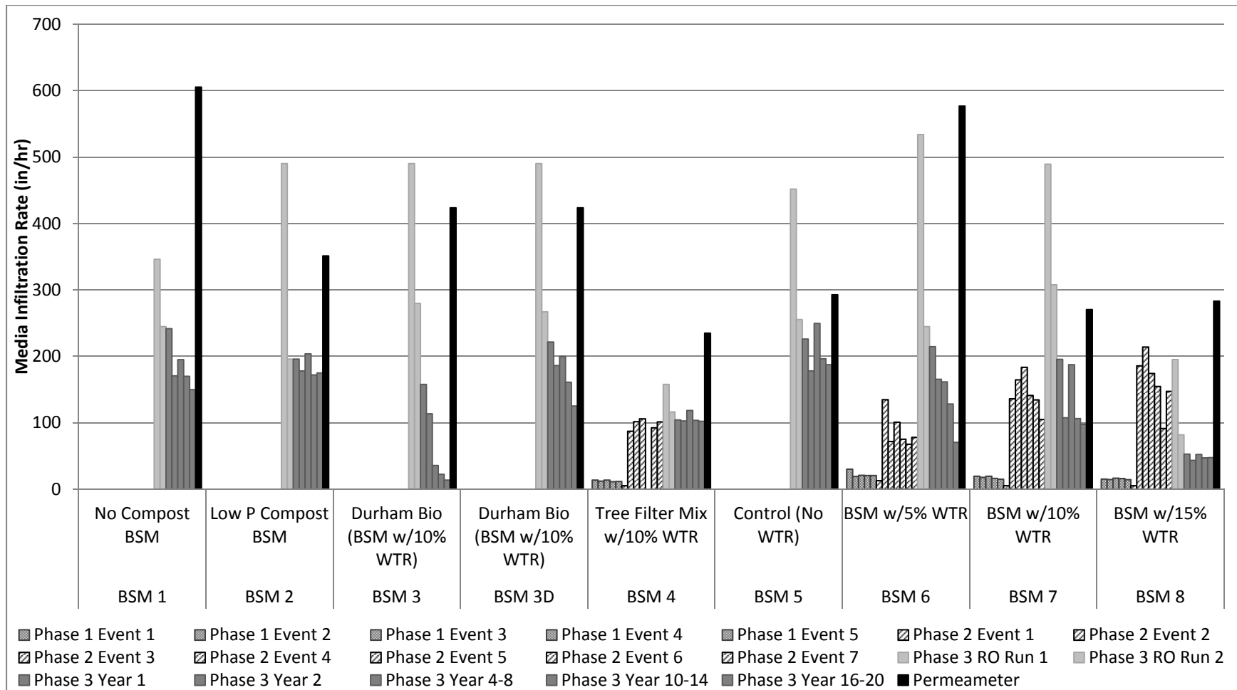
Figure 24. Infiltration Rates of filter media (BSMs) used in each column study phase and permeameter tests. RO runs indicate runs with clean water (ROwater) prior to the start of the experiment.
