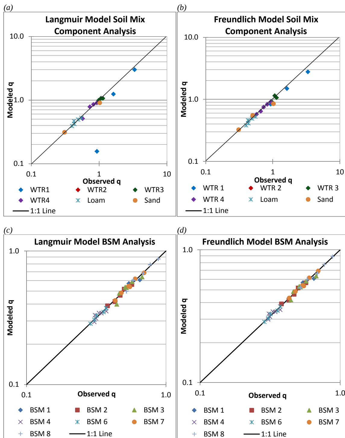
Figure 23. Isotherm Model Assessment: Linear Regression of Observed vs. Modeled q (mg/g).
