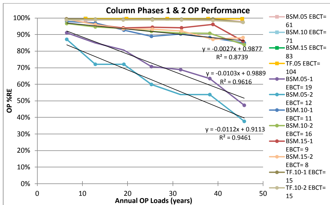
Figure 25. Phases 1 and 2 Column Removal Efficiencies based on annual nutrient loads of 43 mg OP/ft 2 . Square markers denote phase 1 columns; circle markers denote phase 2 columns.
