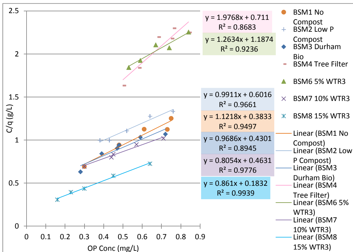
Figure 21. Langmuir Isotherm Model for BSMs
