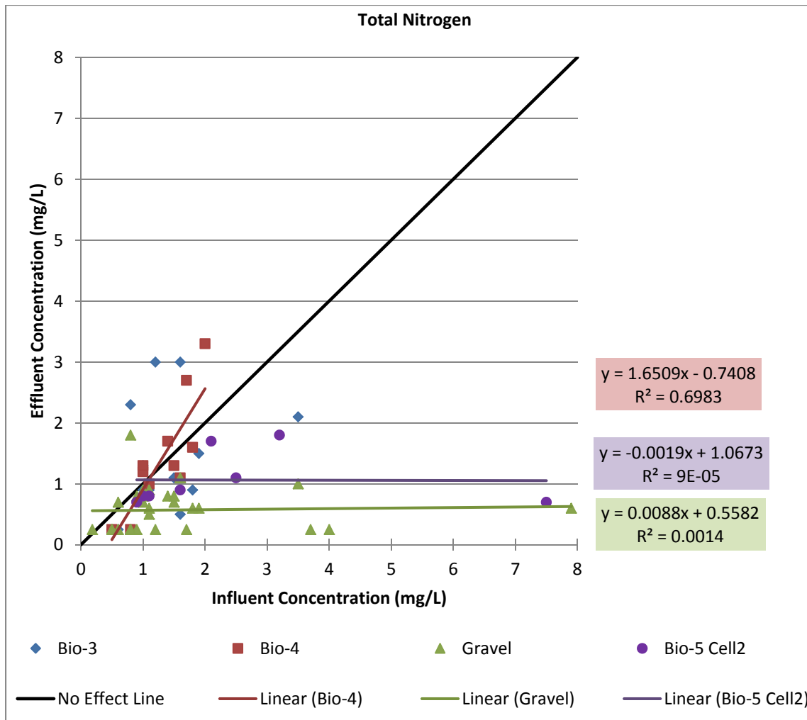
Figure 38. Treatment Effect Plot on TN for 4 UNH systems.
