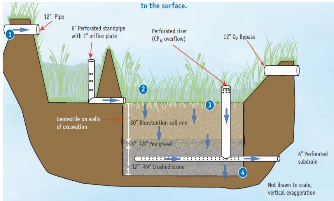
Figure 1. Bioretention Schematic
