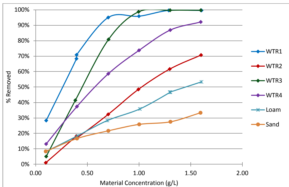
Figure 17. Adsorption Isotherm Data for BSM Constituents.
