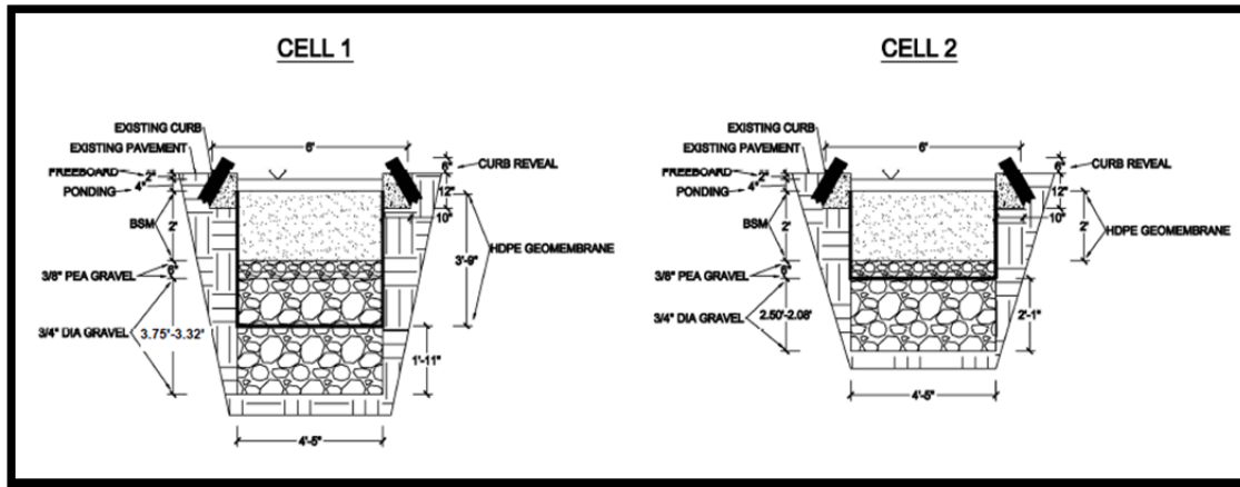
Figure 13. Cross-Section of Durham Bio-5 Bioretention Cells.
