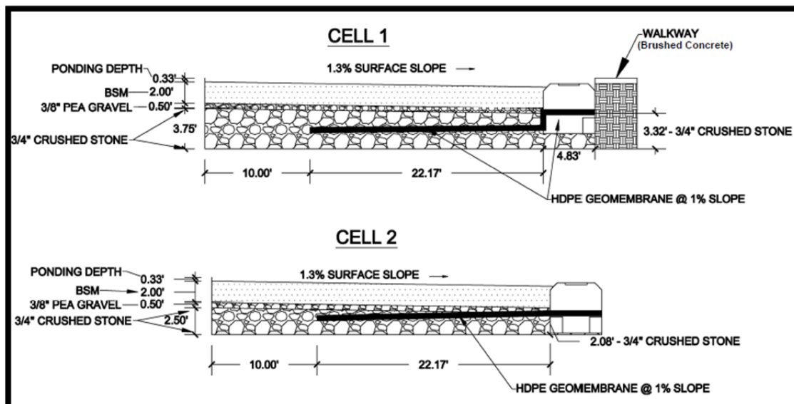
Figure 12. Long Section of Durham Bio-5 Bioretention Cells.
