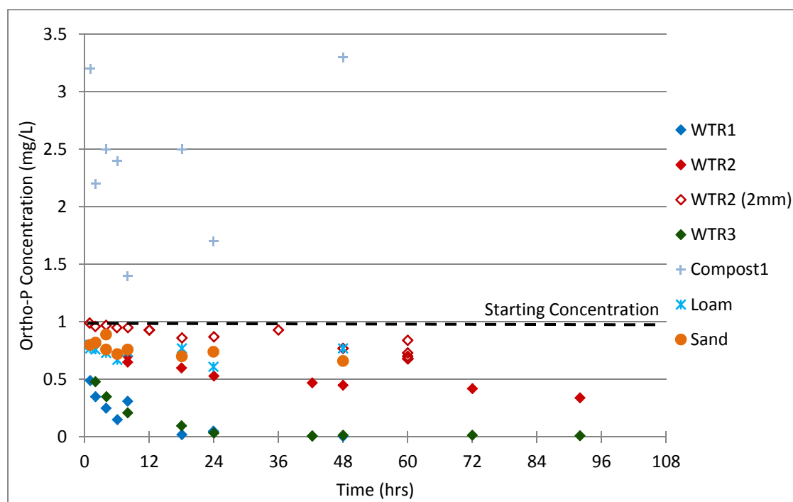
Figure 16. Kinetics Study Results.
