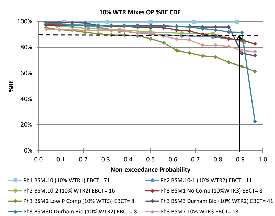
Figure 27. Column Performance for OP Removal from all columns with 10% WTR from phases 1-3. Phase 1 mix (BSM.10) has box markers. Phase 2 mixes have circular markers. Phase 3 mixes have diamond markers. Empty Bed Contact Time is given for each mix in minutes.
