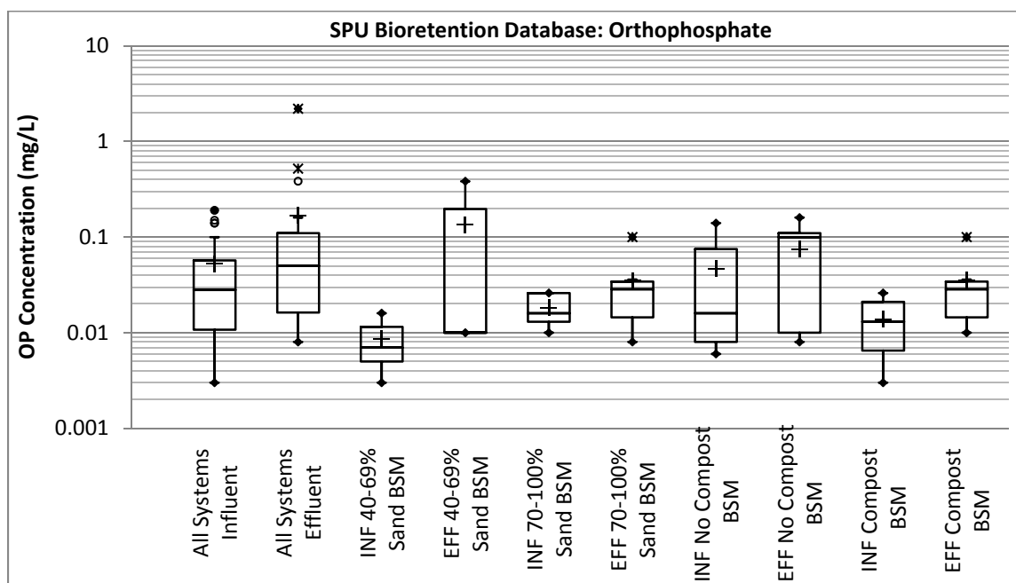
Figure 5. Box-and-Whisker Plots for Orthophosphate from the SPU Bioretention Database.
