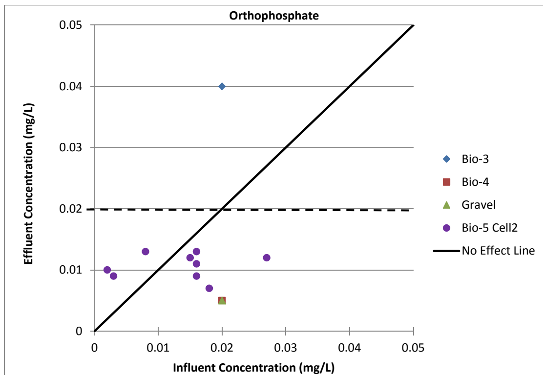
Figure 36. Treatment Effect Plot on OP for 4 UNH systems.
