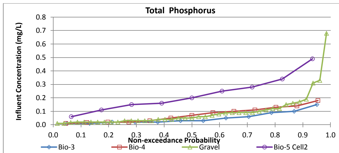
Figure 34. Influent Concentration distribution for 4 vegetated systems monitored by UNHSC.
