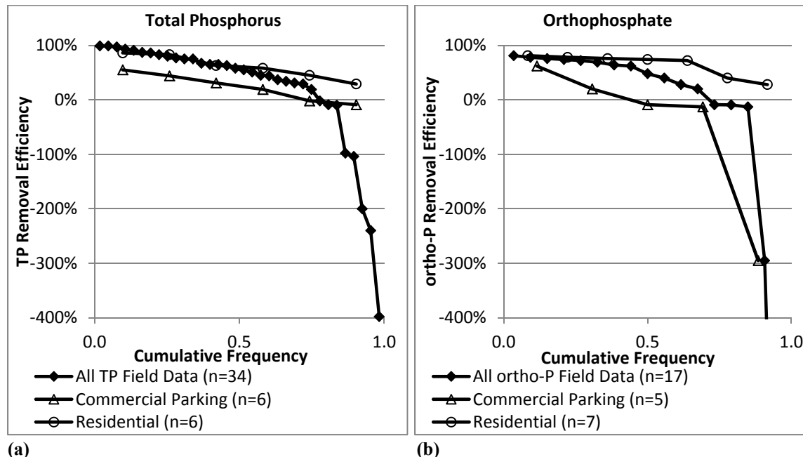
(a) (b) Figure 6. Cumulative Frequency Functions of Total Phosphorus and Orthophosphate Removal Efficiencies in the SPU Bioretention Database.
