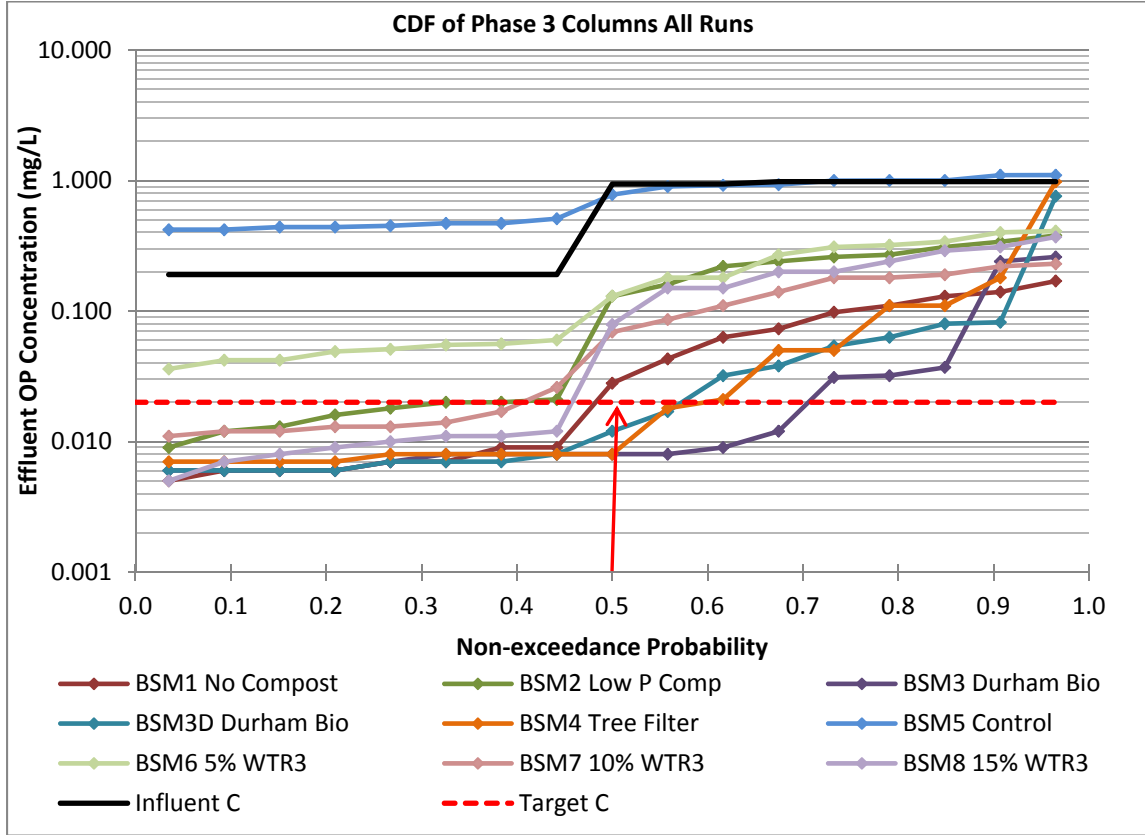
Figure 28. Cumulative Distribution of orthophosphate concentrations in phase 3 column study.
