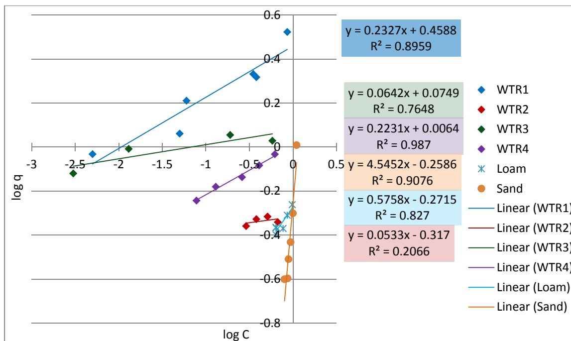
Figure 20. Freundlich Isotherm Model for Constituents
