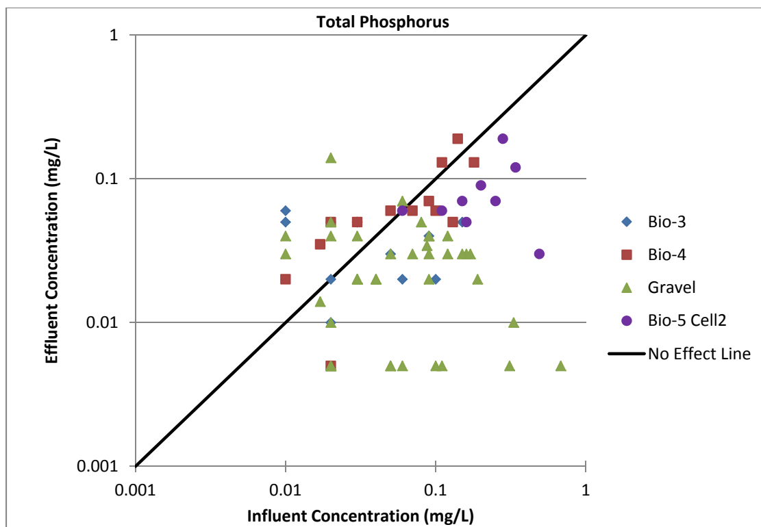
Figure 37. Treatment Effect Plot on TP for 4 UNH systems.
