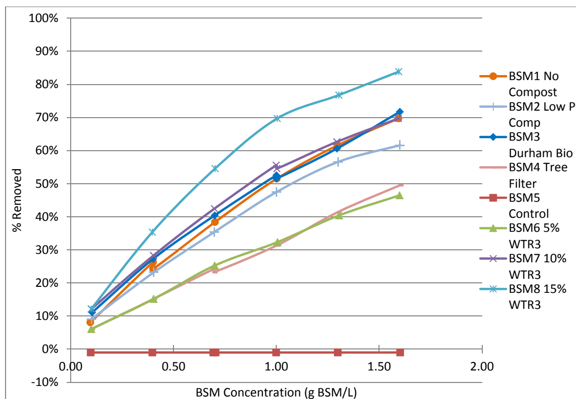
Figure 18. Adsorption Isotherm Data for BSMs
