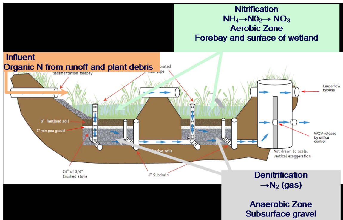
Figure 2. Gravel Wetland Schematic
