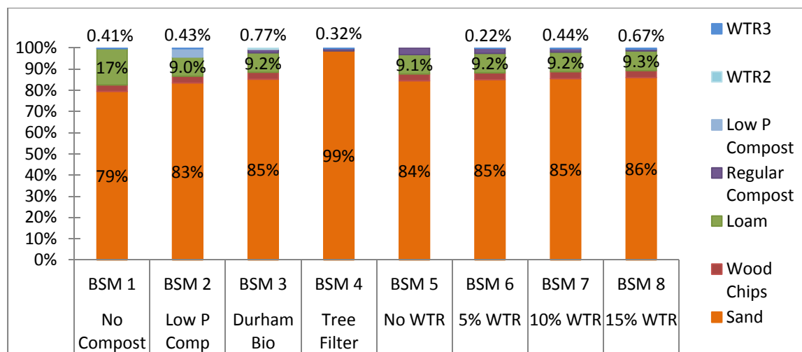
Figure 15. BSM Composition on a dry mass basis Numbers above the columns represent the % WTR content in the BSM on a dry mass basis.
