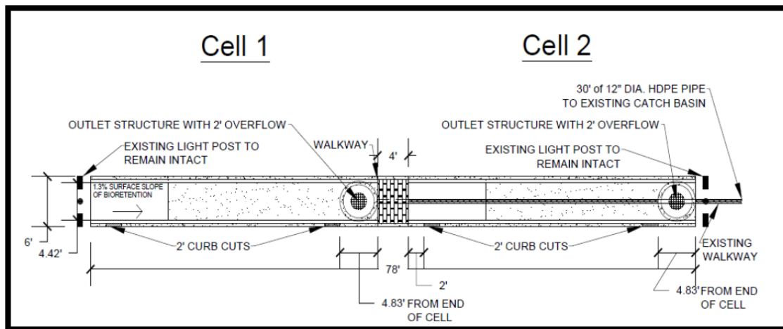
Figure 11. Layout of Durham Bio-5 Bioretention Cells.
