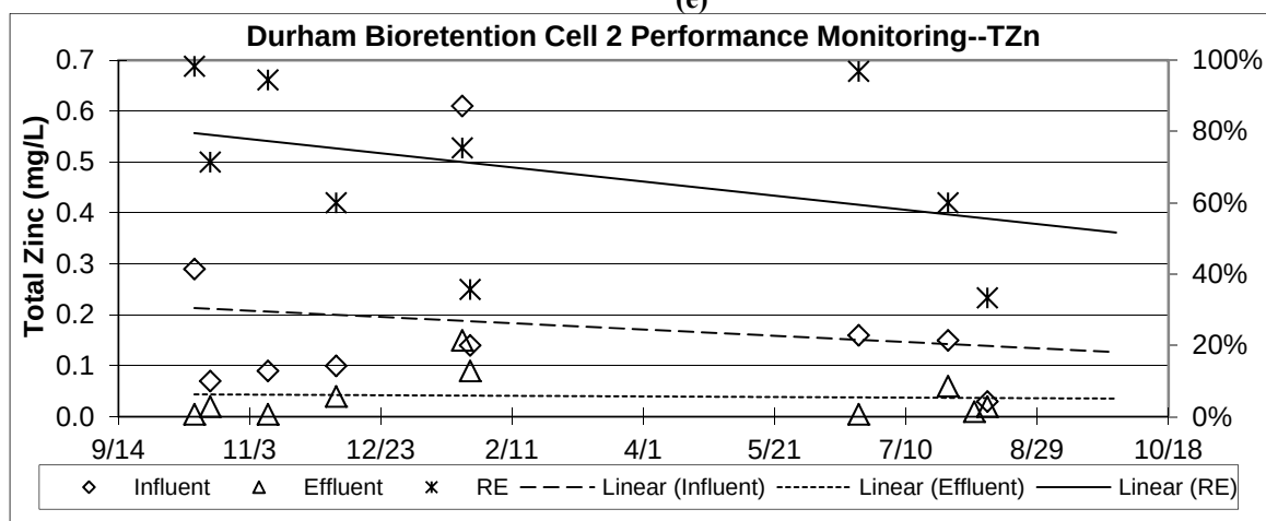
Figure 30. Time Series Water Quality Data from Bio-5 Cell 2 for contaminants (a) Total Suspended Sediments, (b) Total Nitrogen, (c) Nitrate, (d) Total Phosphorus, (e) Orthophosphate, and (f) Total Zinc.
