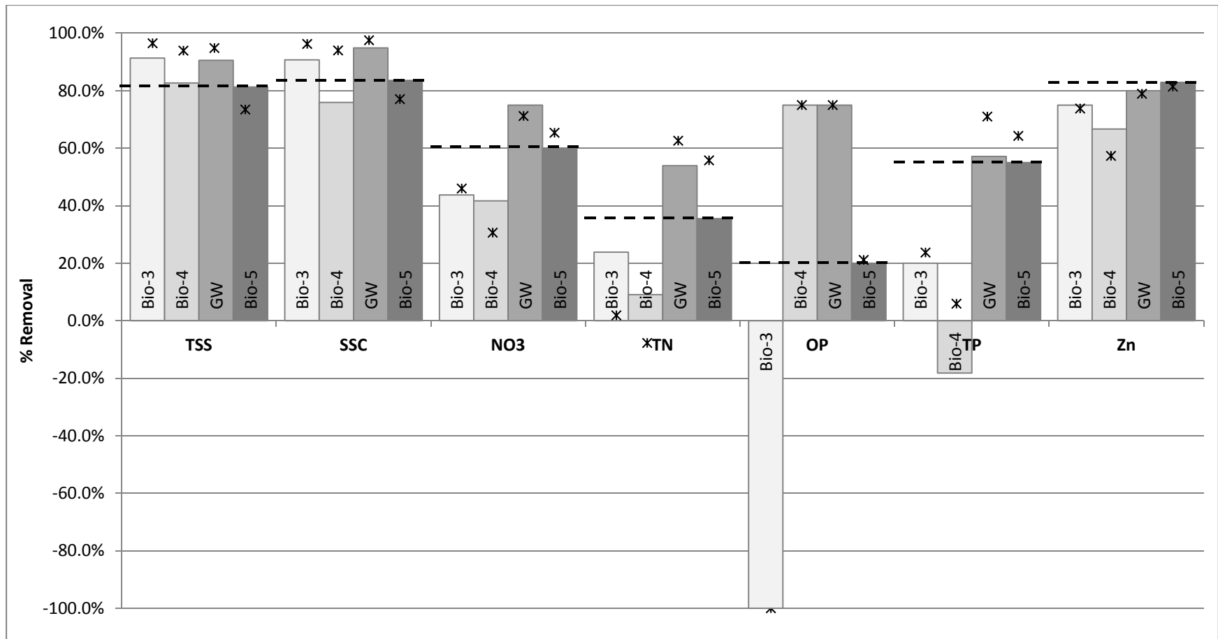
Figure 33. Contaminant Removals by 4 UNHSC vegetated stormwater treatment systems. Columns indicate the median %RE, while *'s represent efficiency ratios.
