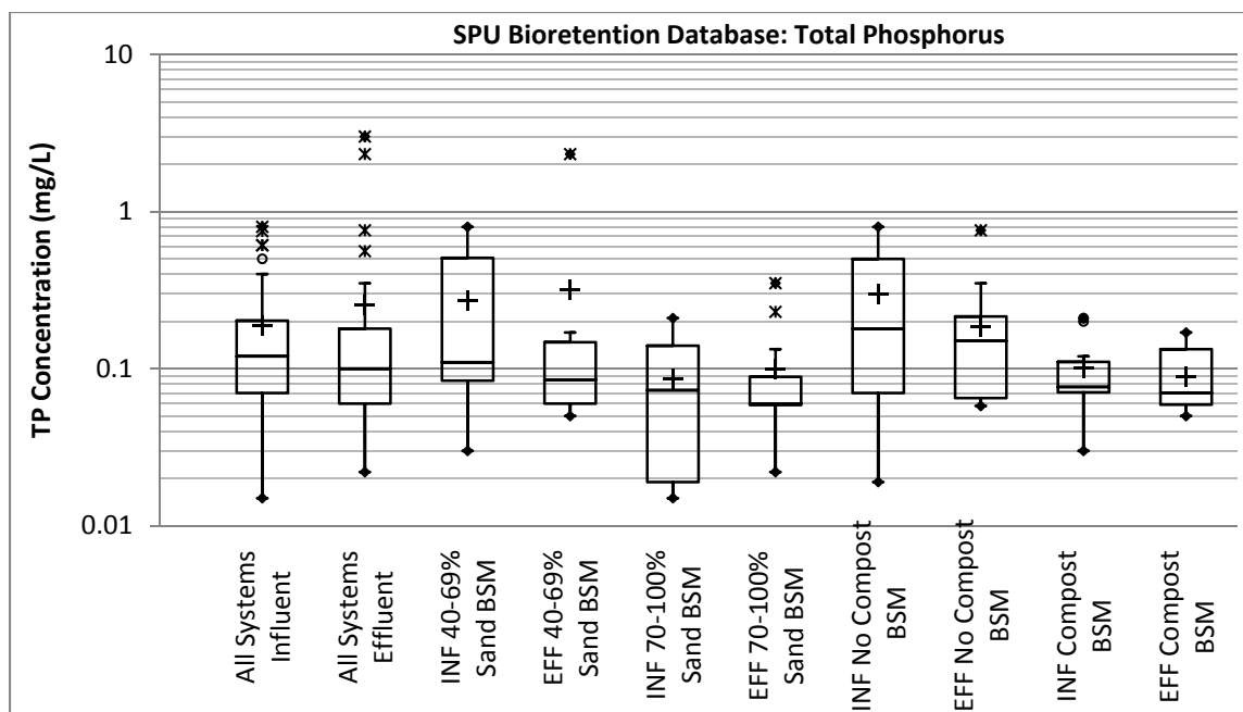
Figure 4. Box-and-Whisker Plots for Total Phosphorus from the SPU Bioretention Database.
