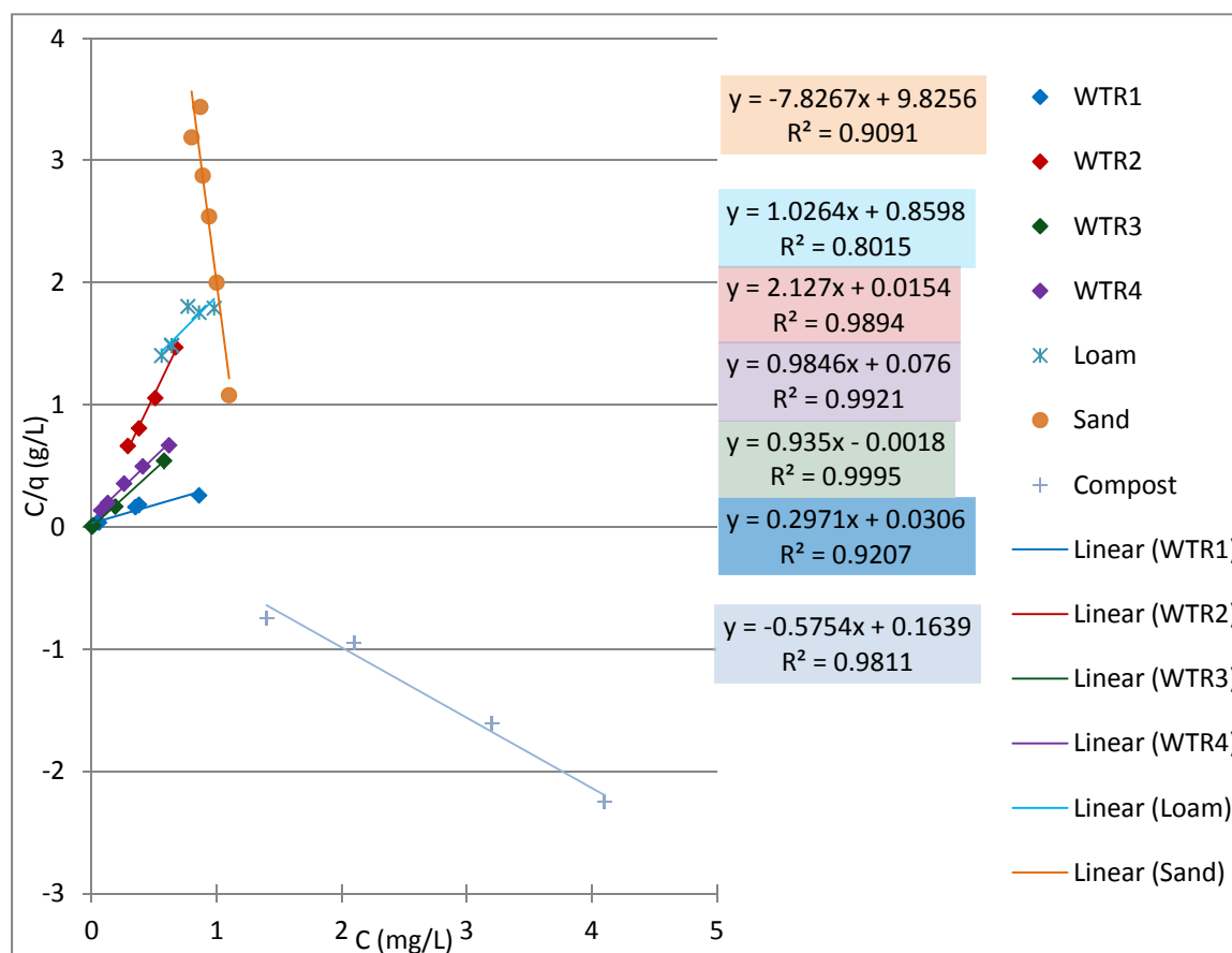
Figure 19. Langmuir Isotherm Model for Constituents
