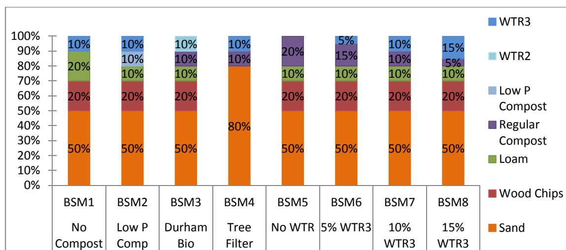
Figure 14. BSM Composition on a volume basis
