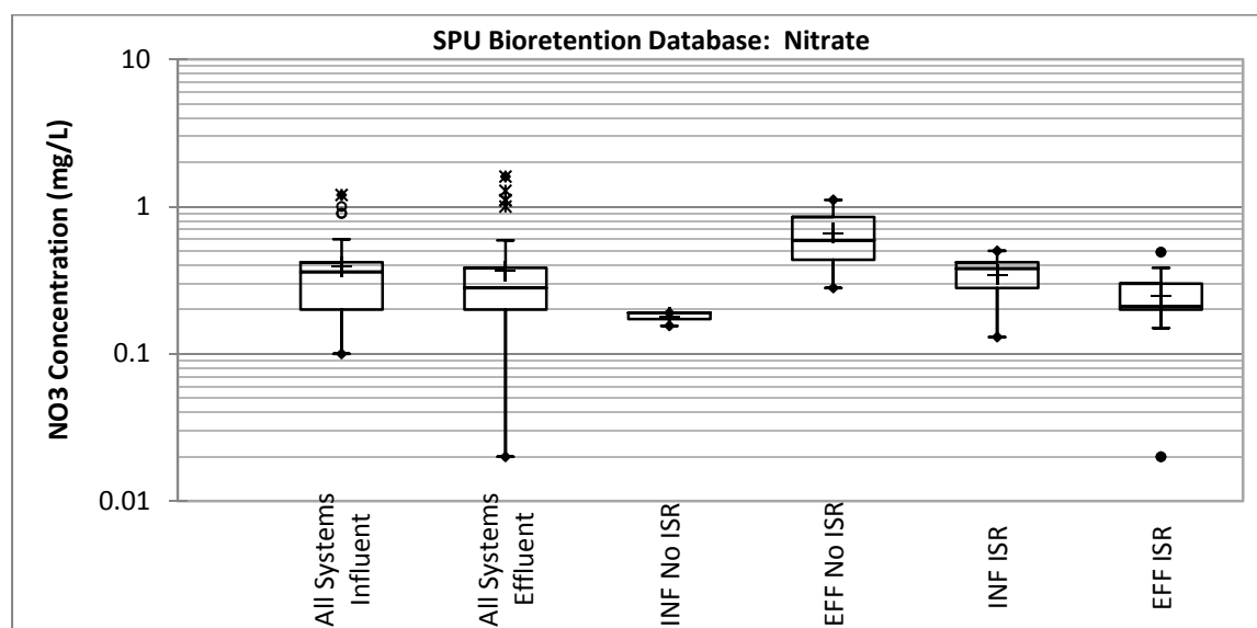
Figure 8. Box-and-Whisker Plots for Nitrate from the Bioretention Database.
