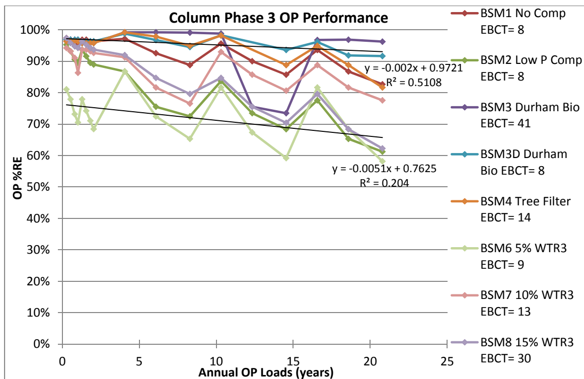
Figure 26. Phase 3 Column Removal Efficiencies based on annual nutrient loads of 43 mg OP/ft 2 .
