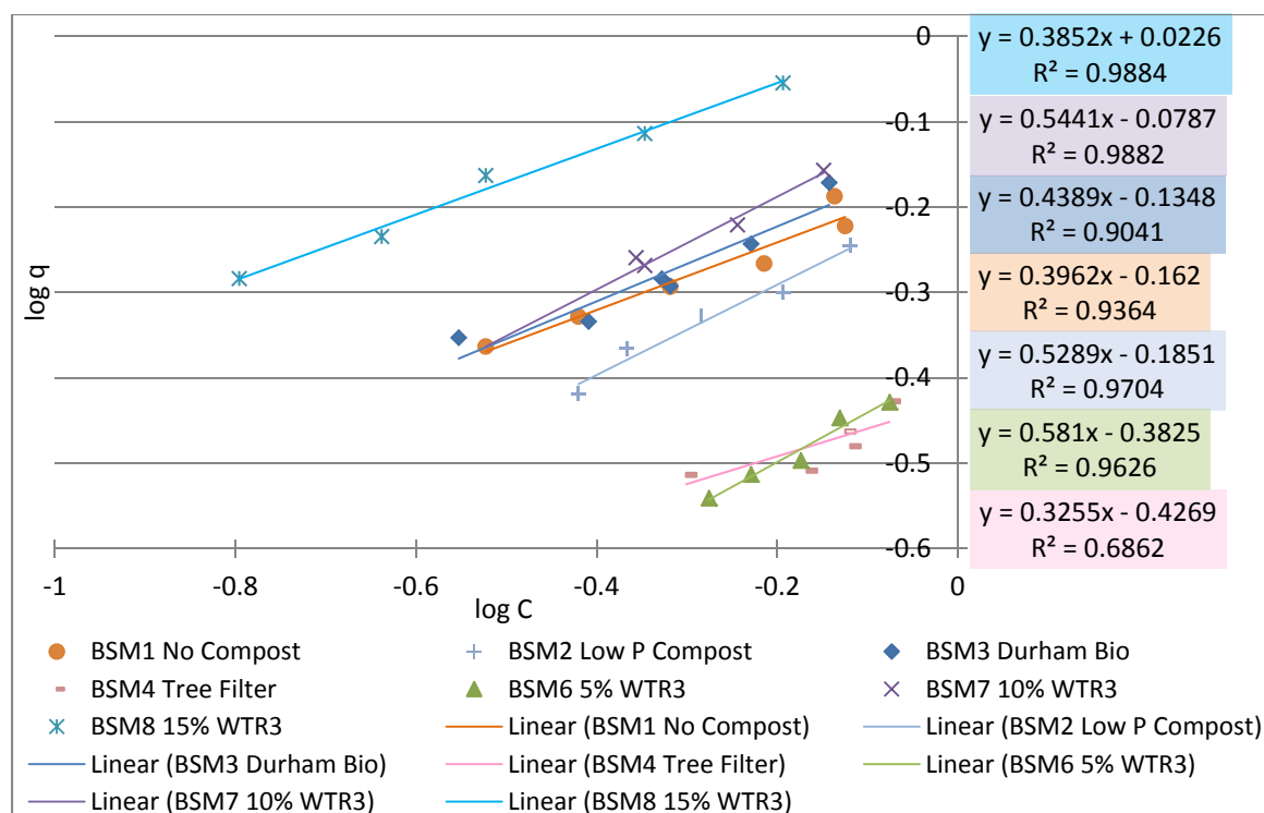
Figure 22. Freundlich Isotherm Model for BSMs
