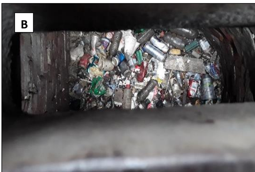
Open-curb inlets (A) can become collection systems for floatables and (B) other potential harmful pollutants during high flow events. Credit: T. Maguire
