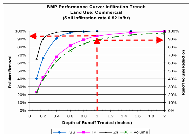
BMP optimization curve displaying estimated pollutant and runoff volume reduction for various depths of runoff treatment. (Source: Tetra Tech for EPA: Stormwater Best Management Practices (BMP) Performance Analysis)
