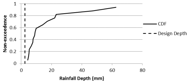
Figure 6 Oyster River Road SGWSC cumulative distribution frequency plot with rainfall design depth of 2.5 mm (0.1 in.) for reference.
